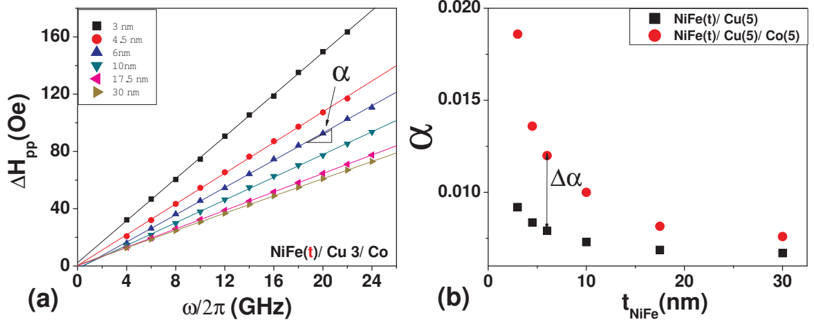
Figure 4.10: (a) Frequency-dependent peak-to-peak FMR linewidth \Delta H_{pp}(\omega) for FM = Ni_{81}Fe_{19} , t_{FM} as noted, films with Co(5nm) overlayers. (b) red dots represents \alpha_{FM2}(t_{F1}) (with the FM2 = Co overlayer) and black squares represents \alpha_{noFM2}(t_{F1}) (without the FM2 = Co overlayer) as extracted from the slope of \Delta H_{pp} vs. \omega plot.
