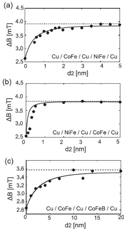
Figure 5.4: The FM_2 thickness dependence of the line width of the FMR power absorption spectra for FM_1/\text{Cu}/FM_2 structure, as observed by Taniguchi et al. [34]. Materials of the FM_2 layer are (a) Ni_{80}Fe_{20} , (b) Co_{75}Fe_{25} and (c) Co_{40}Fe_{40}B_{20} , respectively.
