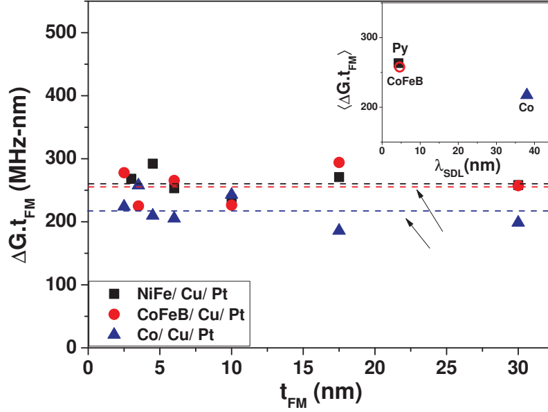
Figure 4.7: The additional nonlocal relaxation due to Pt overlayers, expressed as a Gilbert relaxation rate - thickness product \Delta G \cdot t_{FM} for Py, CoFeB, and Co. Inset : dependence of \Delta G \cdot t_{FM} on spin diffusion length \lambda_{SD} as tabulated in ref. [42].
