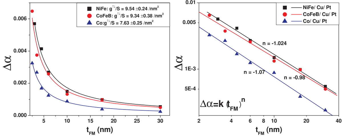
Figure 4.6: Contributed Gilbert damping \Delta\alpha(t_{FM}) = \alpha_{Pt}(t_{FM}) - \alpha_{noPt}(t_{FM}) for FM ( =Py, CoFeB, and Co ), plotted (a) in a linear scale, (b) in a log-log scale. The slopes express the power law exponent n = -1.03 \pm 0.04 .
