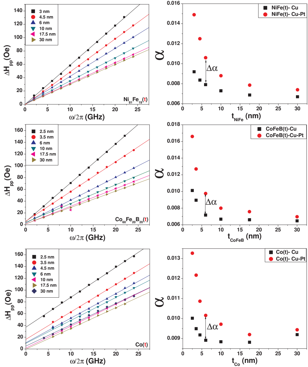
Figure 4.5: The one's in the left side represents \Delta H_{pp}(\omega) as a function of \omega for NiFe, CoFeB and Co heterostructures with the Pt overlayer. The one's in the right side are the contributed Gilbert damping \Delta\alpha(t_F) = \alpha_{Pt}(t_F) - \alpha_{noPt}(t_F) for NiFe, CoFeB and Co
