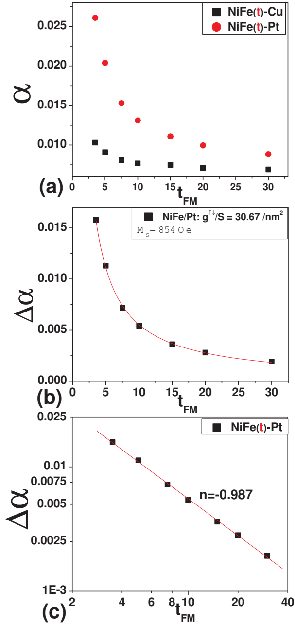
Figure 4.9: Damping parameter for Pt in direct contact with Py. (a) red dots represents \alpha(t_{Py}) for Py/Pt structure and black squares represents \alpha(t_{Py}) without the Pt overlayer. (b) Additional damping \Delta\alpha(t_{Py}) is plotted as a function of t_{Py} (b) in linear scale, (c) in Log-log scale.
