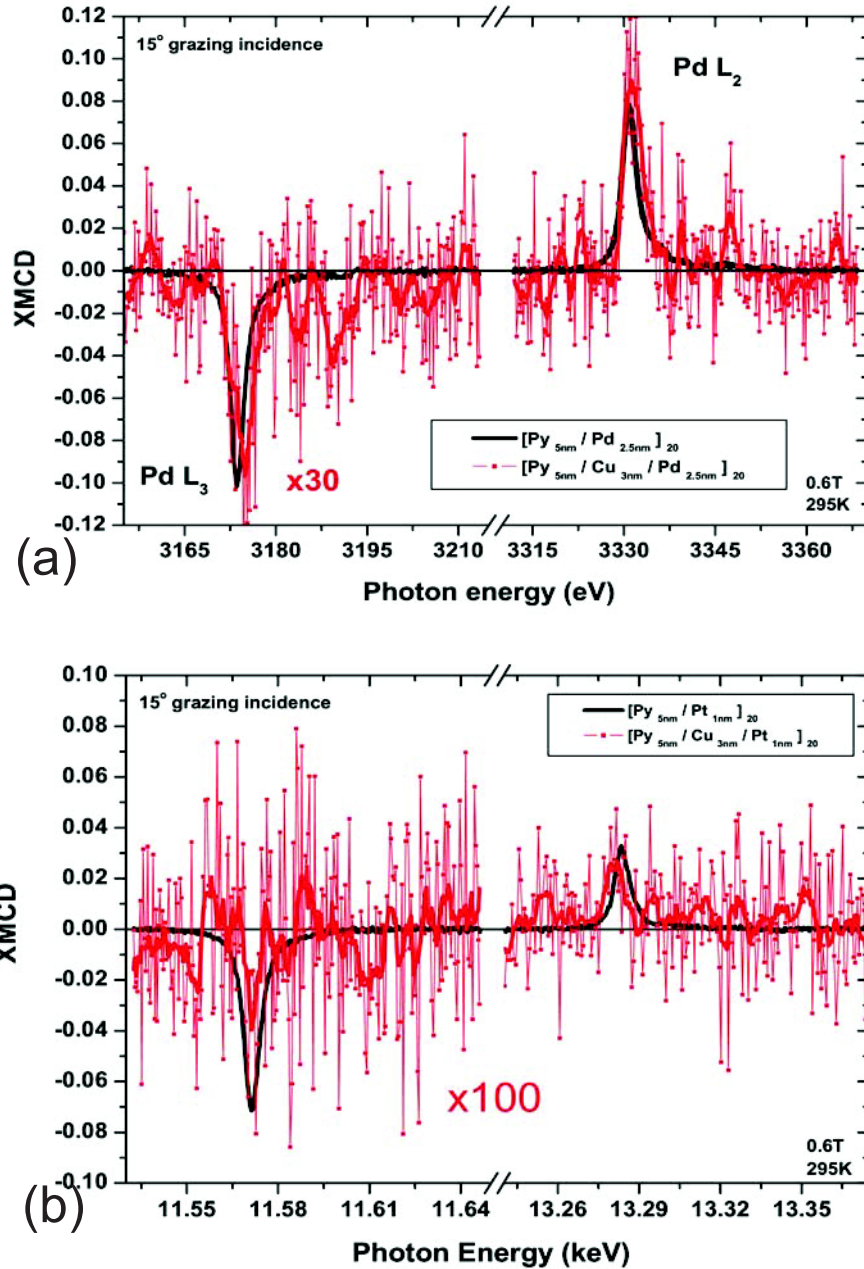
Figure 6.2: XMCD spectra for (a) direct exchange-coupled [Py(5nm)/Pd(2.5nm)]_{20} and indirect exchange-coupled [Py(5nm)/Cu(3nm)/Pd(2.5nm)/Cu(3nm)]_{20} samples (magnified by a factor of 30). (b) direct exchange-coupled [Py(5nm)/Pt(1nm)]_{20} and indirect exchange-coupled [Py(5nm)/Cu(3nm)/Pt(1nm)/Cu(3nm)]_{20} samples (magnified by a factor of 100).
