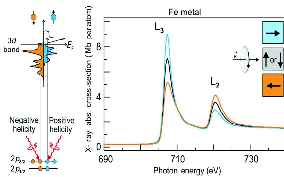
Figure 3.6: Schematic of X-ray magnetic circular dichroism (XMCD) effect for L -edge, with LCP and RCP X-rays. This figure was taken from ref. [52].
