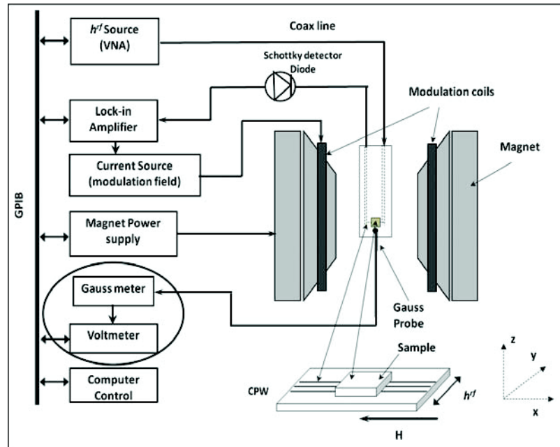
Figure 3.3: Schematic diagram of the FMR spectrometer. Microwave radiation is transmitted through a CPW, located between the pole pieces of the electromagnet. Transmitted power is converted into voltage using a Schottky diode and used as the Lock-in Amplifier input.
