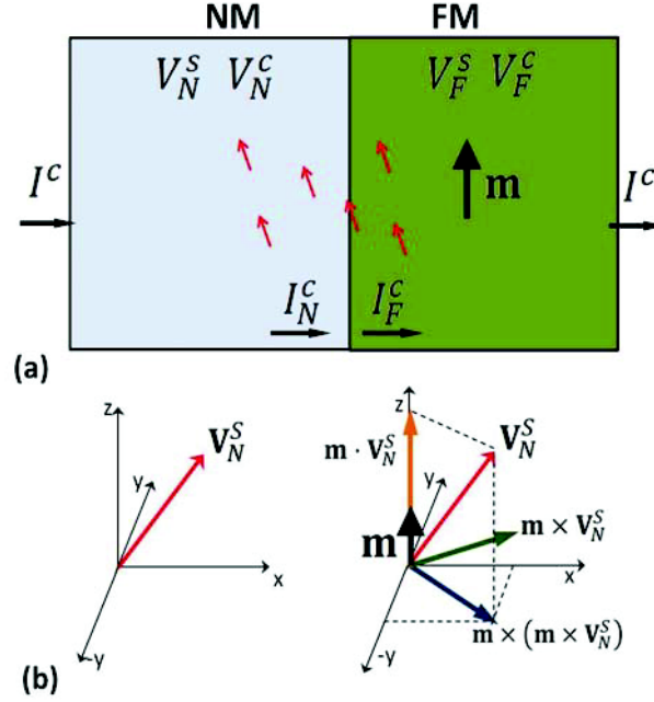
Figure 2.3: Schematic illustration of the spin transfer torque in layered NM/FM structure. Spin accumulation \mathbf{V}_N^S in the NM induces a spin-transfer torque \tau_{STT}^{bias} on FM.
