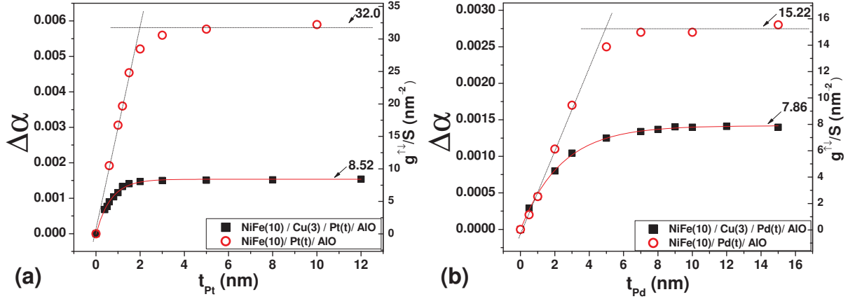
Figure 5.7: \Delta\alpha for 10 nm of NiFe as a function of t_{PM} for (a) Pt , (b) Pd . Red circled represents the data for structures where Pt or Pd are in direct contact to NiFe , and black squares represents where 3 nm of Cu spacer separates NiFe from Pt or Pd .
