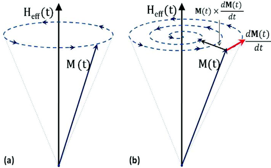
Figure 1.3: (a) Uniform precession of magnetization without any damping in the system. (b) Damping acts \perp to the direction of motion of the magnetization \mathbf{M} , and makes it relax along the effective field \mathbf{H}_{eff} .
