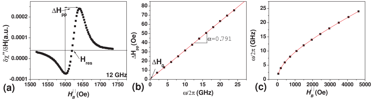
Figure 3.5: (a) Sample Lineshape obtained by our FMR spectrometer. (b) peak-to-peak linewidth \Delta H_{pp} obtained at different microwave frequencies are plotted. Damping parameter \alpha obtained from the slope of the plot. (c) Resonance fields H_{res} are plotted as a function of applied microwave frequency \omega (Kittel plot).
