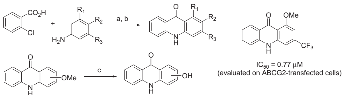
Scheme 2. Synthesis of acridones (azaxanthenes). (a) Cu, K_2CO_3 , (b) H_3PO_4 , (c) AlCl_3 for demethylation of OMe at C-1), BBr_3 (for demethylation of OMe at other positions) [105].
