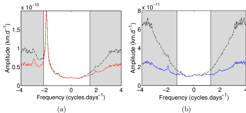
FIGURE 3.4 – Illustration of the effect of the buoy position uncertainty on the transfer function using datasets (a) number 8 and (b) number 1. The red and blue bold curves are the transfer functions computed from the raw buoy positions. The black dashed curves are associated transfer functions computed using the respective dataset, but after adding noise to the buoy positions (300 m standard deviation). We outline in gray the frequencies affected by the uncertainty on the buoy positions.
