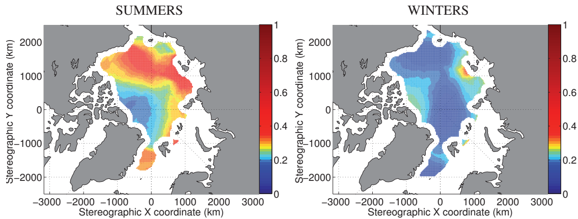
FIGURE 2.9 – Spatial pattern of inertial oscillation magnitude within the Arctic Basin in summer (left) and in winter (right). These two fields are computed from the seasonal M dataset. A spatially averaged value of M values, denoted \overline{M} , is computed following Eq. (2.10) for each point of a 25 km resolution grid. The graphic representation is a linear interpolation of the gridded \overline{M} values. In order to not represent regions with little data, an \overline{M} value at a given grid point is plotted only if its associated weight is greater than a minimum value we arbitrarily set to 1000.
