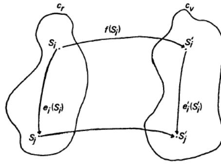
Figure 2.2: The Virtual Machine Map (source : [6])
