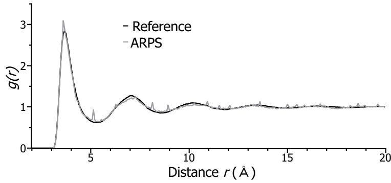
Figure 4.5.10: Radial distribution functions of an Argon system obtained with full-dynamics and AR simulations (periodic 3D box, 343 particles, NVT ensemble). After 50 000 simulation steps RDF in the AR simulation is noisier than the reference one.
