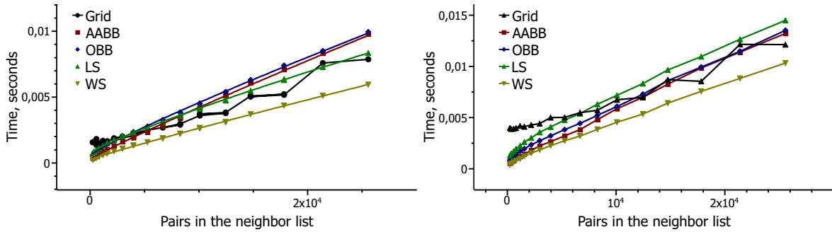
Figure 2.3.12: Cutoff test. Computational performances of all algorithms as functions of the number of pairs in contact for the system of two apoferritin molecules. Results obtained on Computer 1 (left) and on Computer 2 (right). Solid lines represent fitting curves, except for those for the grid algorithm.
