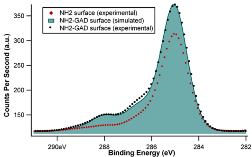
Figure 3.29: Comparison between experimental and simulated spectra for \text{NH}_2 -GAD surfaces.
