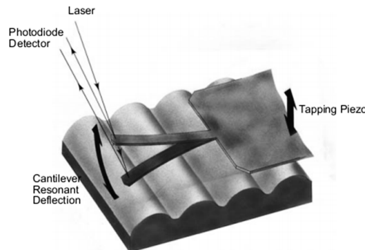
Figure 2.11: The AFM was used in tapping mode, in this mode the cantilever is not steadily in contact with the surface sample, but is oscillating [124,125].
