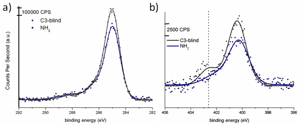
Figure 3.36: The profile of C1s (a) and N1s (b) high resolution spectra changed after immersion in solution of C3. (a) shows the same profile, hence the interpretation of a new surface modification is difficult. (b) shows the N1s spectra with a new component at 402.5 eV that appeared, which indicates that a surface modification took place.
