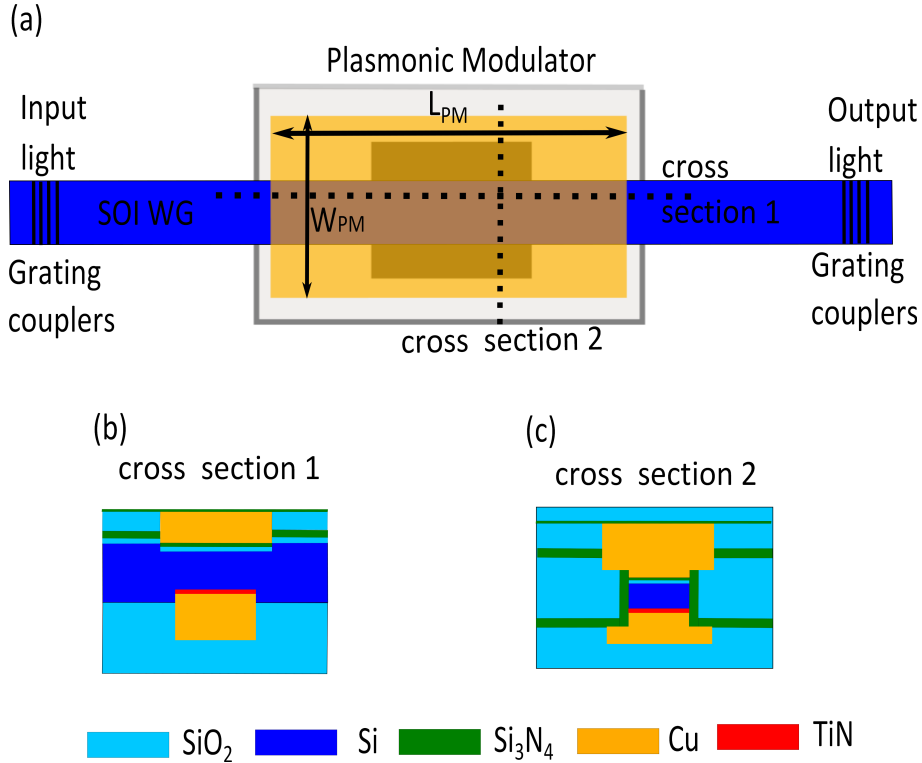
FIGURE 3.12 – Schematic top view of the integrated plasmonic modulator (a) with different cross accordingly to different planes; cross section in the direction of propagation (b) cross section in perpendicular direction (c).
