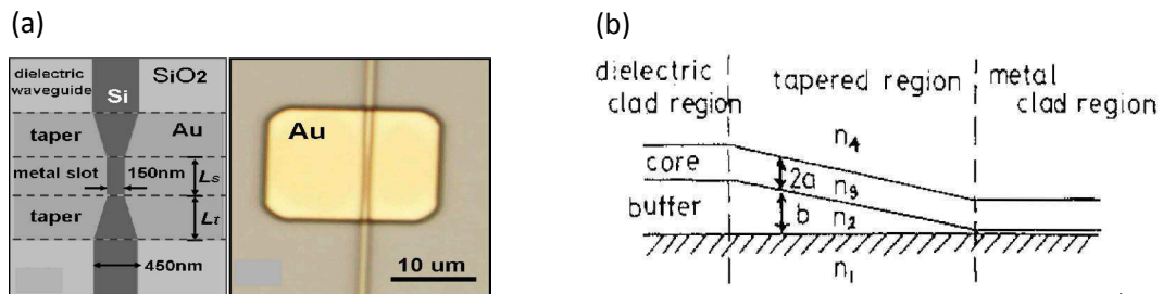
FIGURE 4.4 – (a) Lateral taper [12]; (b) vertical taper [13] connecting dielectric WG with metal WG.
