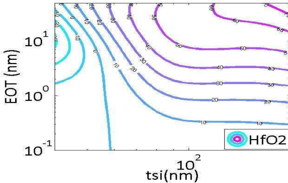
FIGURE 8.1 – Percentage gain in propagation length (%) compared to the SiO 2 as a function of EOT and Si thickness when Al 2 O 3 or HfO 2 are used.
