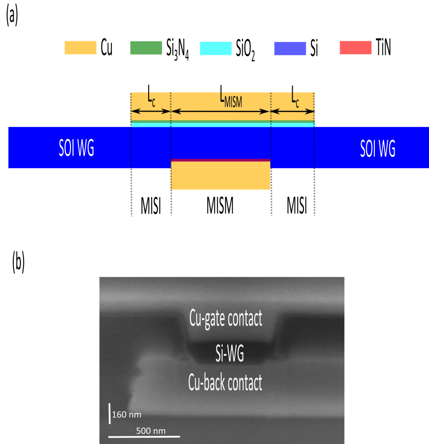
FIGURE 4.5 – (a) Hybrid plasmonic waveguide showing the coupling structure (MISI) connecting the SOI-waveguide and MISM; (b) SEM image of the cross section of the MISM structure
