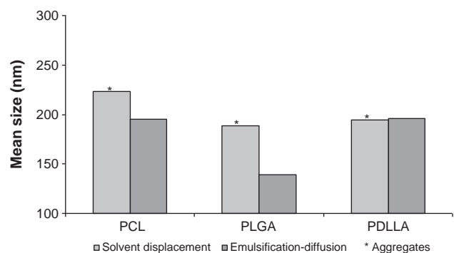
Fig. 9. Influence of polymer nature on size of submicron spheres prepared by solvent displacement and emulsification-diffusion methods (polymer and the stabilizing agent concentrations: 10 mg/ml and 1% respectively).
