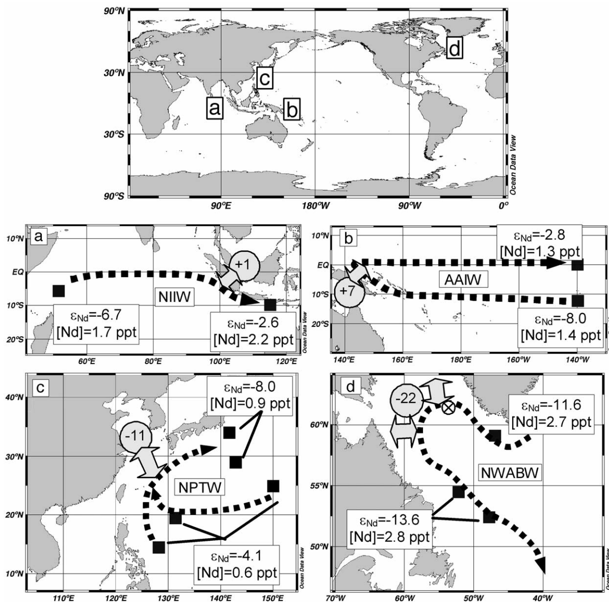
Fig. 2. Variations of the Nd isotopic composition and concentration within a water mass due to continent/ocean interactions. 1 ppt (part per trillion) = 10^{-12} g g ^{-1} . Left panel shows the location of the other panels. (a) NIIW, (b) AAIW, (c) NPTW and (d) NWABW (acronyms defined in Table 1). The sample locations are shown by the black squares, water mass pathways are schematized by the dotted arrows and the Nd isotopic composition of the interacting sediments are shown on gray circles [16,20,21,41]. The double arrows schematize boundary exchange. In panel (d) the cross indicates the location of the station used to quantify the mixing and evidence the occurrence of external inputs.
