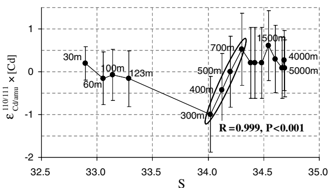
Fig. 10. Cd isotopic composition ( \epsilon_{\text{Cd/amu}}^{110/111} ) times Cd concentration (nmol/L) versus salinity. The ellipse shows the linear relationship found between 300 and 700 m depth. The corresponding regression coefficient ( R ) and significance level ( P ) are indicated, as are some sampling depths. Errors bars are calculated by propagating the 0.8 \epsilon_{\text{Cd/amu}} unit uncertainty characterizing the Cd isotopic composition data (the 2% uncertainty of the concentration data are ignored).
