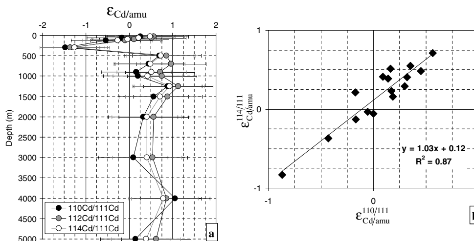
Fig. 7. Comparison of the isotopic compositions derived from different Cd isotope ratios at station K1 (N.W. Pacific). All isotopes were measured simultaneously. Error bars represent the mean discrepancy between replicates (0.8 \epsilon_{\text{Cd/amu}} unit). Note that the data from station DYFAMED (not shown for clarity purpose) do not show such inter isotope consistencies (because of unsatisfactory Sn interference corrections).
