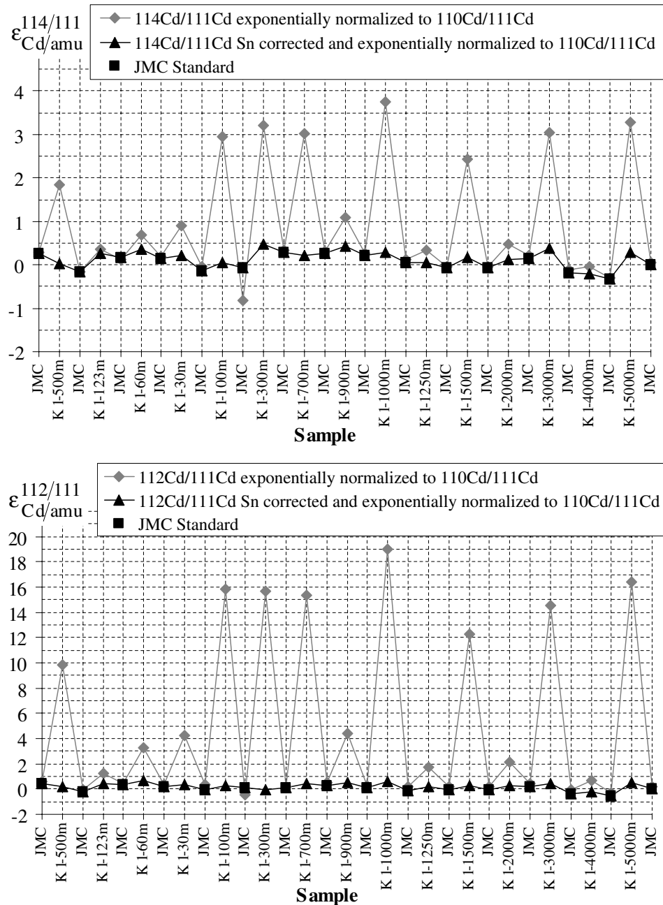
Fig. 3. Tin interference corrected and uncorrected data during one measurement session. The \varepsilon_{\text{Cd/amu}} values are calculated relative to the mean JMC standard Cd ratios.
