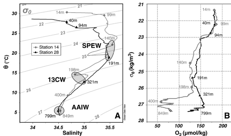
Fig. 2. A) Potential temperature ( \theta ) – salinity diagram. Potential density ( \sigma_\theta ) is shown (in \text{kg m}^{-3} ). B) dissolved oxygen concentration profiles for station 14 (in grey) and station 28 (in black). The samples presented in this study are indicated by symbols and their depths are reported (in meters).
