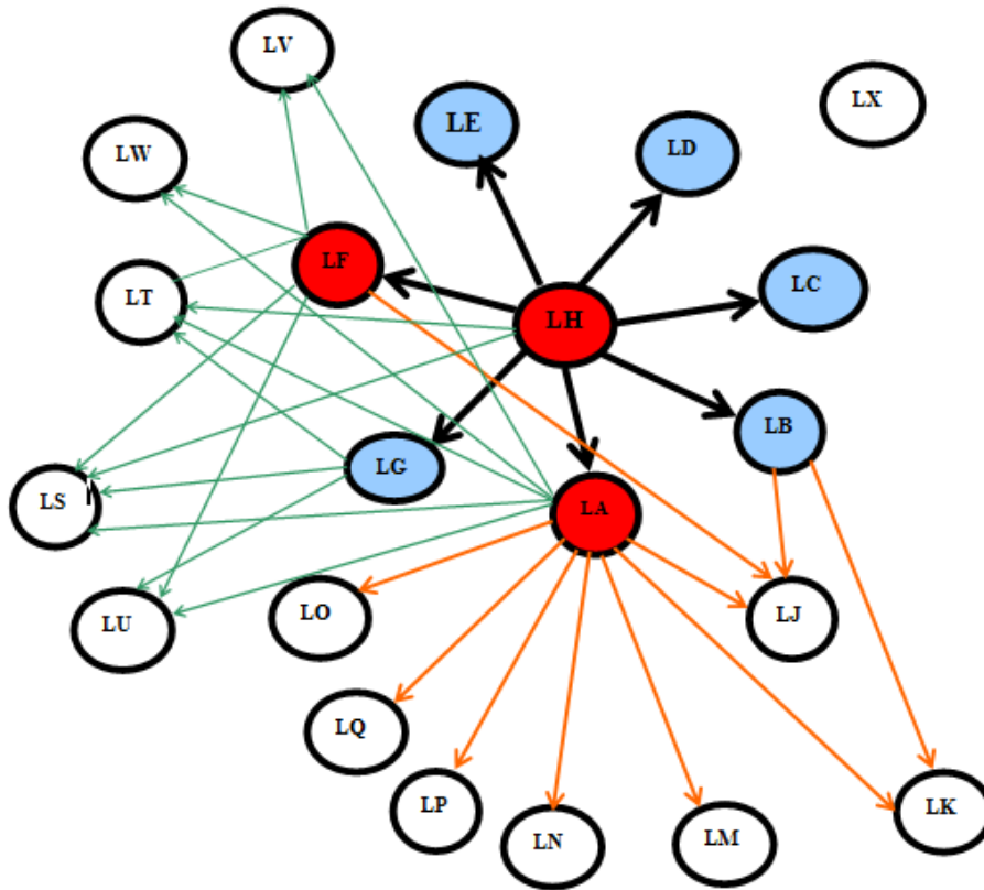
Figure 8.6: Concept of dominating sets.
