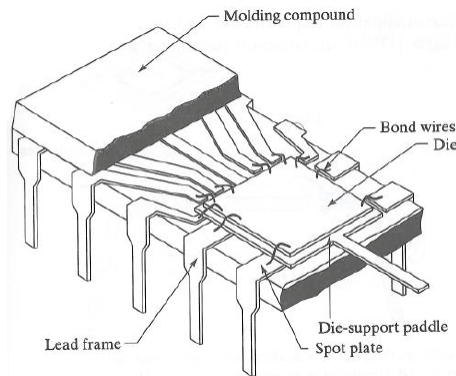
Figure 2.5: Back-End Processing [101].
