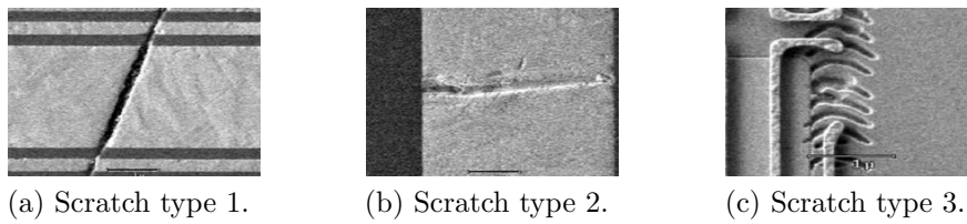
Figure 3.3: Scratches on wafers.
