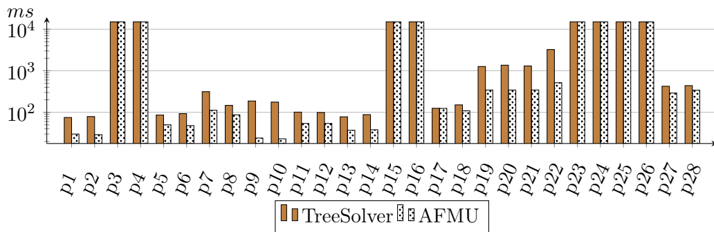
Figure 7.4: Results for the UCQProj test suite (logarithmic scale).
