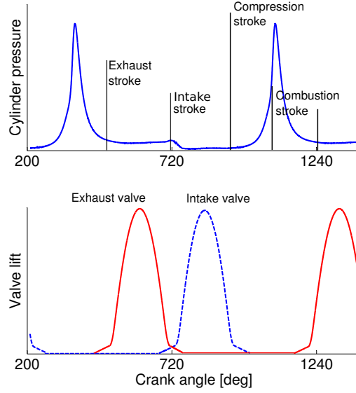
Figure 4.4: Engine cycles representation
