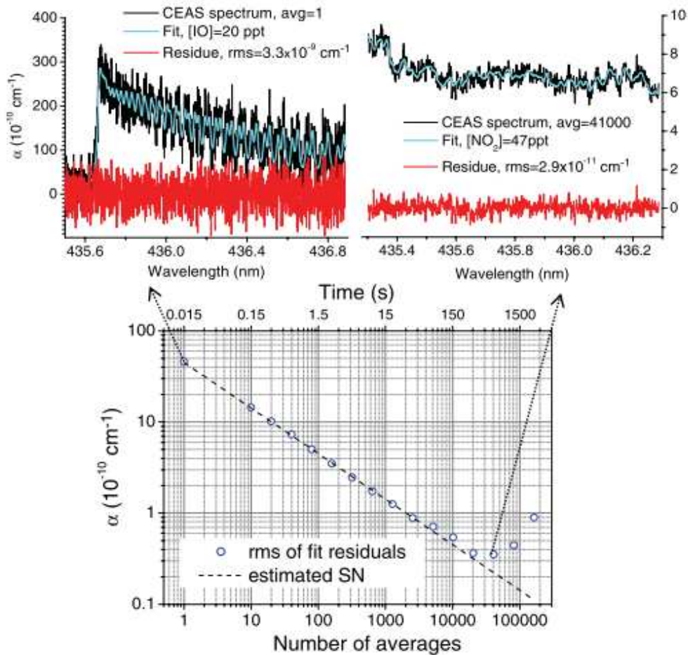
Figure 3.35: Top left: IO spectrum for a single 12 ms CCD exposure. Top right: spectrum of \text{NO}_2 from averaging 41 000 CCD exposures. Spectral fits using a linear combination of literature cross sections for IO and \text{NO}_2 yield the displayed molecular concentration. Fit residuals have rms values corresponding to the expected level of photon shot noise. At the bottom is a plot of the rms versus the averaging number.
