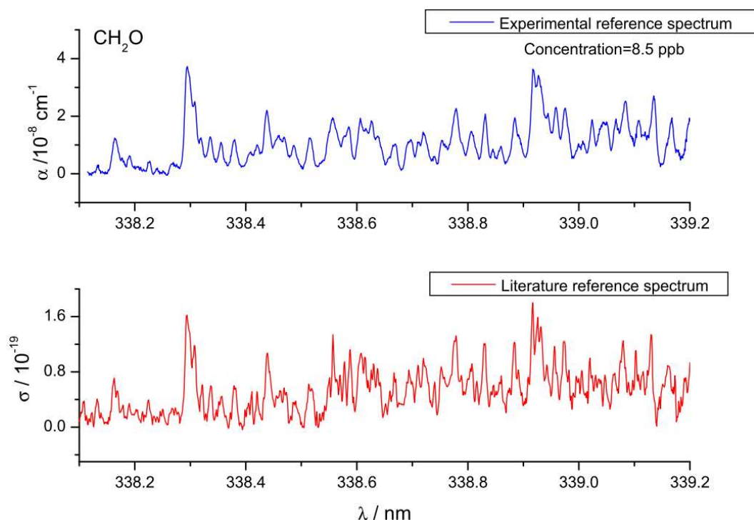
Figure 3.20: In blue, the experimental spectrum acquired at atmospheric pressure, used as a reference by the fit procedure. In red, UV absorption spectrum of CH 2 O around 338.5 nm from the literature [60], acquired at atmospheric pressure, and at a resolution of 0.35 cm -1 .
