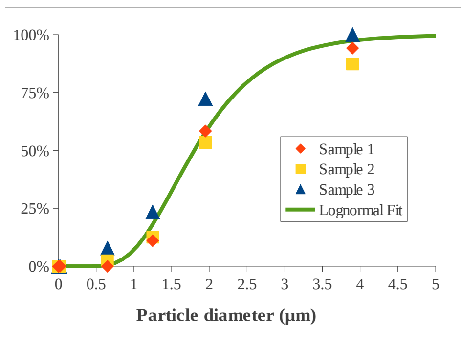
Figure A1-3: Cumulative mass size distribution measured using 6 stages cascade impactors. Solid line represents a log-normal fitting with a mean value of 1.8 µm and a standard deviation of 0.4.
