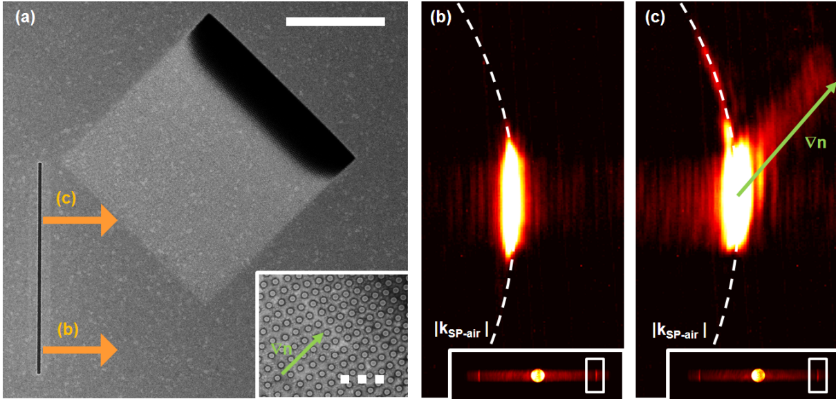
Figure 4.4.: GRIN slab - (a) SEM image of a GRIN slab ( 20 \times 20 \mu\text{m}^2 ) and a nanoslit source (250 nm wide, 20 \mu\text{m} long). The direction of increase in rod spacing defining the index gradient \nabla n is shown in the inset. The scale bars correspond to 10 \mu\text{m} (continuous) and 1 \mu\text{m} (dashed). - (b)+(c) LR micrographs in reciprocal space of SPs propagating outside (b) and inside (c) the GRIN structure, respectively. While in (b) just the mere SP resonance is visible, (c) demonstrates modulation of k_{SP} along the direction of the index gradient \nabla n .
