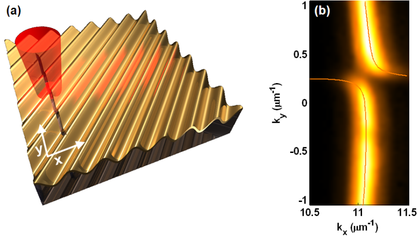
Figure 8.1.: (a) Plasmonic crystal sensing scheme. SPs are launched by monochromatic illumination of a nanogroove source oriented 45^\circ to a sinusoidal metal grating. - (b) IRF around the M-point of a P = 580/\sqrt{2} nm gold grating in a water environment, illuminated at \lambda_0 = 782 nm. The image was acquired by LR microscopy of the reciprocal space, theoretical modeling (solid line) was preformed as discussed in chapter 5 for a modulation amplitude \gamma = 3.7 \times 10^{-2} .
