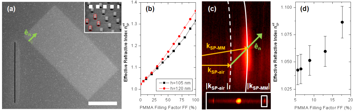
Figure 4.3.: (a) SEM image of a rectangular slab ( 15 \times 30 \mu m^2 ) made of PMMA rods of 91 \pm 5 nm diameter and a height of h_{PMMA} = 106 nm. A nanoslit (250 nm wide, 20 \mu m long) is used as an SP source. An SEM zoom of the rods taken at 52^\circ is shown in the inset. The interface normal \hat{e}_n is marked by the green arrow, scale bars correspond to 10 \mu m (continuous) and 1 \mu m (dashed), respectively. - (b) Dependence of the SP refractive index n_{SP}^{eff} on the lateral PMMA filling factor (FF), determined from calculations using the differential method [157, 158]. - (c) LR microscopy image in reciprocal space of SPs in an effective index medium (FF=0.18). The inset shows the full reciprocal space. The magnified area (white box) demonstrates the shift of the SP resonance from k_{SP-air} along the interface normal \hat{e}_n to the SP wavevector in the metamaterial k_{SP-MM} . - (d) n_{SP}^{eff} variation with FF, controlled by varying the rod spacings from 220 nm to 360 nm, determined from measurements of the direction \hat{k}_{SP} of the SP wavevector in LR microscopy reciprocal space images. Errors have been estimated by Gaussian propagation of the uncertainty in \hat{k}_{SP} measurement.
