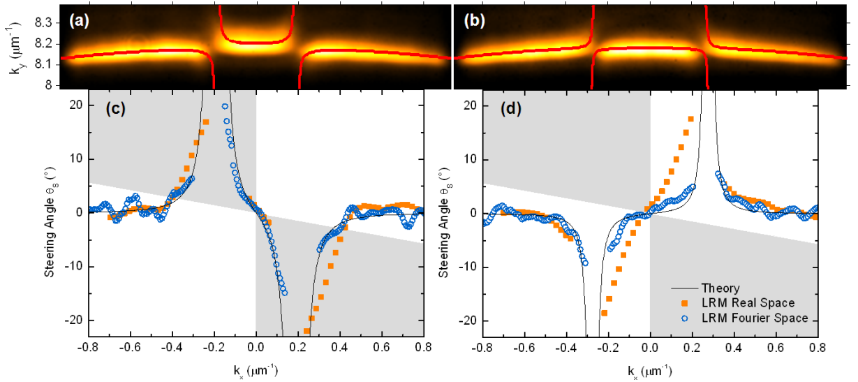
Figure 5.6.: 2PGs with periods P = 750/\sqrt{2} \text{ nm} < P_{\text{Bragg}} (left) and P = 790/\sqrt{2} \text{ nm} > P_{\text{Bragg}} (right) - (a+b) Detail of the IFD of 2PGs around the bandgap region from LR images. Calculated IFDs are superimposed with modulation depths \gamma = 0.020 and \gamma = 0.010 , respectively. - (c+d) Steering angle \theta_S as a function of k_x , extracted from real and reciprocal space LR images as well as calculations. Especially for P = 790/\sqrt{2} \text{ nm} a deviation of real space and Fourier space results is observed, which can be explained by the inherent convolution of the real space SPs with the still finite \delta k_x = 0.1 \text{ } \mu\text{m}^{-1}
