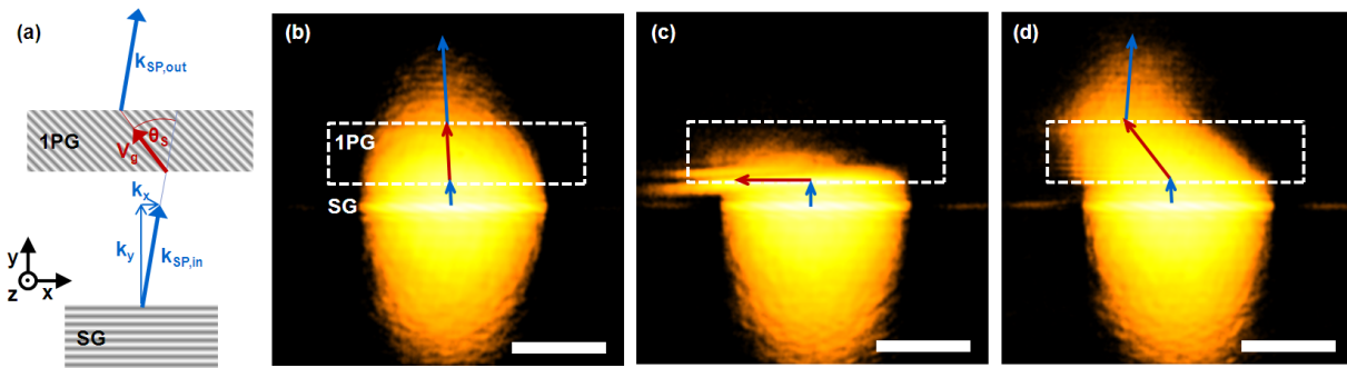
Figure 5.4.: Real space experiments - (a) Sketch of the experimental setup with source grating SG ( 100 \times 10.6 \mu\text{m}^2 , P = 760 \text{ nm} ) separated \sim 3.7 \mu\text{m} from a 1PG ( 150 \times 32 \mu\text{m}^2 , P = 760/\sqrt{2} \text{ nm} ). The incident SP wavevector \mathbf{k}_{\text{SP},\text{in}} as well as the group velocity \mathbf{v}_g and the steering angle of SPs \theta_s inside the grating are shown. - (b-d) LR real space images of SPs launched by the SG with varying in-plane component k_x = -0.53, +0.05, +0.19 \mu\text{m}^{-1} of \mathbf{k}_{\text{SP}} . Scale bars correspond to 50 \mu\text{m} .
