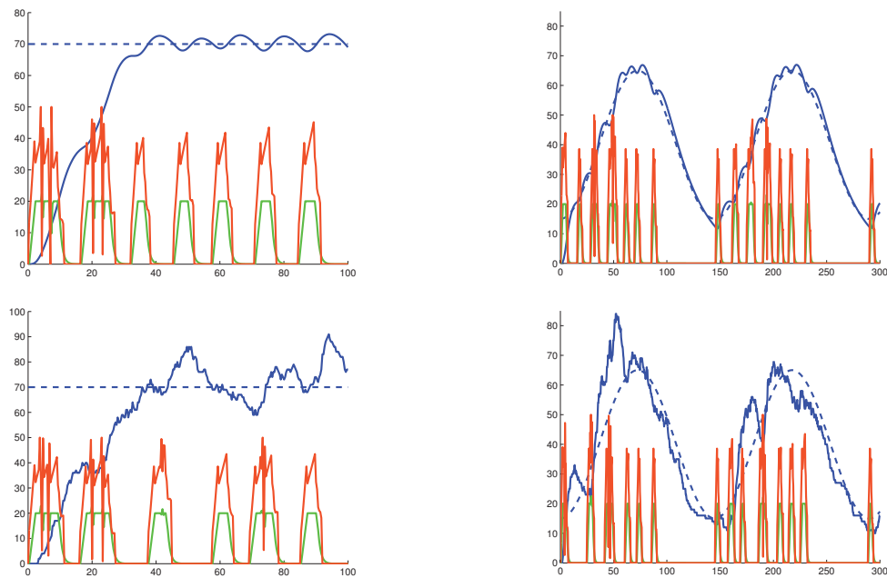
Fig. 6. Simulated control experiments. In all plots, dotted blue, orange, green, and solid blue represent the target protein profile, the applied osmolarity ( \times 50 ), the nuclear concentration of Hog1, and the concentration of the X protein. System behavior is either computed using a deterministic (ODE, top) or a stochastic (Gillespie, bottom) model. Time is in minutes.
