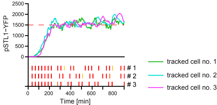
Figure 34: Repetitions of single cell control experiments. The control inputs for different single cell control experiments vary, even though the target value is the same (in this case 1500 f.u.). This highlights the need for closed loop control, because cellular variability requires different inputs to make different cells follow the target profile faithfully.
