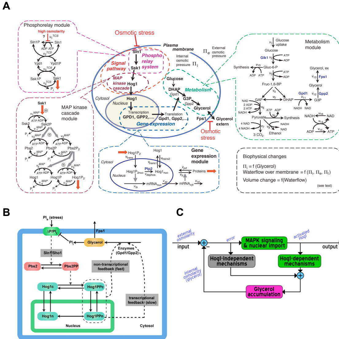
Figure 10: Different models of the HOG pathway. (A) Model of Klipp et al. [71] including gene expression and metabolic response to HOG pathway activation. The model consists of 32 ODE terms and 70 parameters. (B) Model by Zi et al. [75] developed to investigate the response of the HOG cascade to oscillating inputs. (C) The minimalistic linear model by Muzzey et al. [70] which has been used to identify the dominating feedback mechanism in the HOG cascade. (The figures have been taken from the corresponding publications.)
