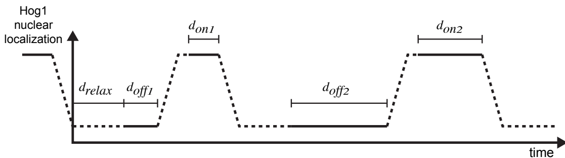
Figure 25: Hog1 profile constraints. A Hog1 profile is made up by reoccurring trapeze motifs, parametrized by a vector of plateau durations d_{on} and a vector of off-times d_{off} . The rise- and fall-off-times of the trapeze are fixed. In addition there is a minimal trapeze duration and a minimal relaxation time. All times that are not variable are indicated as dotted lines.
