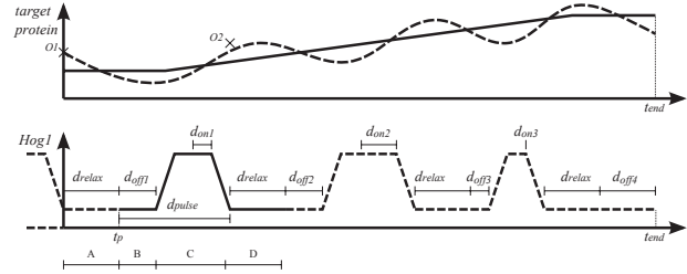
Fig. 4. Model predictive control for the GE controller. ( Bottom ) Hog1 profile with n = 3 motifs, defined by d_{off} = (2, 2, 1, 4) and d_{on} = (1, 2, 0) times. ( Top ) Corresponding protein profile (dotted line) with its reference profile (solid lines). This profile has been computed during period A, based on the observation O1 . During periods B and D, no stress will be applied ( osm_e = 0 ), whereas in period C, the signal transduction controller will be used to apply osmotic stresses yielding the desired Hog1 profile. Based on measurement O2 , the control strategy will be updated during period D. t_p denotes the start time of the current pulse.
