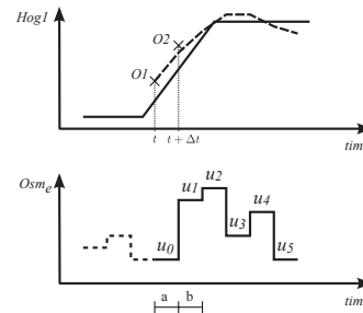
Fig. 5. Model predictive control for the ST controller. External osmolarity profile corresponding to osm_e = (u_i)_{i \in [0,5]} , computed during period a, based on observation O1 . u_0 will be effectively applied during period b, and a new osmolarity profile will be computed based on observation O2 .
