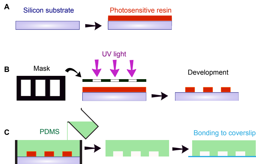
Figure 18: Microfabrication process. (A) A silicon wafer is covered with a photoresist. A regular thickness is achieved by rotating the wafer. The thickness of the photoresist layer is determined by its viscosity and by the rotational speed. (B) A pattern is transferred from a mask to the photoresist by UV light. After that the non-exposed part (negative photoresist) can be removed by a developing solution. (C) The pattern on the wafer can be used to construct microfluidic devices consisting of PDMS. Therefore fluid PDMS is applied to the master, polymerized and subsequently peeled off. After that the PDMS can be attached to a coverslip. (Modified illustration. Original by Agnès Miermont)
