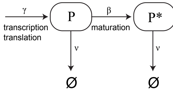
Figure 37: Gene expression model proposed by Charvin et al. [131]. The model comprises the unmaturred protein level ( P ) and the matured version ( P^* ). Unmaturred protein is produced with rate \gamma and then converted in a maturation step to matured protein with rate \beta . Both, unmaturred and matured protein are degraded with a rate proportional to \nu .
