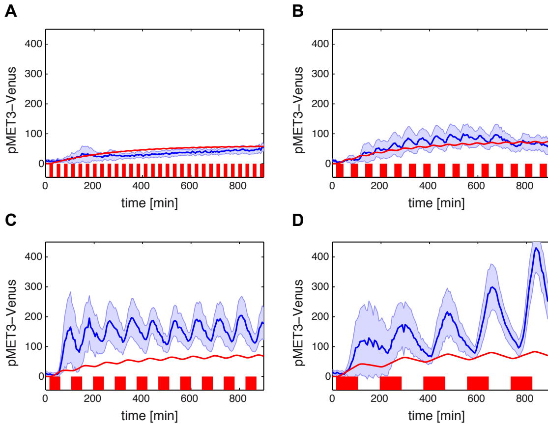
Figure 38: Calibration of pMET 3 -Venus gene expression and model fit. The cellular media is alternated between media without methionine (on, red bars) and media containing methionine (off). The on and off phases lasted 15 (A), 30 (B), 45 (C) and 90 (D) minutes. The mean cellular Venus fluorescence is shown as a blue line and the fluorescence standard deviation as a blue envelope. The model shown in Figure 37 was fitted to all four experiments simultaneously and the resulting model simulations are indicated as red lines.
