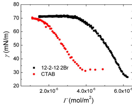
Fig. 6.13 Comparison of equations of state for the 12-2-12-2Br/100 mM NaBr system and CTAB/100 mM NaBr system
