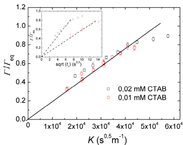
Fig. 4.9 The surface excess ratio \Gamma/\Gamma_{\text{eq}} as a function of K for two concentrations of CTAB, 0.01 (circles) and 0.02 mM (squares), where K = \frac{C_b}{\Gamma_{\text{eq}}} \sqrt{t_1} . The inset shows the \Gamma/\Gamma_{\text{eq}} as a function of \sqrt{t_1} . K was calculated using \Gamma_{\text{eq}} = 3.25 \times 10^{-6} \text{ mol/m}^2 for C_b = 0.01 \text{ mM} and 3.5 \times 10^{-6} \text{ mol/m}^2 for C_b = 0.02 \text{ mM} , taken from Fig. 4.7.
