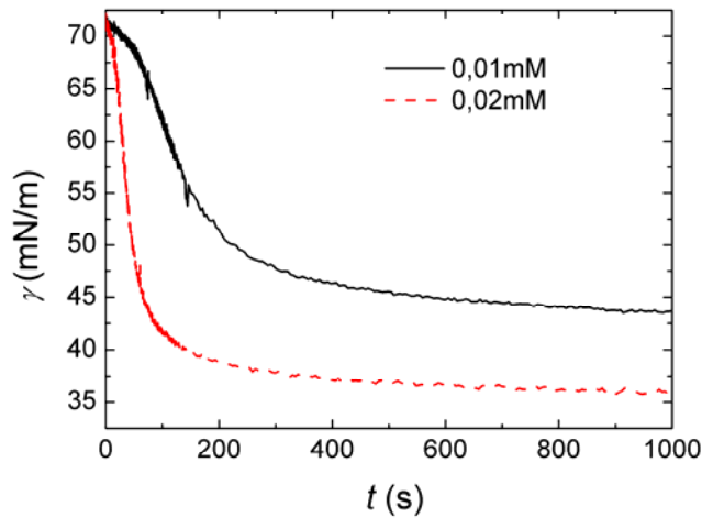
Fig. 4.2 Dynamic surface tension for the CTAB system with two concentrations (0.01 and 0.02 mM) in the presence of 100 mM NaBr.
