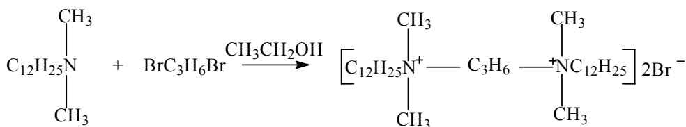
Scheme 3.2 Synthesis of 12-3-12·2Br
