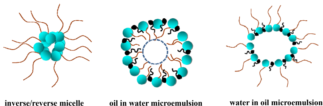
Scheme 2.3 Types of surfactant self assemblies
