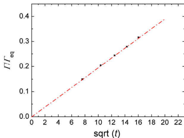
Fig. 6.14 Normalized surface concentration as a function of the square root of the bubble aging time t for 0.005 mM 12-2-12·2Br in the presence of 100 mM NaBr
