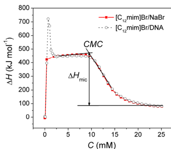
Fig. 8.2 Calorimetric titration curves of 150 mM [C_{12}mim]Br into 10 mM NaBr solution (■); 0.1 mM DNA solution in the presence of 10 mM NaBr (○).
