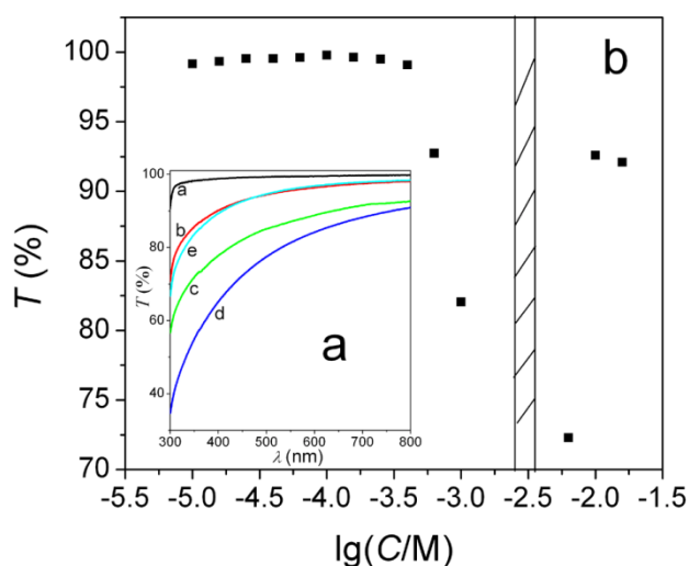
Fig. 8.5(a) Transmittance of [C_{12}mim]Br/DNA solutions ( T ) as a function of wavelength ( \lambda ) at various [C_{12}mim]Br concentrations ( C ). The [C_{12}mim]Br concentrations (a-e) are 0, 0.63, 1, 6.3, 10 mM; Fig. 8.5(b) [C_{12}mim]Br concentrations ( C ) dependence of the transmittance at 450 nm T^{450} (%) of [C_{12}mim]Br/DNA solutions. The striped region corresponds to the precipitation region.
