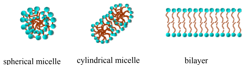
Scheme 2.2 Various types of micelles
