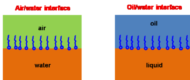
Scheme 2.1 Assembly of surfactants at the air/water interface and oil/water interface
