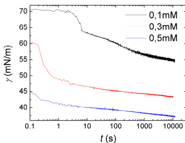
Fig. 6.4 Dynamic surface tensions of 12-2-12·2Br/H 2 O solutions, at concentrations close to CMC
