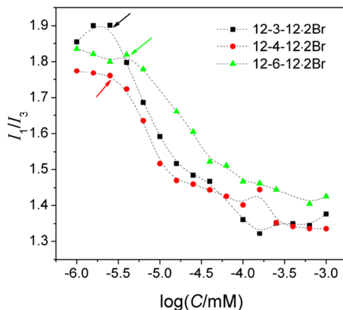
Fig. 7.14 Dependence of micropolarity in 12-O-12·2Br/DNA system on the surfactant concentration, where the DNA concentration is kept at 10^{-4} M.
