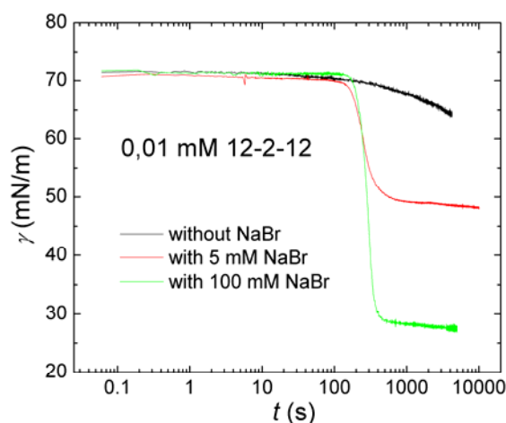
Fig. 6.7 Dynamic surface tensions of 0.01 mM 12-2-12-2Br solution with increasing concentrations of NaBr
