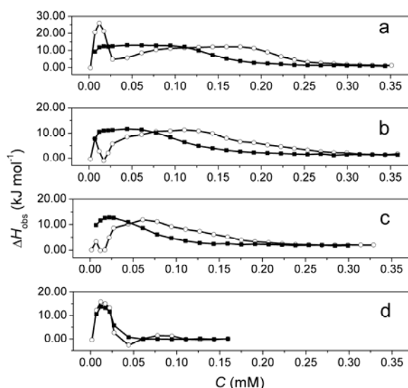
Fig. 7.7 Calorimetric titration curves of 12-3-12·2Br into brine (■) and 0.10 mM DNA solutions (○) with various NaBr concentrations: (a) 10 mM; (b) 15 mM; (c) 20 mM; (d) 50 mM at 298.15 K
