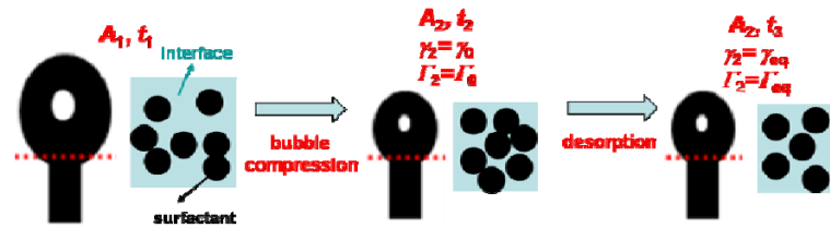
Scheme 5.1 Description of bubble compression and the desorption process, with the blue plane denoting the bubble interface and the black spots denoting the surfactant molecules
