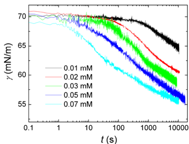
Fig. 6.3 Dynamic surface tensions of 12-2-12·2Br/H 2 O solutions, at different concentrations far below CMC
