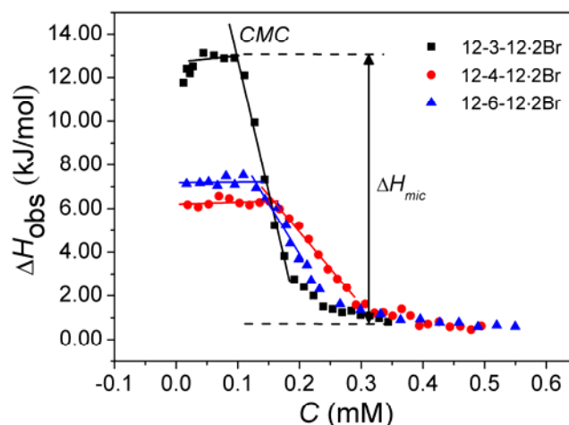
Fig. 7.13 Calorimetric titration curves of 12-O-12:2Br (O=3, 4, 6) into 100 mM NaBr
