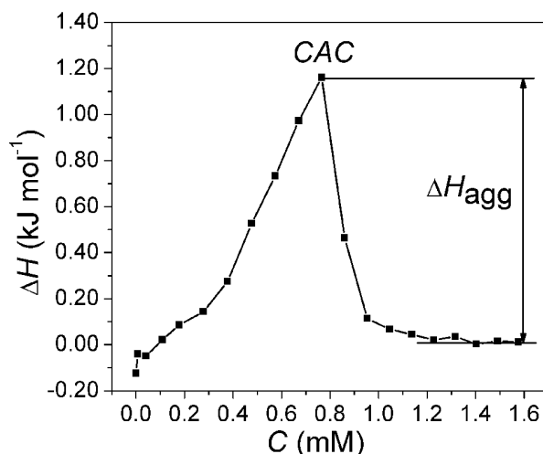
Fig. 8.3 Calorimetric titration curve of 10 mM [C 12 mim]Br into 0.1 mM DNA solution.
