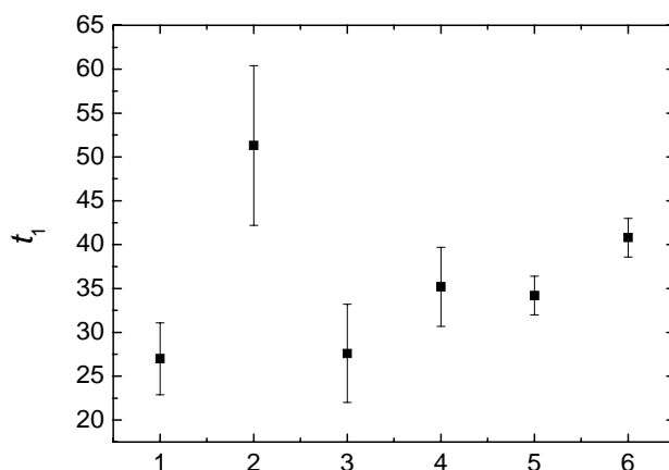
Fig 5.8 Characteristic times for desorption for different surfactant systems, from left to right (1 to 6) are C_{12}E_6 , CTAB/100 mM NaBr, TTAB/100 mM NaBr, AOT/100 mM NaCl, AOT/100 mM KCl, AOT/50 mM MgCl_2 respectively. Each value is based on the measurements for the same surfactant system averaged from measurements at different concentrations.
