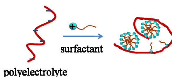
Scheme 2.10 Aggregation process of surfactants around the polyelectrolyte
