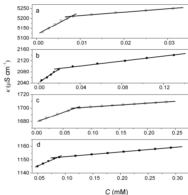
Fig. 7.1 Dependence of conductivity ( \kappa ) on the 12-3-12·2Br concentration with various NaBr concentrations: (a) 50 mM; (b) 20mM; (c) 15 mM; (d) 10 mM at 298.15 K
