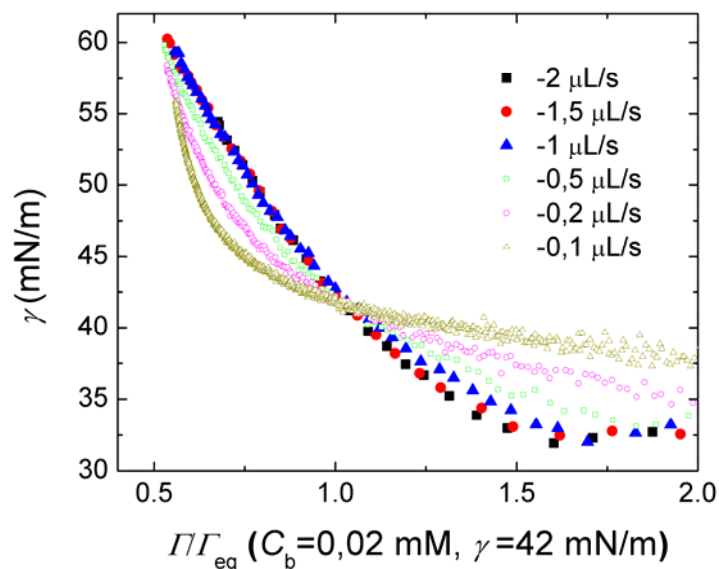
Fig. 4.4 Surface tension \gamma as a function of the calculated surface concentration \Gamma , normalized by \Gamma_{eq} at various compression rates. \Gamma_{eq} is the equilibrium surface concentration for 0.02 mM C_{12}E_6 , where the equilibrium surface tension \gamma_{eq}=42 mN/m. Note that at low compression speeds the calculated value of \Gamma does not correspond to the actual value of \Gamma because desorption or adsorption occurs.
