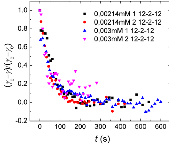
Fig. 6.16 Dependence of normalized surface tension on the time during the desorption process for 12-2-12·2Br systems with different surfactant bulk concentrations, and the line is the fitting of
