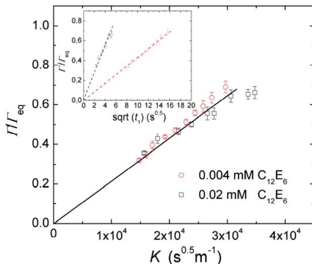
Fig. 4.8 The surface excess ratio \Gamma/\Gamma_{\text{eq}} as a function of K for two concentrations of C_{12}E_6 , 0.004 (circles) and 0.02 mM (squares), where K = \frac{C_b}{\Gamma_{\text{eq}}} \sqrt{t_1} . The inset shows the \Gamma/\Gamma_{\text{eq}} as a function of \sqrt{t_1} . K was calculated using \Gamma_{\text{eq}} = 2.1 \times 10^{-6} \text{ mol/m}^2 for C_b = 0.004 \text{ mM} and 3 \times 10^{-6} \text{ mol/m}^2 for C_b = 0.02 \text{ mM} , taken from Fig. 4.6.
