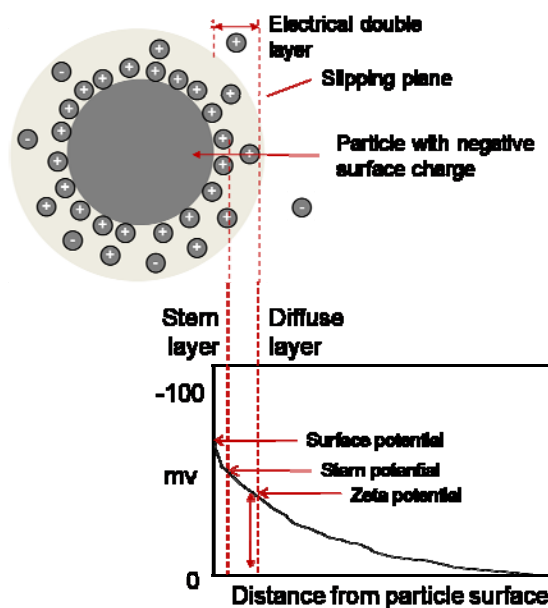
Scheme 3.9 Illustration of the zeta potential and electrical double layer
