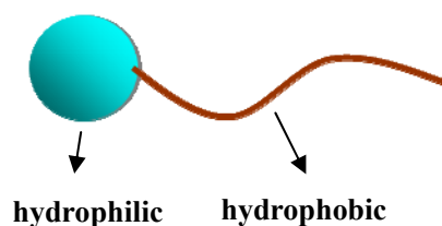
Scheme 1.1 Typical surfactant structure
