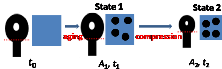
Scheme 4.1 Description of the proposed bubble compression method, with the blue plane denoting the bubble interface and the black spots denoting the surfactant molecules
