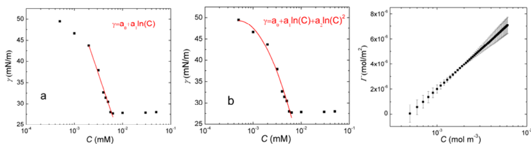
Fig. 6.11 Equilibrium surface tension of 12-2-12-2Br in 100mM NaBr solution as a function of surfactant bulk concentration, fitted with the Equation 6.7 (a) and fitted with Equation 6.8 (b); dependence of surface concentration on the surfactant bulk concentration (c).
