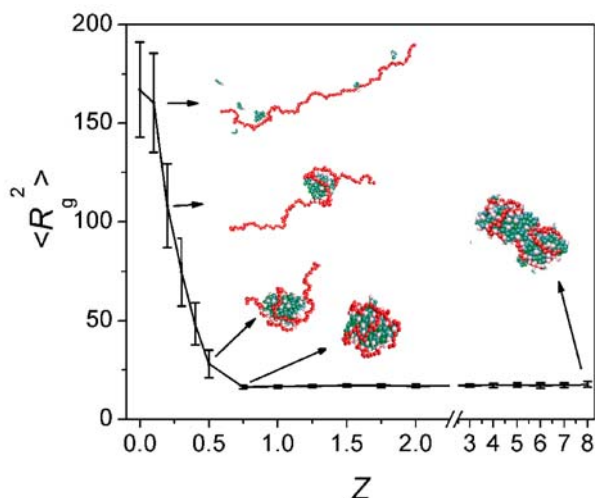
Fig. 8.10 Mean-square radius of gyration \langle R_g^2 \rangle of polyelectrolyte (in the unit of \sigma^2 ) as a function of (+/-) charge ratio Z in the system. At each Z , 600 equilibrium simulation steps were
