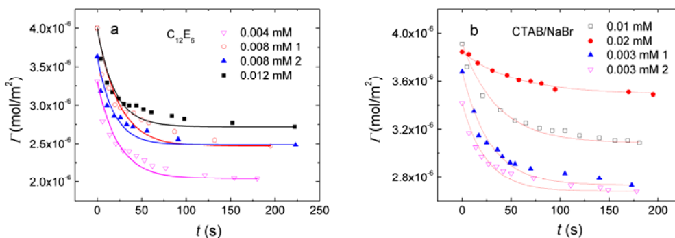
Fig. 5.4 Exponential fits for the calculated surface concentration in time for two systems C_{12}E_6 (a) and CTAB/100 mM NaBr (b).
