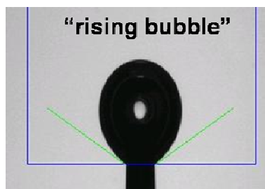
Scheme 3.5 The rising air bubble configuration
