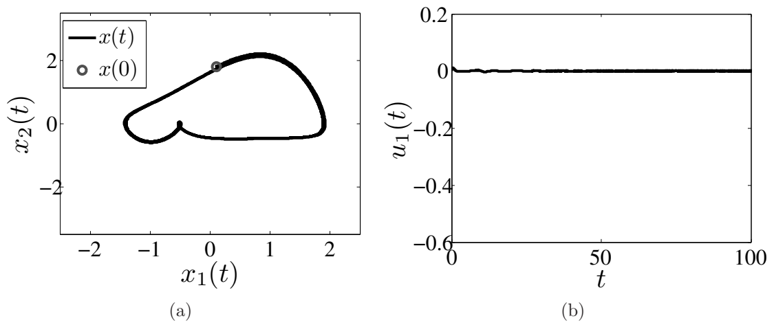
Figure 8.25: TUPO2 stabilized using the aPBC with k = -0.125 and x(0) = [0.1, 1.8]' . (a) State space and (b) time series of the control effort.
