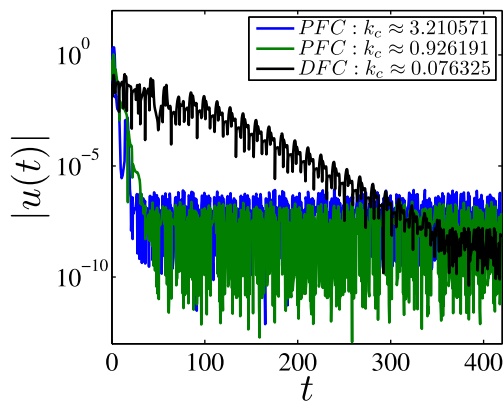
Fig. 5. Time series of the magnitude of the control signal u(t) of the target UPO of the vdP system for a = 0.988 using DFC with k_c = 0.07632510479 (black line), PFC with k_c = 0.92619140625 (green line) and PFC with k_c = 3.2105712890625 (blue line). (For interpretation of the references to colour in this figure legend, the reader is referred to the web version of this article.)
