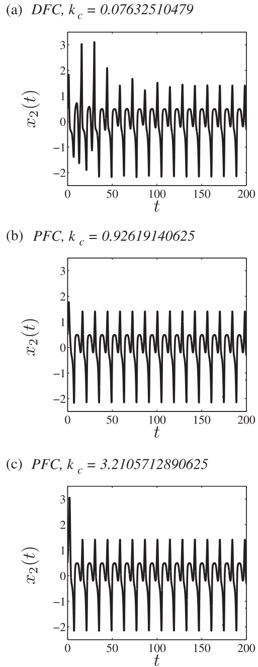
Fig. 4. Time series of the controlled x_2(t) showing the stabilization of the target UPO of the vdP system for a = 0.988 using (a) DFC with k_c = 0.07632510479 , (b) PFC with k_c = 0.92619140625 and (c) PFC with k_c = 3.2105712890625 .
