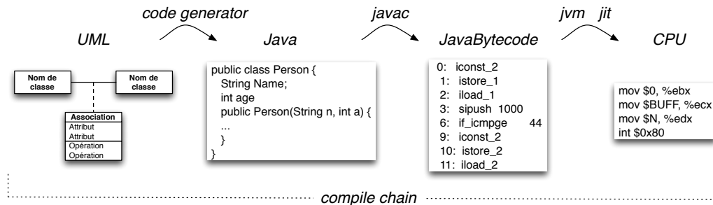
Figure 2.14: Java compile chain.
