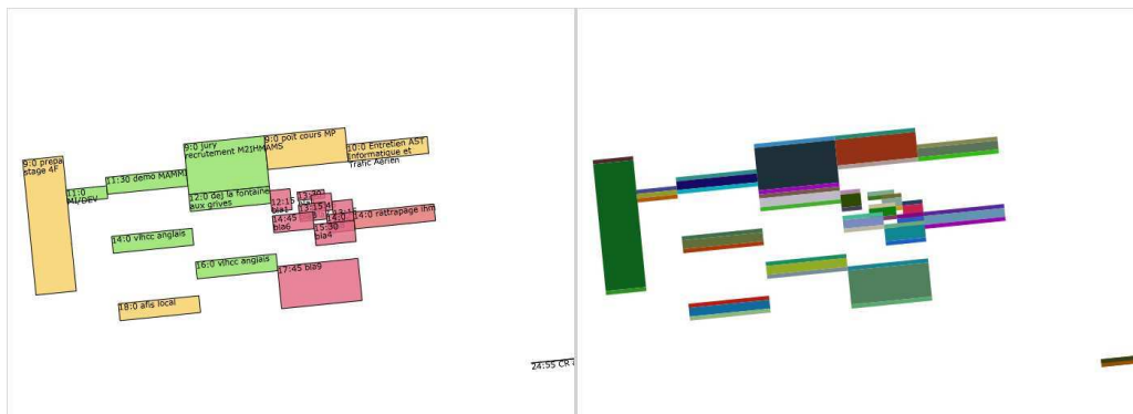
Figure 2.9: The display and picking views of the week view of a calendar.
