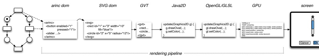
Figure 2.13: MPIA-Arinc rendering pipeline.
