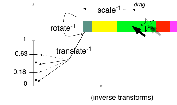
Figure 2.7: Inverse transformation for a drag of the thumb of a scrollbar.
