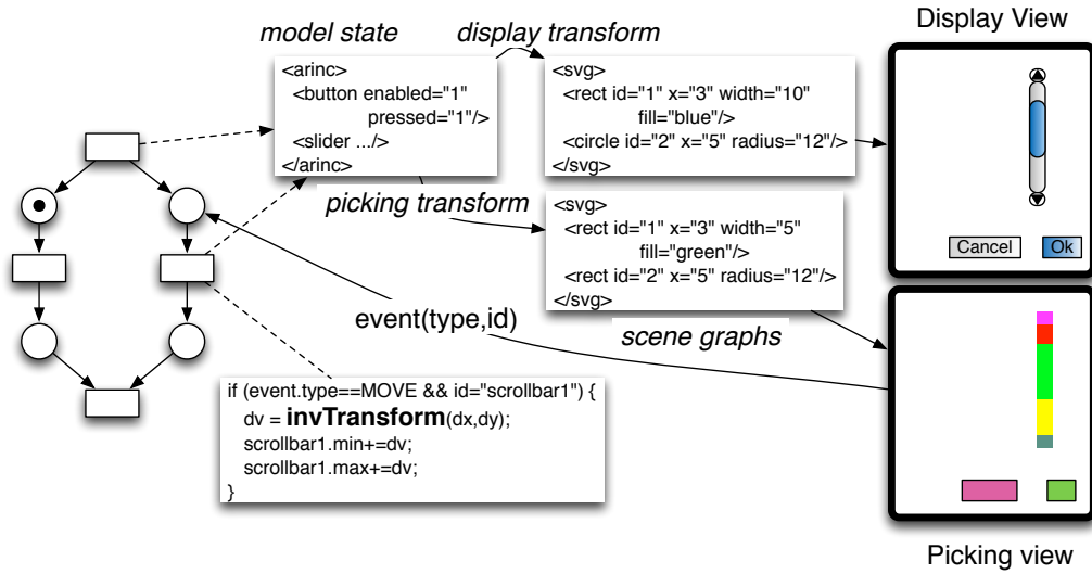
Figure 2.8: MPIA-Arinc final architecture: the controller code handles user events with minimum knowledge of the graphics by using the inverse transformation (in bold).
