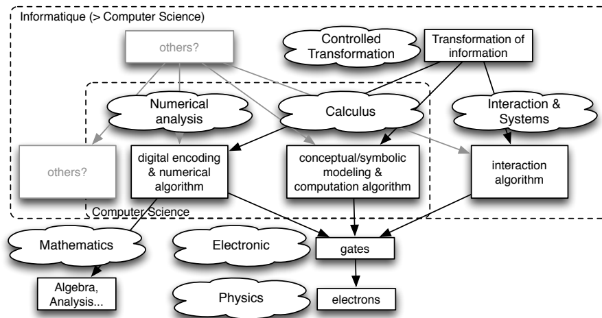
Figure 5.3: Informatics is more than Computer Science
