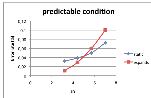
Figure 3.4: ... but they make more errors when ID>5
