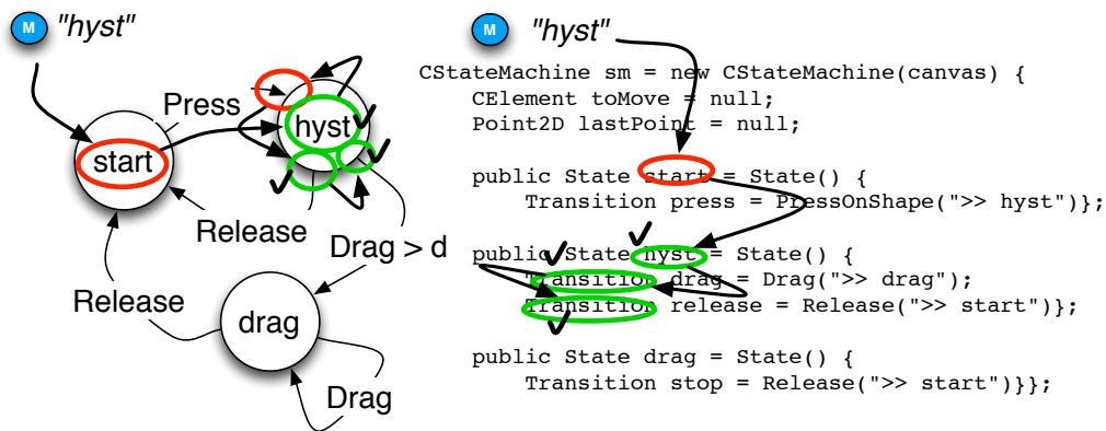
Figure 4.6: ScanVis for the task "find the entering transitions of state 'hyst'"
