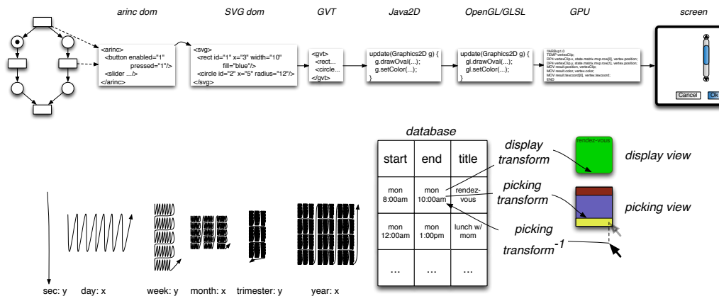
Figure 5.8: The rendering pipeline and forward transformation and inverse transformations help design and code interactive graphics
