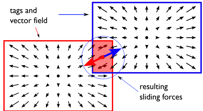
Figure 2.16: Vector field inside tags and the resulting sliding forces (from [Tis11]).
