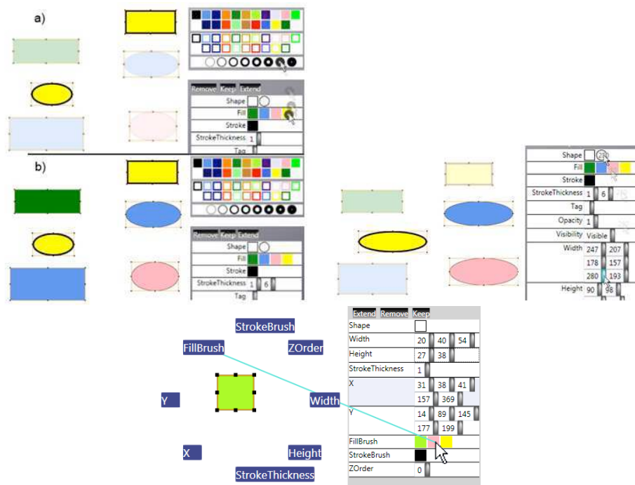
Figure 3.11: ManySpector interactions: from a sample to a shared value (left), from a shared value to a shared value (middle), from a clone to a shared value (right) to specify a dependency
