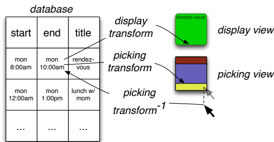
Figure 2.10: Principles of a week-view calendar architecture with MDPC.
