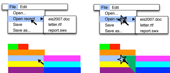
Figure 2.3: Display and picking views of a resting menu (left) and while navigating (right).
