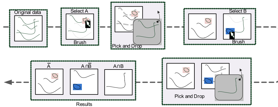
Figure 3.7: Implicit intersection boolean operation by direct manipulation
