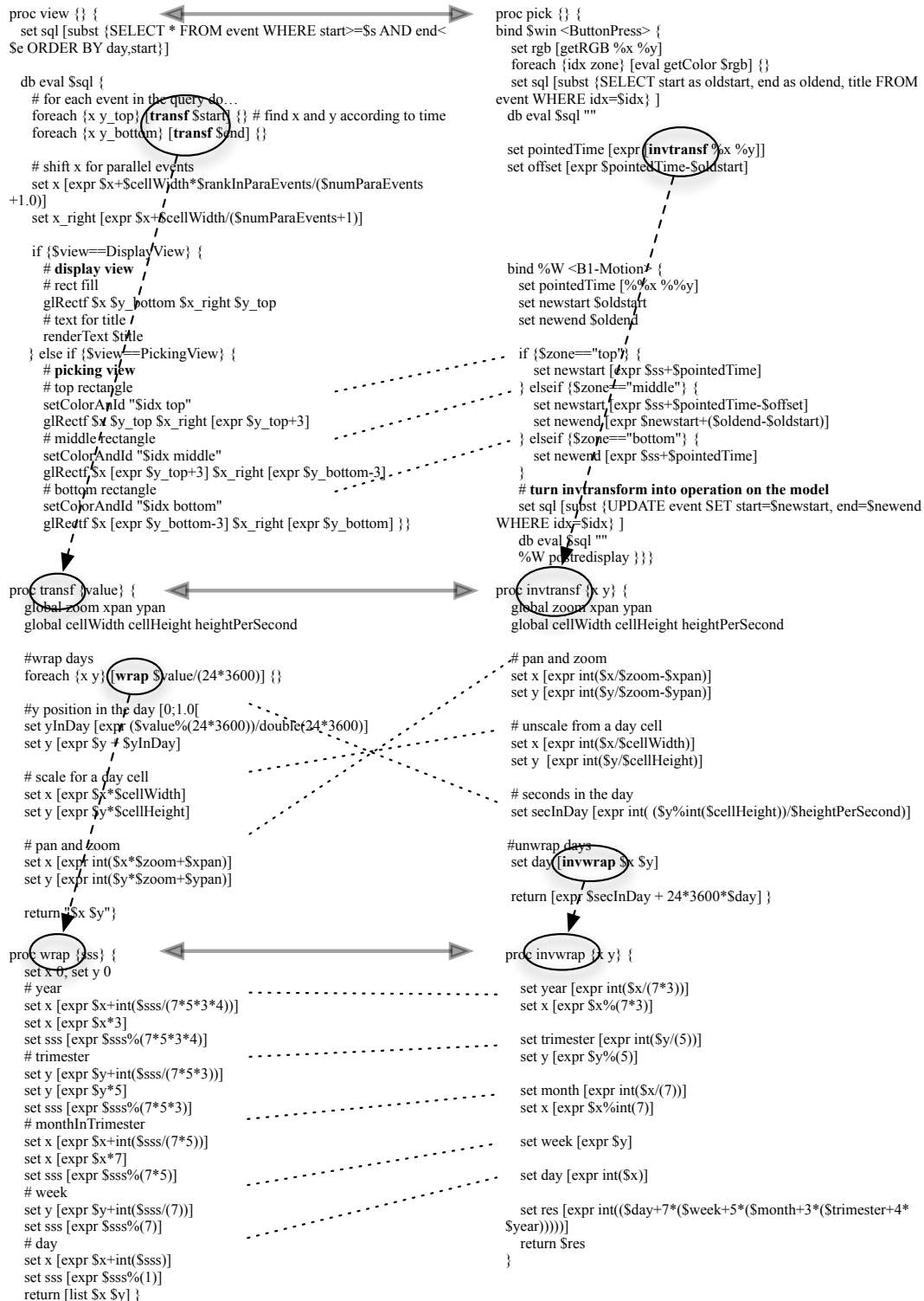
Figure 2.12: Actual code for calendar in Tcl. Left: disp. & pick. views, transformation (transf) and wrapping (wrap) - Right: their inverse (pick, invtransf, invwrap). Note the symmetry or asymmetry of functions and their inverse.
