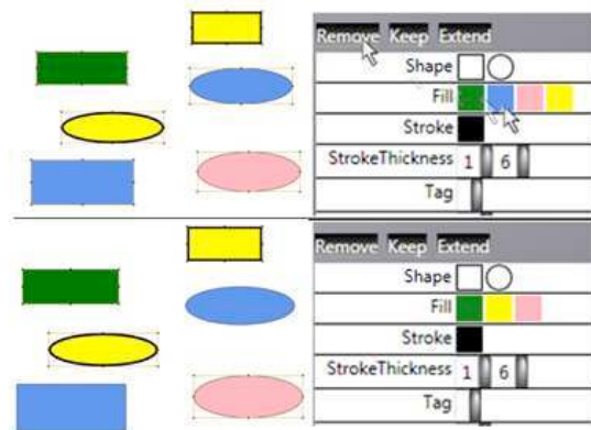
Figure 9. The user drags the Remove tool onto the “fill: blue” shared value. Blue objects are removed from the selection.
