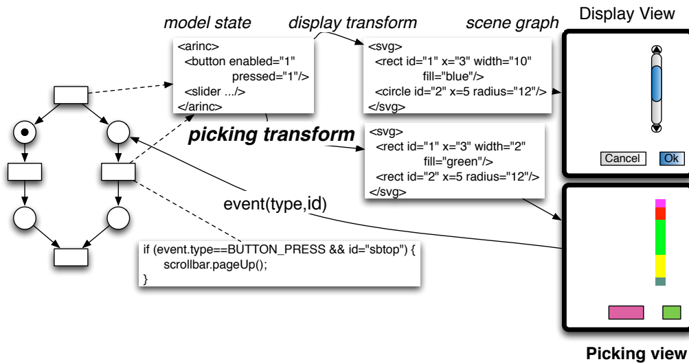
Figure 2.4: Architecture of the MPIA-Arinc application with picking transform and view (in bold).
