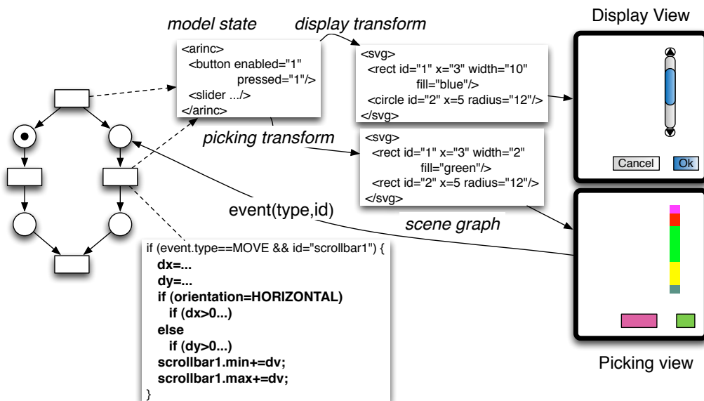
Figure 2.5: The controller still contains code (in bold) related to graphics when handling thumb dragging.
