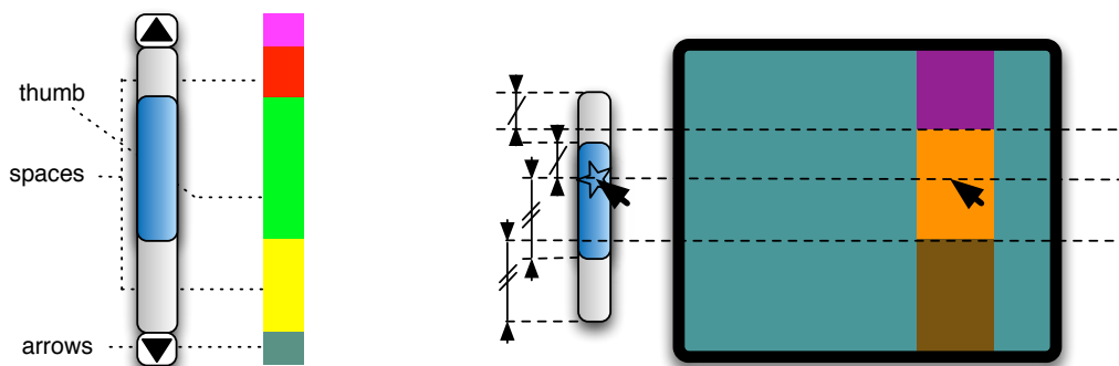
Figure 2.2: Display and picking views of a resting scrollbar (left) and while manipulating the thumb (right).
