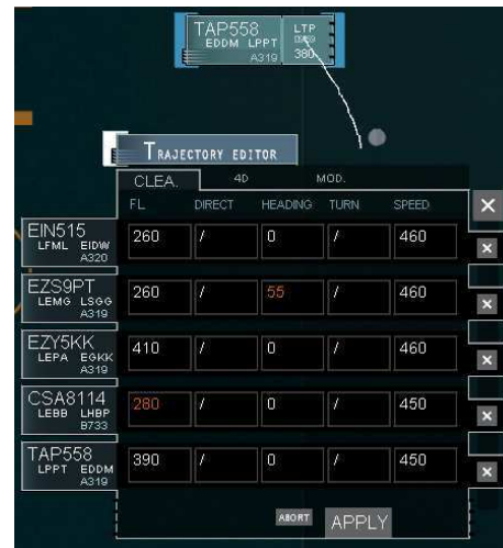
Figure 3.9: Partial accomplishment of actions with MAMMI’s trajectory editor
