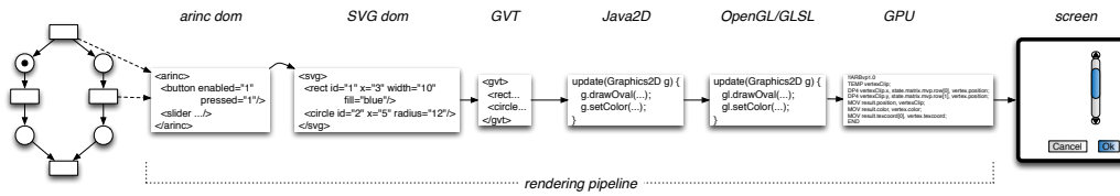
Figure 2.13: MPIA-Arinc rendering pipeline.
