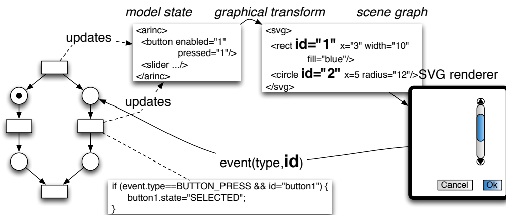
Figure 2.1: The MPIA-Arinc application refactored with MVC
