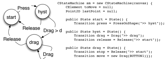
Figure 1. Two representations of the same program using various graphical features.
