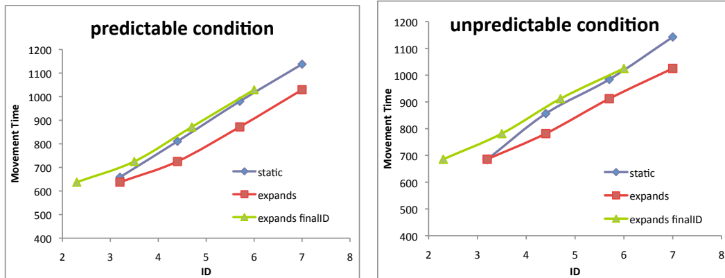
Figure 3.3: (left) When expansion is predictable, users are as fast as if the targets were double the size. (right) Even if expansion is unpredictable, users are still as fast as if the targets were double the size (surprise, and confirmation of M&B)...
