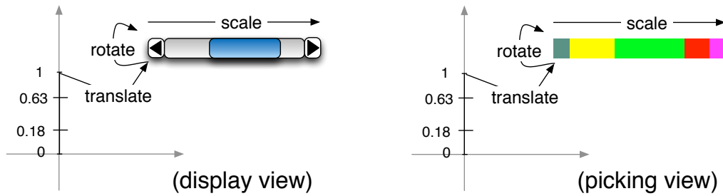
Figure 2.6: Graphical transformations from the model of a scrollbar to the graphics.
