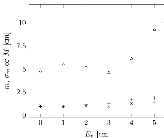
Figure 4.12: Statistical results: three sources above an homogeneous ground, with different accuracies on sources positioning. The frequency range analysis is reduced to [100-2 000] Hz. m (+), \sigma_m (x), M ( \triangle ).
