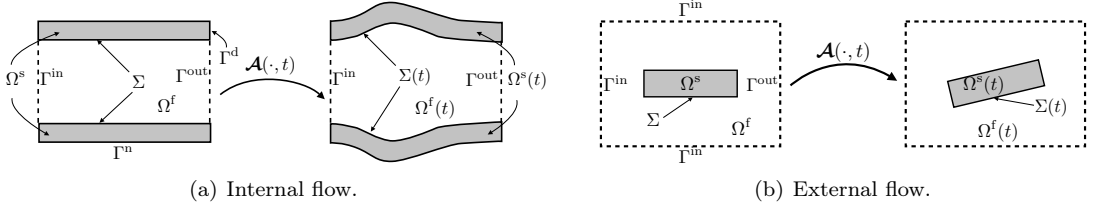
Figure 1.1: Geometrical fluid-structure configurations.
