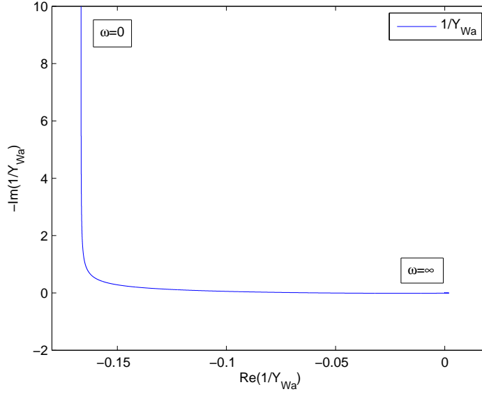
FIGURE 5.8 – Impédance \frac{1}{Y_{W_a}}
