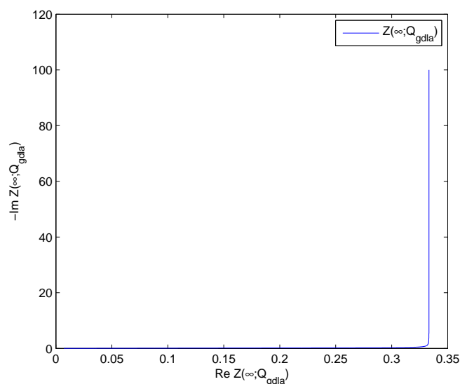
FIGURE 5.12 – Impédance Z(\infty; Q_{gdl_a})
