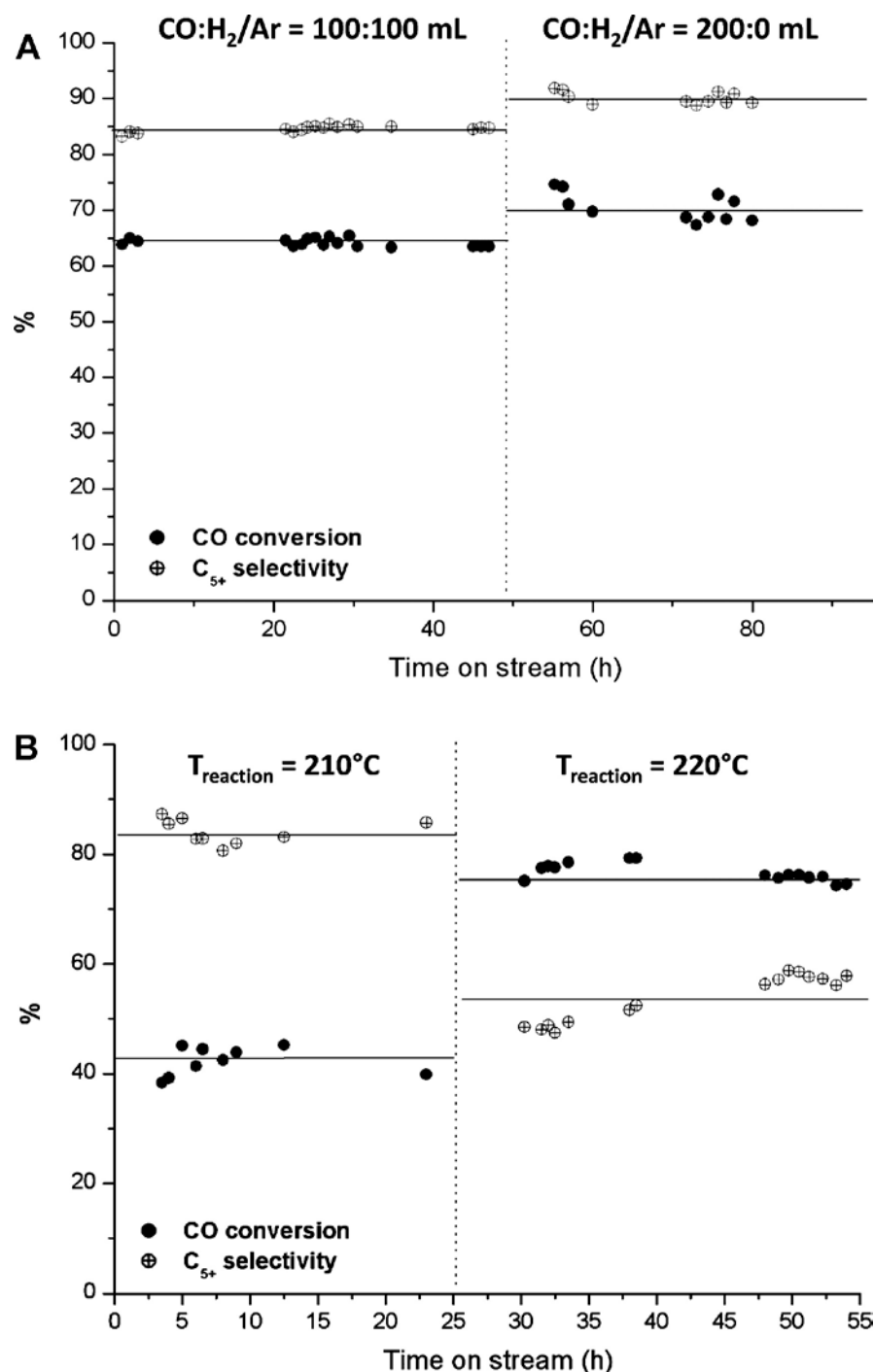
Figure 7. FTS activity and C 5+ selectivity obtained on the Co/SiC (A) and Co/ Al 2 O 3 (B) catalysts. (A) Co/SiC. Reaction conditions: H 2 :CO molar ratio = 2, total pressure = 40 atm., reaction temperature = 220°C. The Co/SiC was tested both under a diluted and pure flow of synthesis gas. (B) Co/Al 2 O 3 . The tests were carried out under a diluted mixture at 210°C and 220°C in order to avoid the problem of temperature runaway. The catalytic results are obtained after a period of stabilization, i.e. 100 h, under diluted synthesis gas and argon mixture under the same reaction conditions.
