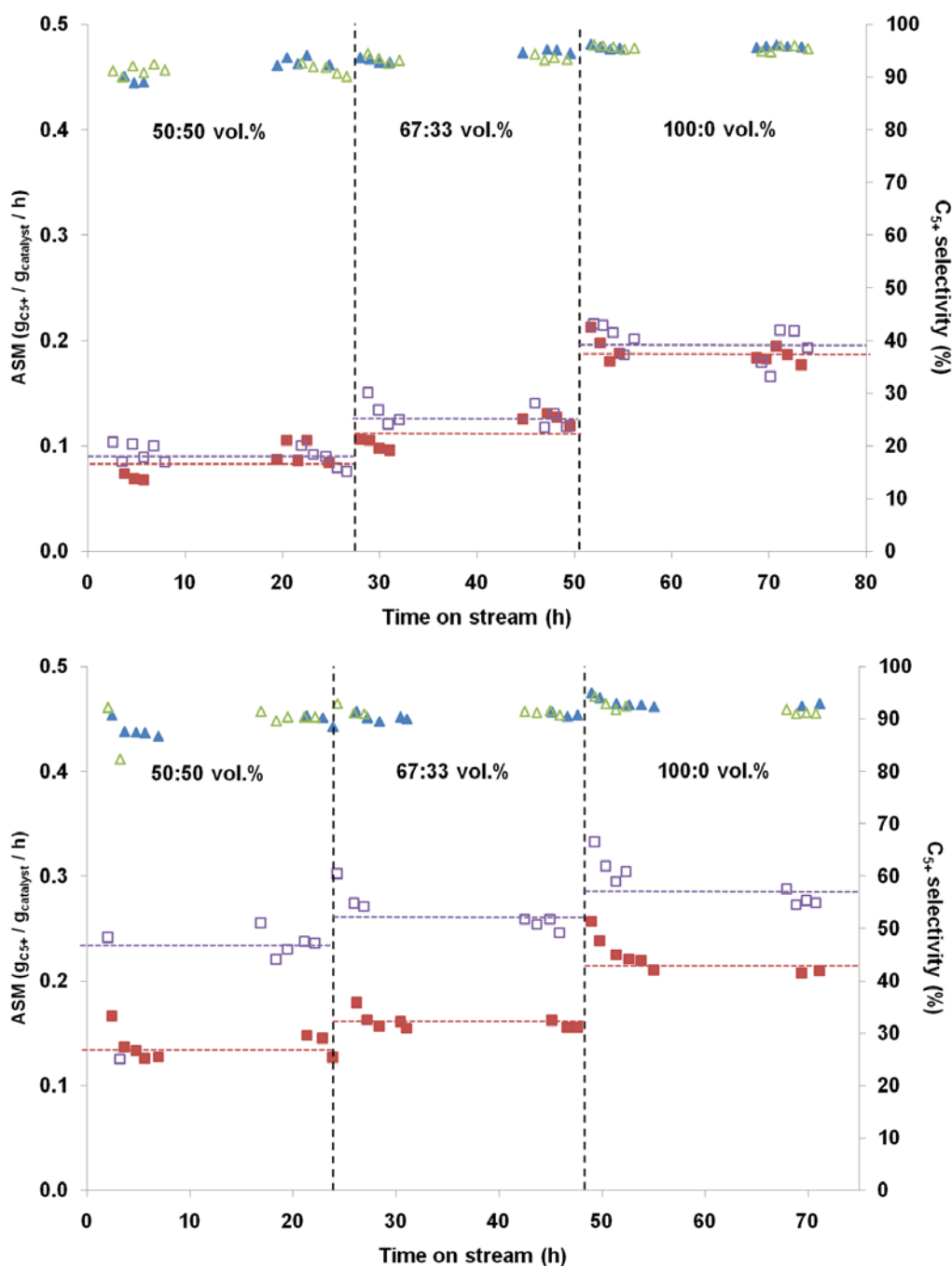
Figure 5. FTS performance on the different cobalt-based SiC catalysts with cobalt loading of (A) 10 wt.% and (B) 30 wt.% as a function of the H_2:CO concentrations. (■) ASM of SiC-LP supported catalyst, (□) ASM of SiC-HP supported catalyst, (▲) C_{5+} selectivity of SiC-LP supported catalyst, (△) C_{5+} selectivity of SiC-HP supported catalyst.
