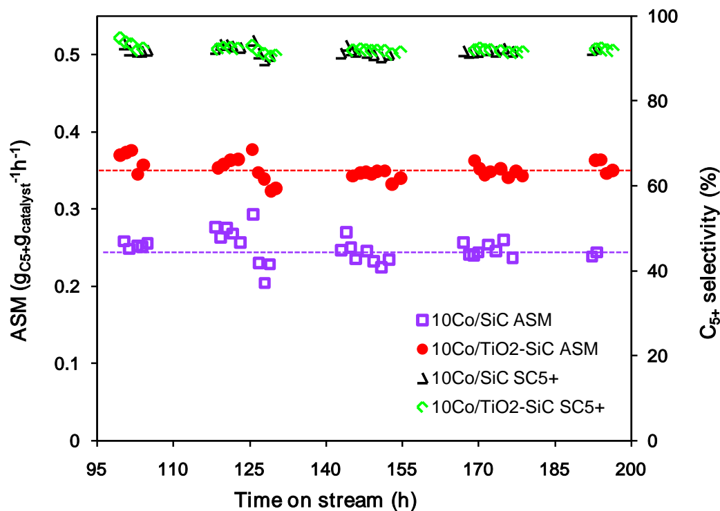
Figure 10. FTS performance and stability of the 10Co/SiC and 10Co/TiO 2 -SiC catalyst as a function of time on stream at 230 °C. Reaction conditions: H 2 /CO molar ratio = 2, pure syngas, total pressure = 40 bar, GHSV = 2850 h -1
