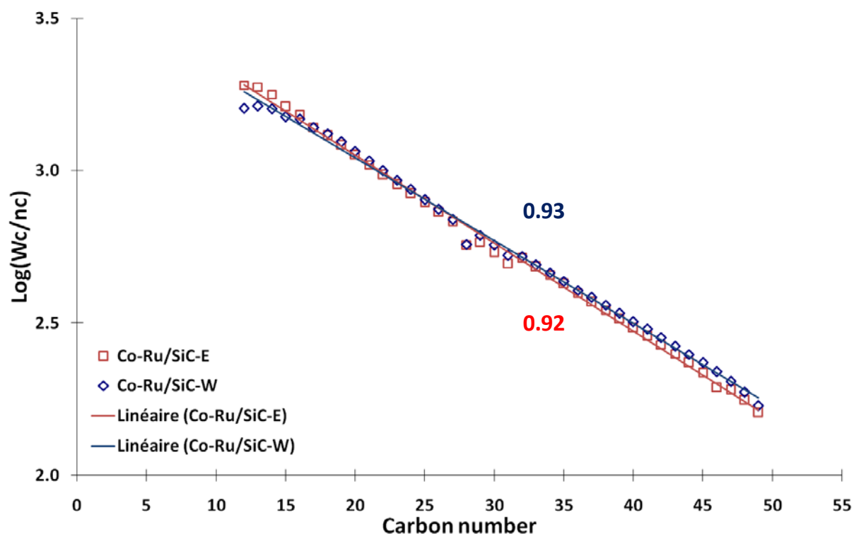
Figure 8. Calculated chain growth factor ( \alpha ) from the linear portion of the hydrocarbons.
