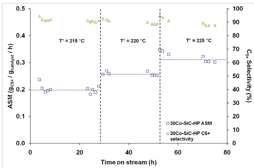
Figure 6. FTS performances on the 30Co/SiC-HP as a function of the reaction temperature. Reaction conditions: catalyst weight = 5 g, Co weight = 1.5 g, H 2 /CO = 2, total pressure = 4 MPa, space velocity = 1900 h -1 .
