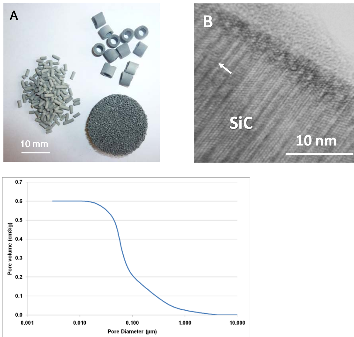
Figure 1. (A) Silicon carbide (SiC) with different macroscopic shapes synthesized according to the gas-solid reaction. (B) HR-TEM micrograph showing the presence of an amorphous layer constituted by a mixture of \text{SiO}_2 and \text{SiO}_x\text{C}_y on the SiC surface and a high number of stacking faults along the [111] growth axis. (C) Representative pore size distribution of the SiC support measured by mercury intrusion.
