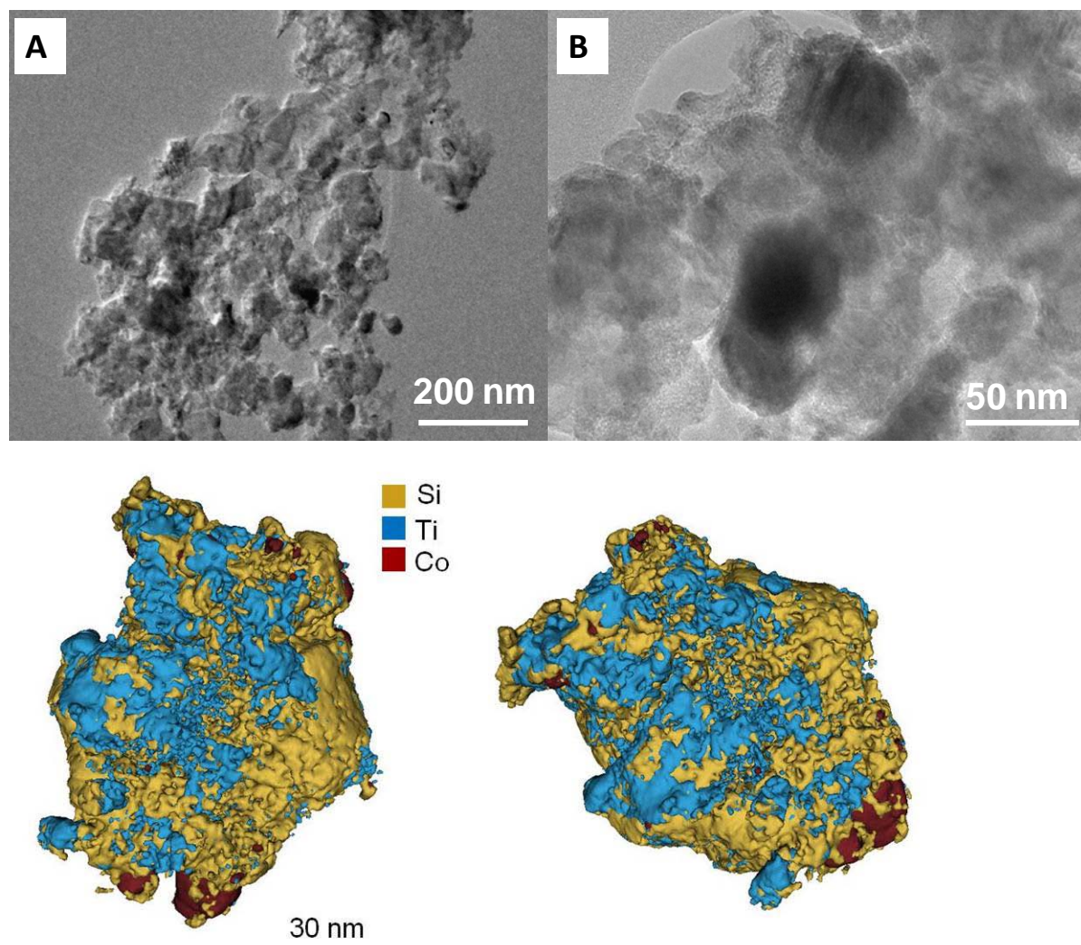
Figure 8. (A, B) TEM images of the 10Co/SiC. (C, D) EFTEM images of 10Co/TiO 2 -SiC showing the interaction of the cobalt particles with the different compounds of the support: Ti (blue), Si (yellow), Co (red). The catalyst was calcined at 350 °C for 2 h followed by a
