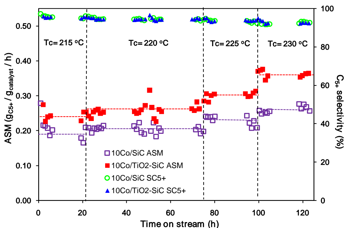
Figure 9. FTS performance and stability of the 10Co/SiC and 10Co/TiO 2 -SiC catalyst as a function of the reaction temperature. Reaction conditions: H_2/CO molar ratio = 2, pure syngas, total pressure = 40 bar, GHSV = 2850 h -1 . The catalysts tested have already been evaluated in the FTS reaction at 215 °C and under a GHSV of 1900 h -1 during about 100 h on stream (not reported).
