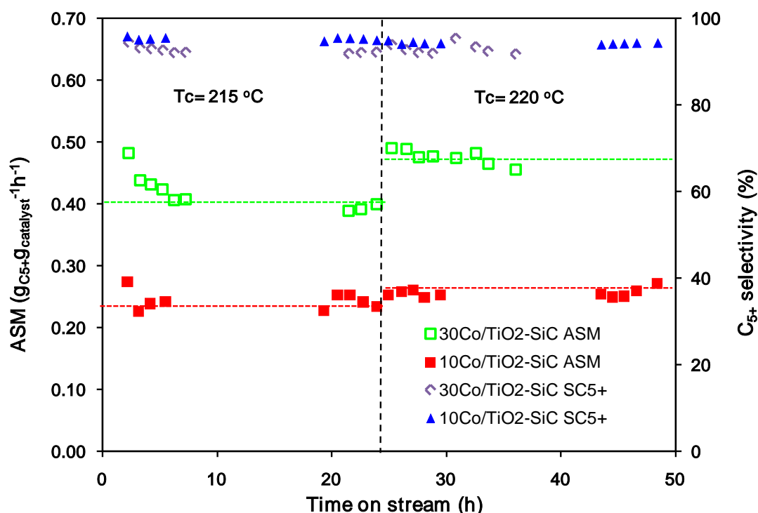
Figure 12. FTS activity and C 5+ selectivity as functions of time on stream on 10Co/TiO 2 -SiC and 30Co/TiO 2 -SiC catalysts. Reaction conditions: H 2 /CO molar ratio = 2, pure syngas, total pressure = 40 bar, GHSV = 2850 h -1
