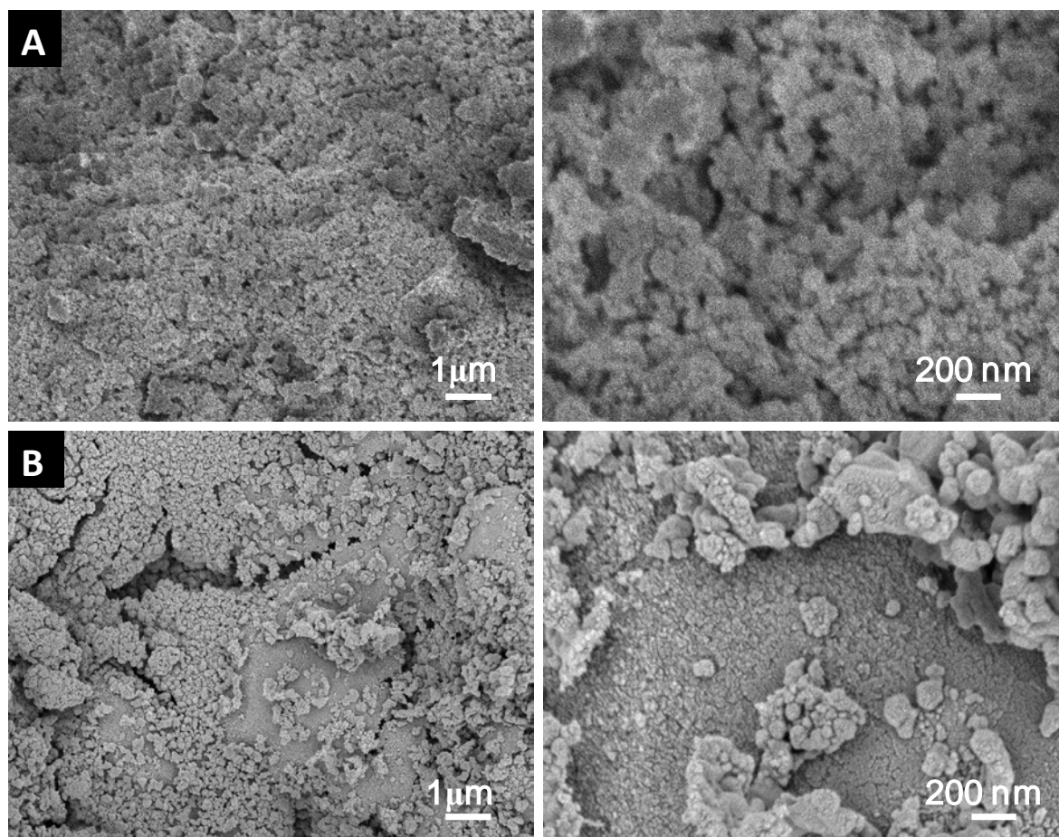
Figure 7. (A) SEM micrographs of the 10Co/SiC after reduction under H 2 at 300 °C for 6 h. (B) SEM micrographs of the 10Co/TiO 2 -SiC after reduction under H 2 at 300 °C for 6 h.
