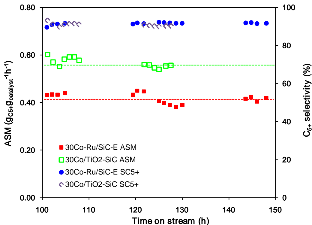
Figure 13. FTS activity and C 5+ selectivity as functions of time on stream on 30Co/TiO 2 -SiC and Co-Ru/SiC-E [20] catalysts. Reaction conditions: H 2 /CO molar ratio = 2, pure syngas, total pressure = 40 bar, GHSV (STP) = 3800 h -1 , reaction temperature = 230 °C.
