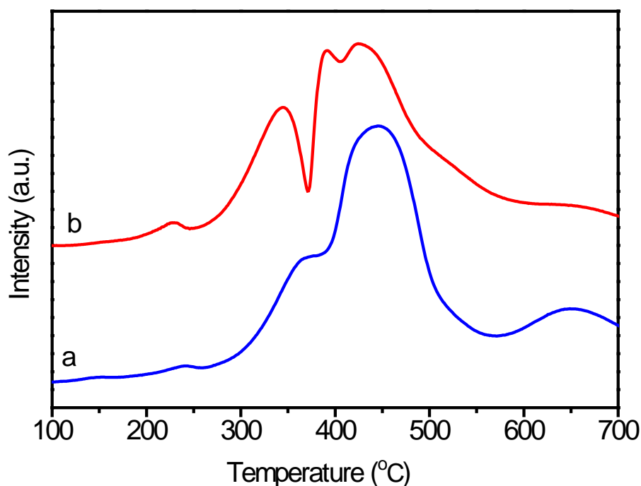
Figure 5. TPR profiles of the (a) 10\text{Co}/\text{SiC} and (b) 10\text{Co}/\text{TiO}_2\text{-SiC} catalysts after calcinations at 350 °C in air for 2 h.
