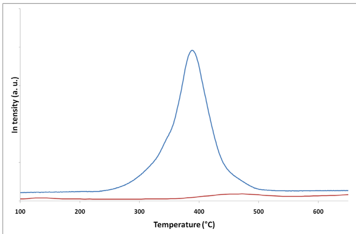
Figure 3. TPR profiles of the Co-Ru/SiC-W (H 2 O) catalysts: after calcinations at 350°C for 2 hrs (blue curve) and after reductions at 300°C for 6 hrs (red curve).
