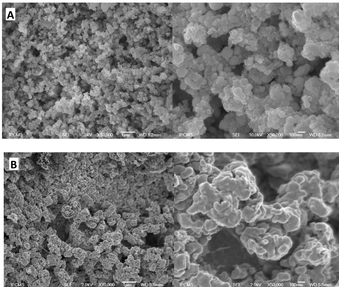
Figure 4. (A) SEM micrographs of the Co-Ru/SiC-W after reduction under H 2 at 300 °C for 6 hrs. (B) SEM micrographs of the Co-Ru/SiC-E after reduction under H 2 at 300 °C for 6 hrs.
