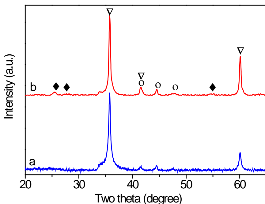
Figure 4. Ex-situ X-ray diffraction patterns of the catalysts: (a) 10Co/SiC; (b) 10Co/TiO 2 -SiC. The catalysts were calcined at 350 °C for 2 h followed by reduction under \text{H}_2 at 300 °C for 6 h. Legends: Diamond (◆): \text{TiO}_2 ; circles (○): Co; triangle (▽): SiC.
