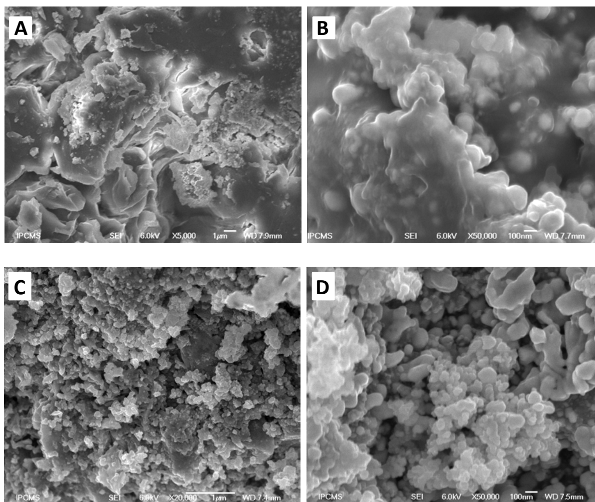
Figure 6. (A, B) SEM micrographs of the Co-Ru/SiC-E catalyst after FTS reaction showing the complete coverage of the catalyst surface by a relatively thick solid hydrocarbons film. (C, D) SEM micrographs of the Co-Ru/SiC-E catalyst after FTS reaction and wax removal at 400°C under He.
