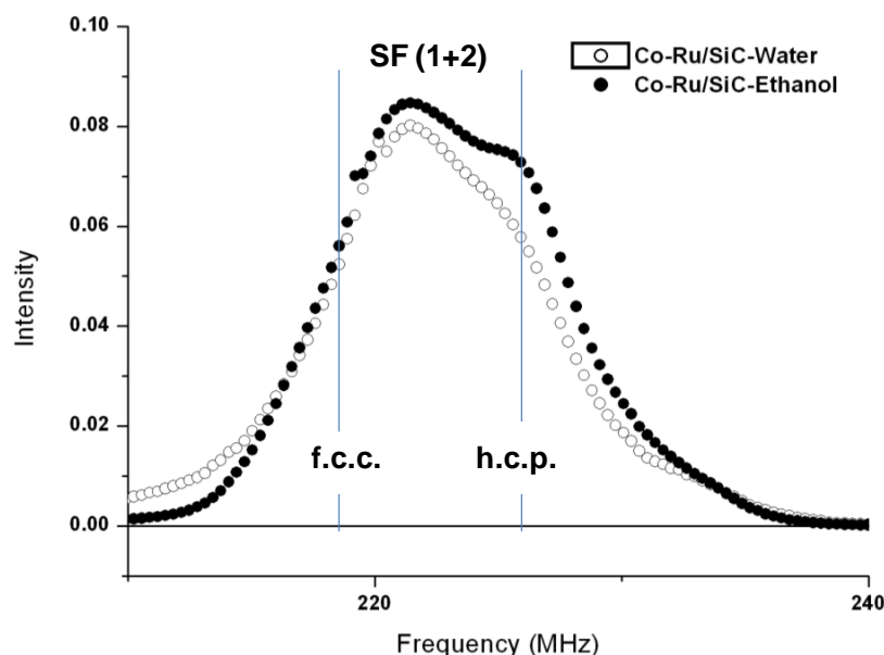
Figure 9. ^{59}\text{Co} NMR spectra of the Co-Ru/SiC-E and Co-Ru/SiC-W catalysts, recorded at 4.2 K, showing the presence of several cobalt species in the sample: Co (fcc), Co (hcp) and stacking faults (SF (1+2)). The total stacking faults (single and double faults) 56 \pm 1\% for the Co-Ru/SiC-E and 52 \pm 1\% for the Co-Ru/SiC-W respectively and is relatively high compared to the pure phases.
