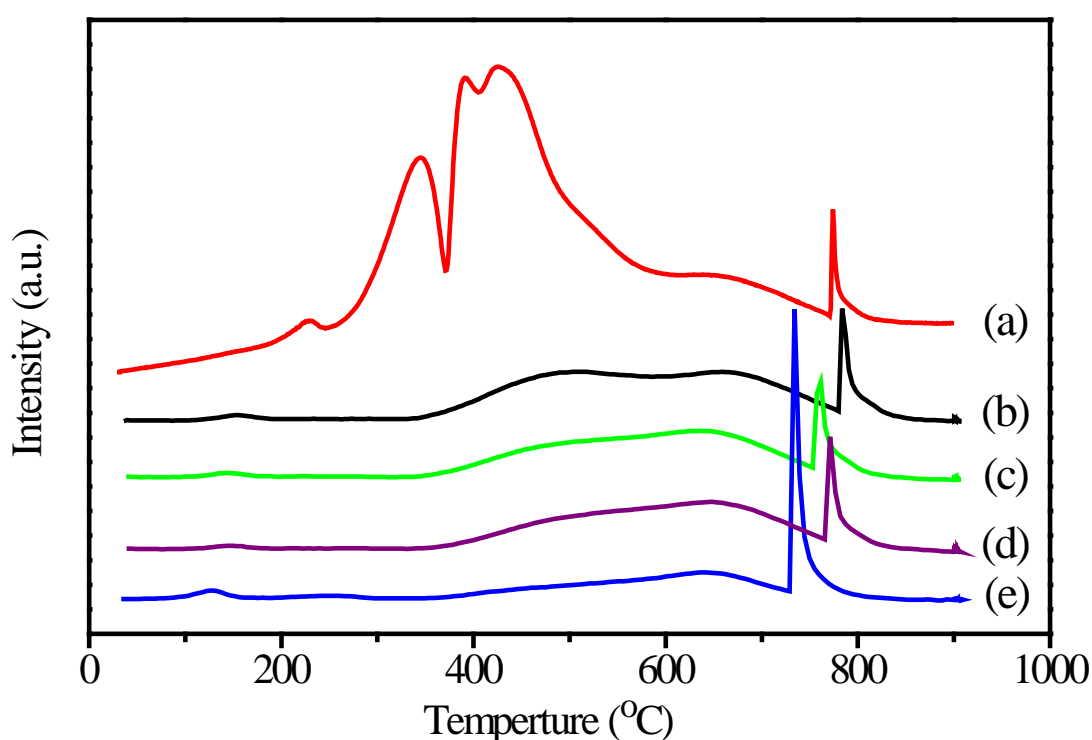
Figure 6. In-situ TPR profiles of Co 10 /TiO 2 -SiC. (a) The TPR was directly test under diluted H 2 with heating rate of 15 °C min -1 ; The sample was in-situ reduced by diluted H 2 (10 vol. % in argon) at 300 °C for (b) 2 h; (c) 3 h; (d) 4 h ; (e) 6 h in TPR equipment, and then under the diluted H 2 with a heating rate of 15 °C. min -1 .
