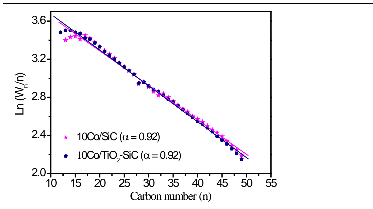
Figure 11. Calculated chain growth factor ( \alpha ) from the linear portion of the liquid hydrocarbons recovered after FTS tests on the Co/SiC and Co/TiO 2 -SiC catalysts.
