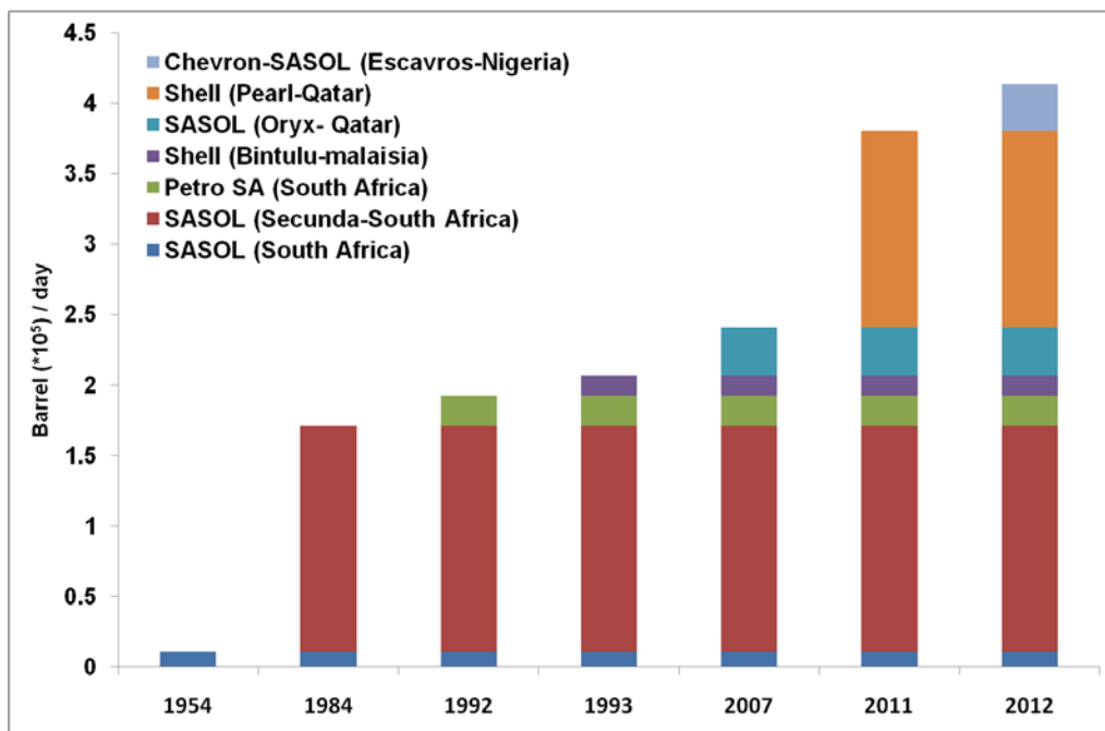
Figure 5. Industrials development of synthetic fuels based on the Fischer-Tropsch process. New FT plants with more important capacity have been developed during the last decade 2 .
