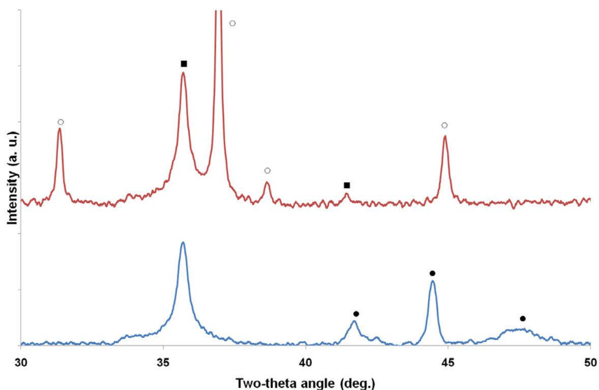
Figure 2. XRD patterns of the 30Co/SiC-HP before and after reduction under \text{H}_2 flow at 300 °C for 6 h confirming the complete reduction of the cobalt oxide phase. (■) SiC, (○) \text{Co}_3\text{O}_4 , (●) \text{Co}^0 .
