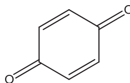
Quinone
