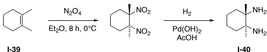
Scheme 5. Reaction of cyclic tetrasubstituted alkene with N_2O_4 .
