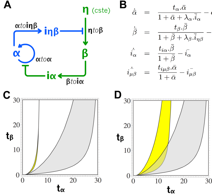
Figure 3.12: (A) Single-autocatalytic module circuit encoding bistability. (B) Non-dimensionalized equations of the simplified model. t_x are the scaled concentrations of template producing x and \lambda_x the ratio of activator over inhibitor binding constant. Periods indicate multiplications. (C) Phase diagram of the bistable circuit in the plane \{t_{\alpha}, t_{\beta}\} , with \{t_{i\alpha}, t_{i\eta\beta}\} = \{0.3, 0.3\} and \bar{\eta} = 1 . Yellow: bistable domain for \{\lambda_{\alpha}, \lambda_{\beta}\} = \{20, 20\} . Gray: bistable domain for \{\lambda_{\alpha}, \lambda_{\beta}\} = \{100, 100\} . (D) Idem with yellow: bistable domain for \{\lambda_{\alpha}, \lambda_{\beta}\} = \{50, 100\} ; and gray: bistable domain for \{\lambda_{\alpha}, \lambda_{\beta}\} = \{100, 100\} .
