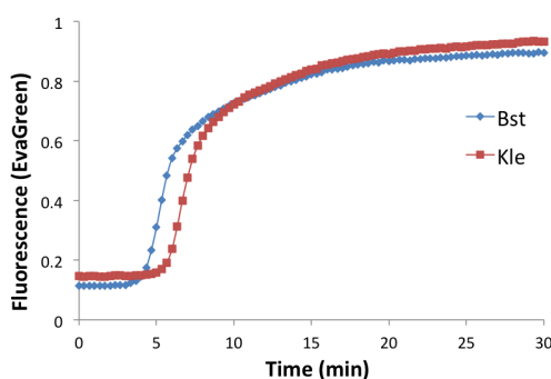
Figure B.1: Amplification of T11 in absence of exonuclease. The reaction is performed at 37 °C, with 0.08 unit/ \mu l of either Bst DNA polymerase (blue curve) or Klenow Fragment (red curve). Nicking endonuclease Nt.BstNBI was used (2 %). Autocatalytic module cT11 (60 nM) was initially put in presence of 0.1 nM of T11.
