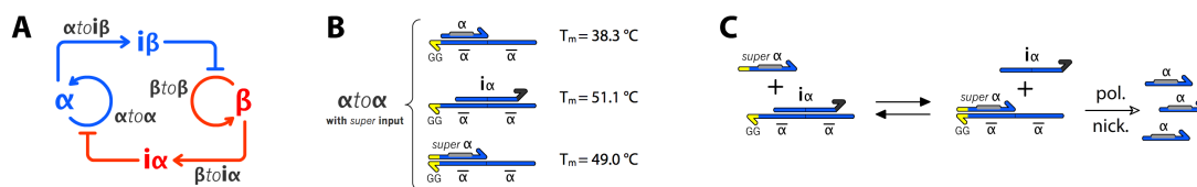
Figure 4.14: Super input principle. (A) Bistable circuit. When, for instance, on state B, \beta is autocatalytically produced and activates the production of i\alpha , that in turn inhibits \alpha to \alpha . (B) Super input enabled \alpha to \alpha has two additional G in 3'. These allow the strong binding of super \alpha , that has a T_m close to that of inhibitor i\alpha . (C) With its two additional 5' bases, super \alpha benefits from a toehold [19] of 6 bases to displace inhibitor i\alpha and subsequently re-activates autocatalytic module \alpha to \alpha .
