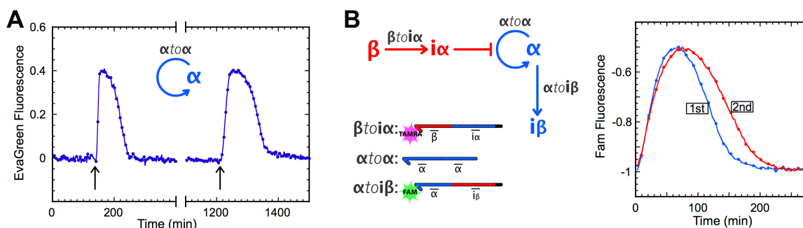
Figure 3.21: Checking the viability of the circuit over time. (A) Autocatalytic module \alpha\text{to}\alpha (20 nM) is given dNTPs (20 \mu\text{M} ) and input \alpha (1 nM) at the times marked by an arrow: first at t = 140\text{min} , then at t = 1220\text{ min} . After having consumed all dNTPs, it stops producing \alpha : fluorescence level gets back to the baseline level. Reaction is monitored with EvaGreen intercalating dye that reports on the total amount of double-stranded DNA in solution. (B) Autocatalytic module \alpha\text{to}\alpha (5 nM) is inhibited by i\alpha produced by \beta\text{to}\alpha (20nM) upon injection of \beta (80 nM). Reaction is monitored with the FAM label of \alpha\text{to}\beta (20 nM): fluorescence increases as \alpha\text{to}\alpha is inhibited. Following a first inhibition (blue curve) a second is triggered 500 minutes later (red curve).
