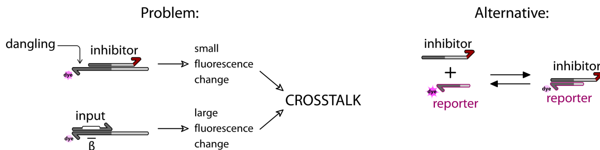
Figure 2.13: (Left) When hybridizing to its template, the input induces a larger fluorescence change than the inhibitor. For this reason, inhibitor strand cannot be directly observed. (Right) A potential solution would be to use a “reporter” of the inhibitor. The reporter is a short DNA strand with a 3'-end fluorophore, that dynamically hybridizes to the inhibitor, inducing a shift of fluorescence intensity. The reporter is designed with in mind to not disturb the circuit functioning: it is shorter than the inhibitor and possibly has mismatches, in order to lower its melting temperature.
