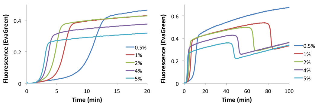
Figure B.3: Amplification of T11vi ( [c11vi] = 60 nM) in absence of exonuclease. The reaction is performed at 37 °C, with Bst DNA Polymerase, and a ramp of Nt.CviPII from 0.5 % to 5 %. Left: the first 20 minutes. Amplification speed increases as the concentration of nickase increases. Right: after a few tens of minutes, the fluorescence decreases suddenly. This happens earlier for higher concentrations of nickase.
