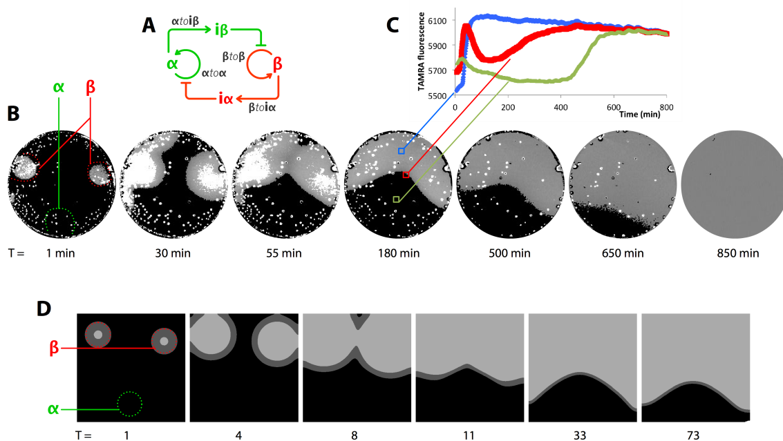
Figure C.1: Bistable circuit in 2D. (A) Bistable circuit. (B) Time-frame of the experiment monitored through Tamra channel. Fluorescence intensity was converted in three levels for visibility (dark, grey and bright). Bright corresponds to high concentration of \beta . The reaction was started with two localized spots of \beta and one of \alpha . (C) Fluorescence time-plot at three different locations. The global decrease of intensity suggests that Tamra gets bleached throughout the reaction. The experiment was run at 42 °C, with [\alpha \rightarrow \alpha] = 10 nM and [\beta \rightarrow \beta] = 20 nM.
