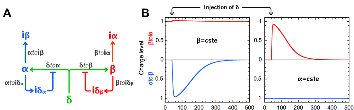
Figure 3.17: Structure and function of the injection layer for the push-push memory system. (A) Inhibition modules \alpha to i \delta_\alpha and \beta to i \delta_\beta produce respectively i \delta_\alpha and i \delta_\beta , depending on the presence of either \alpha or \beta . Inhibitors i \delta_\alpha and i \delta_\beta inhibit the activation modules \delta to \alpha and \delta to \beta . In the resulting circuit, in the presence of \alpha , \delta to \alpha is inhibited, and injection of the external input \delta will only activate \delta to \beta , hence produce \beta . Conversely, in presence of \beta , only \delta to \alpha will be sensible to external input \delta . (B) Theoretical time traces of the charge level of the templates \beta to i \alpha and \alpha to i \beta either when the constant presence of \alpha is imposed and a short pulse of \delta is applied (left), or when the constant presence of \beta is imposed and the same short pulse of \delta is applied (right).
