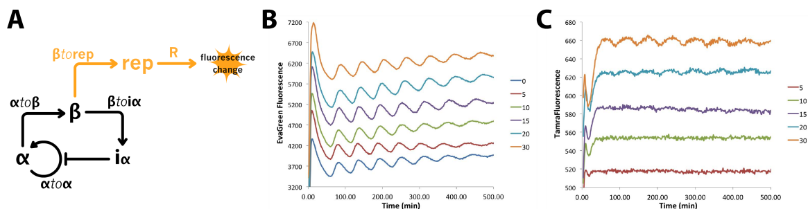
Figure 2.12: Reporting module plugged to the C11bt oligator. (A) Circuit of the oligator (in black) and plugged reporting module (in orange). (B) Fluorescence time plots of EvaGreen intercalating dye for a ramp \beta\text{torep} (0 to 30 nM) and (C) corresponding time plots of Tamra. Curves are offset for visibility. The experiment was run at 38.5 °C, with concentrations of templates as follows: \alpha\text{to}\alpha = 30 nM, \alpha\text{to}\beta = 5 nM, \beta\text{to}\alpha = 35 nM and \text{R} = 30 nM. Sequence of \text{R} is 5'-C*A*A*GTCACATGG-3'-TAMRA. Duplex \text{r}:\text{R} has a predicted (Dinamelt) T_m of 40.3 °C.
