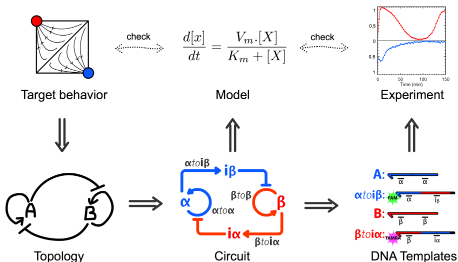
Figure 3.9: Implementation of a target behavior with the DNA-toolbox. A target behavior can correspond to one out of a number of network topologies. These topologies can in turn be translated into an assembly of modules compatible with the toolbox. A simple model of the corresponding circuit allows one to check the consistency of the chosen design with the target behavior, and find out the key parameters or conditions that the circuit must meet in order to perform as expected. The following step consists in the design of the templates that encode the activation, autocatalysis and inhibition modules of the circuit, and the experimental implementation. The experiment should be in good agreement with the simple (or more detailed) model, which can in turn be used to adjust the experimental parameters of the circuit.
