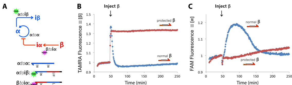
Figure 4.11: Inhibition using protected input. (A) Circuit and templates. [\alpha\alpha] = 10 nM, [\alpha\beta] = [\beta\alpha] = 30 nM. 250 nM of either “regular” \beta or protected \beta is injected to inhibit autocatalytic module \alpha\alpha . The corresponding reaction (at 42 °C) is monitored with TAMRA (B) (high fluorescence corresponds to high concentration of \beta ) and FAM (C) (low fluorescence corresponds to high concentration of \alpha ). Injection of regular \beta (blue curves) results in a spike in (B) - because injected \beta is progressively degraded by the exonuclease - and a transient inhibition of \alpha\alpha in (C). Injection of protected \beta (red curves) results in an increased fluorescence followed by a plateau in (B) - because protected \beta is not degraded by the exonuclease - and a very slow and continuous inhibition of \alpha\alpha in (C).
