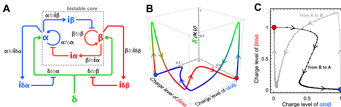
Figure 3.7: (A) Circuit of the push-push memory: a single external input \delta controls the bistable core. (B) Calculated 3D trajectories in the space {Charge level of \alpha to i\delta\alpha , Charge level of \beta to i\delta\beta , Normalized total concentration of \delta } for the push-push memory switching from A to B (blue) and B to A (red). Normalized values of \delta (injected as a gaussian spike) from 0 to 1 are associated to a color gradient from blue/red to green. (C) Experimental trajectories of the push-push memory circuit showing two independent experiments: one where the system is initially set on the state A, then flipped to B upon injection of 30 nM of \delta , and another where the same system is set in state B, then flipped to A upon injection of the same input. The charge level of \beta to i\delta\beta higher than 1 indicates that the amount of \beta transiently produced by activation module \delta to \beta during switching exceeds the concentration of \beta at the stable state B.
