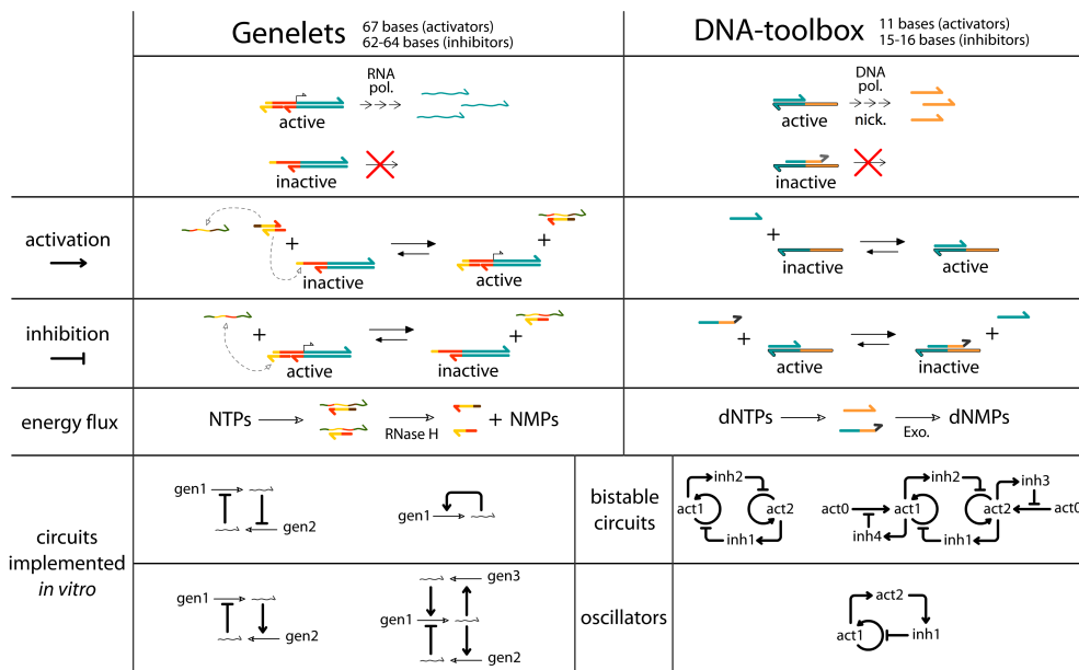
Figure 2: Two systems allowing the rational assembly of dynamic reaction circuits from basic units. Genelets are double-stranded DNA that contain a nicked promoter (in red). When the promoter is complete (genelet indicated as “active”), a RNA polymerase transcribes it in RNA transcripts (thin wavy strands) that establish the communication between genelets. “Activation” is obtained when the sequestered DNA activator of an inactive genelet is released by an activating RNA transcript. “Inhibition” is obtained as an inhibiting RNA transcript binds and displaces the DNA activator of an active genelet, thus inactivating it. A RNase degrades RNA transcripts into NMPs. In the DNA-toolbox, short DNA activators activate DNA templates (bottom strands) that consequently produce other DNA activators or inhibitors and establish the communication between templates. “Activation” is obtained as a DNA activator hybridizes to a DNA template and primes polymerization. “Inhibition” is obtained as a DNA inhibitor hybridizes to a template, thus blocking activators. An exonuclease degrades DNA activators and inhibitors into dNMPs. Both systems led to experimental implementations of various dynamic circuits encoding oscillations and bistability.
