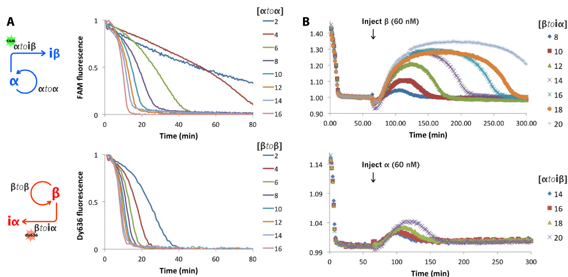
Figure 4.12: Balancing a bistable circuit. Here, we use a different \beta : 5'-CAGAGTCCAAG-3' which produces a negative fluorescence change as it hybridizes on the dy636-modified \beta to \alpha . (A) Charge of inhibition modules (20 nM) \alpha to \beta (up) or \beta to \alpha (down) by respectively \alpha to \alpha or \beta to \beta (ramp of concentration from 2 to 16 nM). In this system, 12 nM of \alpha to \alpha seems to charge \alpha to \beta in the same amount of time as 6 nM of \beta to \beta charges \beta to \alpha . (B) Inhibition of \alpha to \alpha (12 nM, up) or \beta to \beta (6 nM, down) by a ramp of concentration (from 8 to 20 nM) of the opposite inhibition module (respectively \beta to \alpha and \alpha to \beta ). Here, 10 nM of \beta to \alpha inhibits \alpha to \alpha for the same time as 20 nM of \alpha to \beta inhibits \beta to \beta . The concentrations to assemble this bistable circuit should then be [\alpha to \alpha] = 12 nM, [\beta to \beta] = 6 nM, [\alpha to \beta] = 20 nM and [\beta to \alpha] = 10 nM. Reaction were performed at 43 °C, and started with 1 nM of input (either \alpha or \beta )
