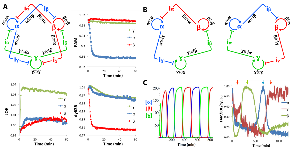
Figure 4.24: Tristability and three-switch oscillator. (A) Tristable circuit. Templates \alpha\text{toi}\beta and \alpha\text{toi}\gamma are labeled with FAM to monitor \alpha (negative fluorescence intensity shift upon charge); \beta\text{toi}\alpha and \beta\text{toi}\gamma are labeled with dy636 to monitor \beta (negative fluorescence intensity shift upon charge); \gamma\text{toi}\alpha and \gamma\text{toi}\beta are labeled with JOE to monitor \gamma (positive fluorescence intensity shift). The system initiated with 1 nM of either \alpha , \beta or \gamma stabilizes in each corresponding state A, B or C, characterized by a shift of fluorescence intensity of, respectively, FAM, dy636 or JOE, as one can observe in the fluorescence time plots of each dye. Concentrations are: [\alpha\text{to}\alpha] = [\beta\text{to}\beta] = 15 nM, [\gamma\text{to}\gamma] = 10 nM, all inhibition modules at 20 nM. (B) Three-switch oscillators oscillating counterclockwise (left) and clockwise (right). (C) Left: model (concentration of free \alpha (blue), \beta (red) or \gamma (green)) for perfectly equilibrated sequences all present in a 20 nM concentration. Right: experimental fluorescence (normalized, and reversed for FAM and JOE whose fluorescence change upon hybridization is negative) time plot for a system with [\alpha\text{to}\alpha] = 20 nM, [\beta\text{to}\beta] = 5 nM, [\gamma\text{to}\gamma] = 5 nM, [\alpha\text{toi}\beta] = 10 nM, [\beta\text{toi}\gamma] = 7.5 nM and [\gamma\text{toi}\alpha] = 5 nM. This latter concentration explain the poor signal induced by \gamma . The reaction was initiated with [\gamma] = 5 nM and [\alpha] = [\beta] = 1 nM. Colored arrows indicate the successive spikes of input species: first comes a spike of \gamma , then \beta , then \alpha , after which \gamma reactivates and the system stalls forever. Sequences are as follows: \alpha : CTGAGTCTTGG, \beta : CAGAGTCCAAG, \gamma : AGGAGTCACAC.
