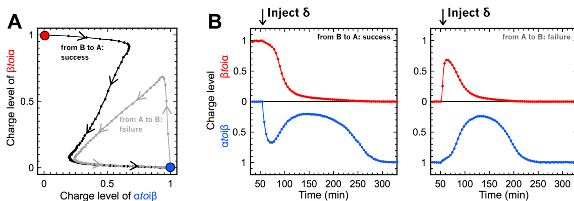
Figure 3.18: Experimental trajectories (A) and time plots (B) of the push-push memory circuit with \delta to \alpha = \delta to \beta = 5 nM and \alpha to i \delta_\alpha = \beta to i \delta_\beta = 4 nM. Upon addition of 30nM of \delta , the circuit switched from B to A, but failed to switch from A to B.
