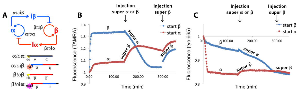
Figure 4.17: Flipping the switch with super input. (A) Bistable circuit and templates: \alpha has two G (and \beta two C) in 3' to receive its super input. Fluorescence of TAMRA (B) and ty665 (C), respectively monitoring \beta (high fluorescence corresponds to high [\beta] ) and \alpha (low fluorescence corresponds to high [\alpha] ). The same reaction mix is initiated with either \alpha (red curve) or \beta (blue curve). At t = 150 min, an injection of 30 nM of either super \alpha or \beta triggers the switching process. The system initially in state B (blue curve) flips to the A state: fluorescence of TAMRA decreases (inhibition of \beta \rightarrow \beta ), that of ty665 also decreases (reactivation of \alpha \rightarrow \alpha ). However, the system initially in state A (red curve) doesn't flip to state B, but seems to end up in an alternate state where both \alpha \rightarrow \alpha and \beta \rightarrow \beta are partially active. At t = 300 min, an injection of super \beta confirms that the system is not responsive anymore.
