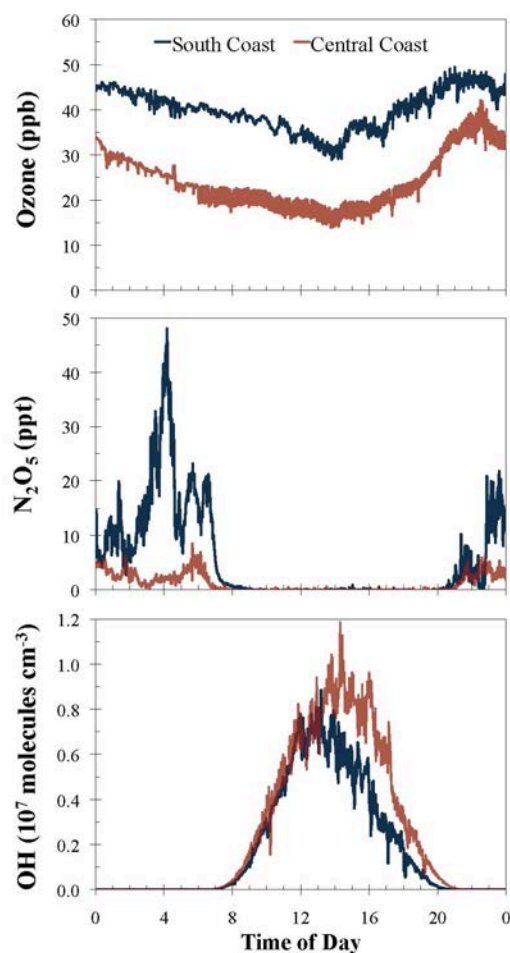
FIGURE 4.6 - Diurnally averaged mixing ratios of ozone ( upper ) and N_2O_5 ( middle ) during the South and Central coast segments of the cruise. Also shown is the diurnally averaged OH concentration ( lower ), which has been calculated from spectral radiometer measurements of the photolysis rate coefficient of ozone to produce O(^1D) using the parameterization developed by Ehhalt and Rohrer (2000), which is not strictly valid for application to the coastal MBL, but should produce estimates within \pm 30\% of more sophisticated model calculations (Sommariva et al., 2009).
