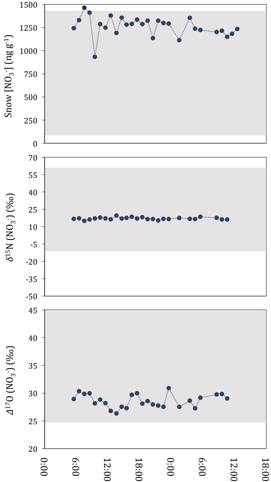
FIGURE 5.4 - Hourly variations in skin layer nitrate concentration ( upper panel ), \delta^{15}\text{N} ( center panel ), and \Delta^{17}\text{O} ( lower panel ) at Dome C during the period 28 - 29 December 2009. The shaded areas represent the measured ranges observed for the entire 2009 - 2010 time series. The analytical uncertainty for each measurement is smaller than the size of the symbols.
