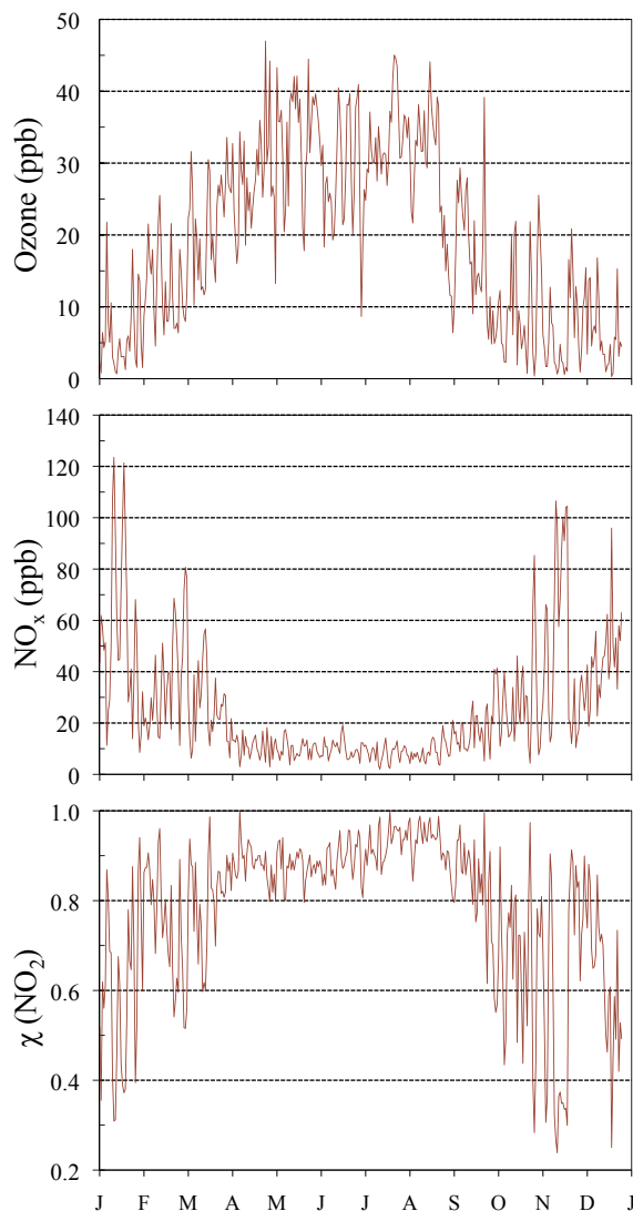
FIGURE 3.2 - 24-hour average mixing ratios of ozone (top) and \text{NO}_x (center) in Grenoble during the 2012 filter sampling campaign. The \text{NO}_2 molar ratio ( \chi_{\text{NO}_2} = \text{NO}_2/\text{NO}_x ) is shown in the bottom panel. Data has been obtained from the local air quality monitoring agency ( http://www.air-rhonealpes.fr ).
