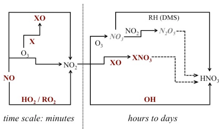
FIGURE 4.1 - \text{NO}_x reactions leading to the formation of nitrate in the atmosphere. Nitrate precursor gases associated with daytime and nighttime pathways are indicated by bold and italicized text, respectively. Dashed lines indicate heterogeneous surface reactions on atmospheric particles.
