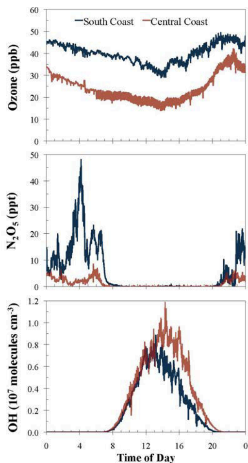
FIGURE 4.6 - Diurnally averaged mixing ratios of ozone ( upper ) and N_2O_5 ( middle ) during the South and Central coast segments of the cruise.
