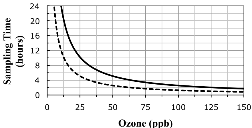
FIGURE 6.1 - Required sampling durations for the collection of 0.5 \mu\text{mol} (broken line) to 1.0 \mu\text{mol} (solid line) of nitrate for various ozone mixing ratios. Sampling time is estimated assuming a flow rate of 3.0 \text{ L min}^{-1} and the overall ozone collection efficiency reported in Chapter 2 (58%).
