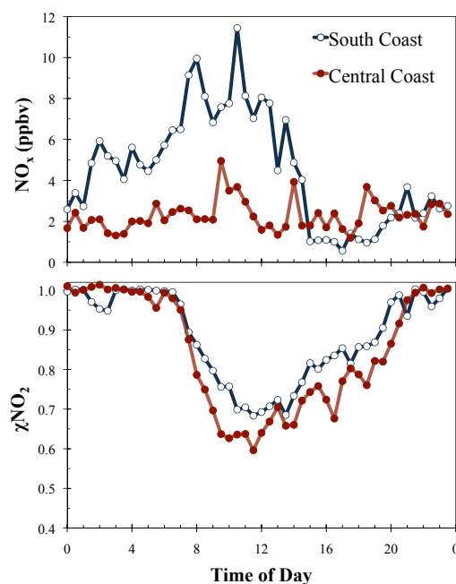
FIGURE 4.5 - Diurnally averaged values for total \text{NO}_x concentration and \text{NO}_2 molar ratio ( \chi_{\text{NO}_2} = [\text{NO}_2] / ([\text{NO}] + [\text{NO}_2]) ) during the two major segments of the cruise on R/V Atlantis . The values shown were computed from 30-minute averages of the NO and \text{NO}_2 concentration measurements conducted onboard.
