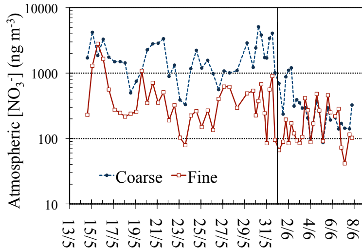
FIGURE 4.3 - Temporal variability in the atmospheric concentration of nitrate in the coarse (supermicron) and fine (submicron) particle fractions. The solid black line indicates the period of transit between the South and the Central Coast regions (1 June).
