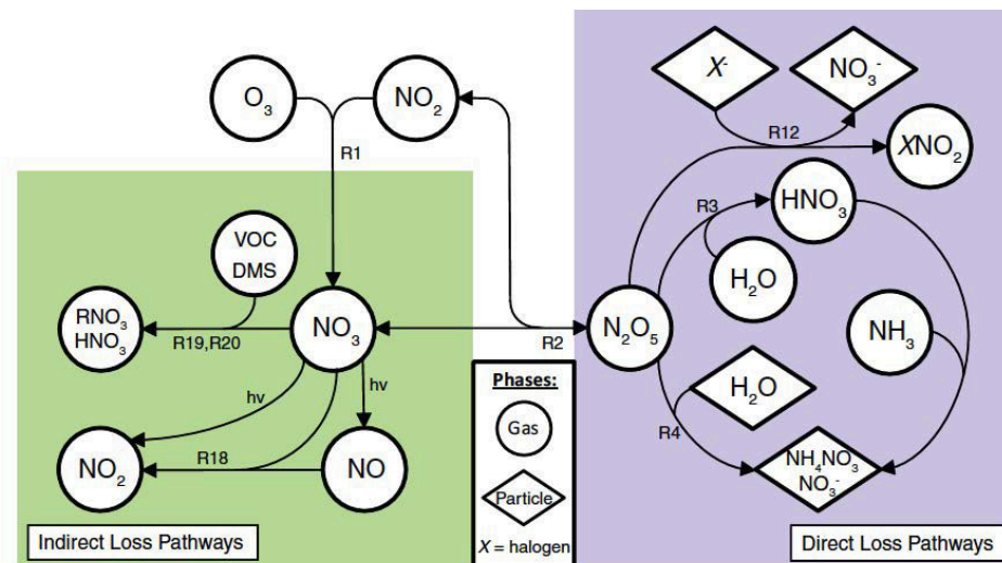
FIGURE 1.14 - Chemical mechanism for N_2O_5 formation and loss. X indicates halogen atoms such as chlorine and bromine that are commonly found in sea-salt aerosol. Circles denote gas-phase species, and diamonds denote species in particle phase (Chang et al. , 2011).
