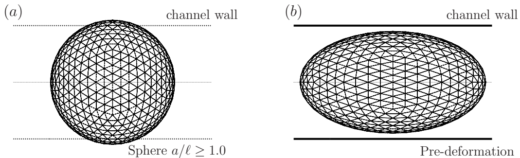
Figure 2.8: Schematic of pre-deformation for large capsules. (a) Large capsule of size ratio a/l \geq 1.0 ; (b) A large spherical capsule is pre-deformed into a spheroid to fit inside the channel.
