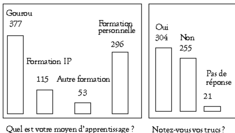
FIG. 2.9 – Formation.
