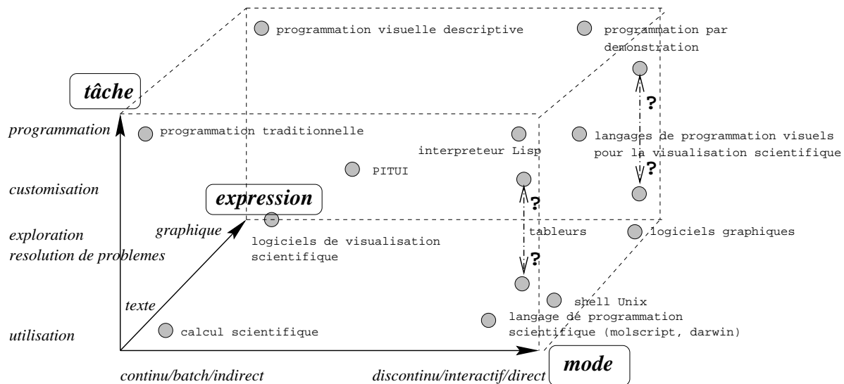
FIG. 1.3 – Axes programmation-interaction.
