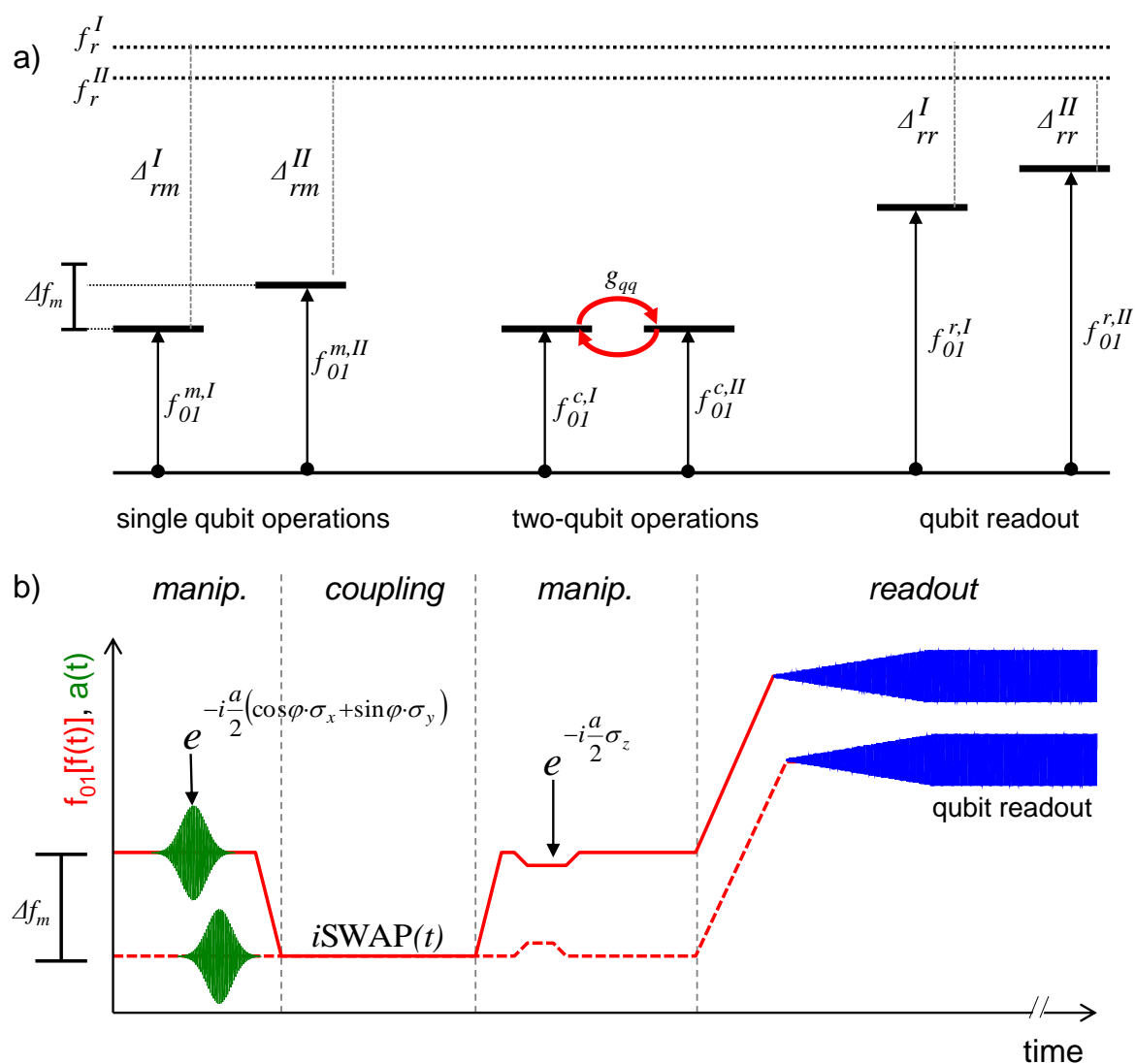
Figure 3.2: Operation principle of the two-qubit processor. a) Frequencies of qubits I and II during the different operations: single-qubit manipulation or parking (index m ), two-qubit resonant coupling (index c ), and qubit readout (index r ). the readout resonator frequencies f_r^{I,II} are also indicated. The smaller the detuning between qubits (resp. between a qubit and its readout), the larger the corresponding coupling 2g (resp. \chi_r^{I,II} ). b) Typical gate sequence consisting of two single-qubit XY-gates, a two-qubit i SWAP( t ) gate, two single-qubit Z-gates, and qubit readout.
