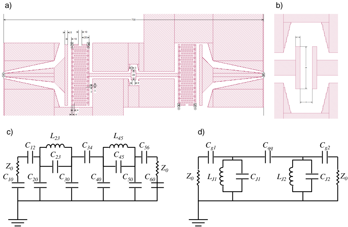
Figure 3.9: a) Schematic of the simulated chip geometry, showing the two coupled Transmon capacitances and the couplings to the readout resonators. b) Detailed view of the qubit coupling capacitance. c) SONNET generated equivalent model of the simulated geometry. d) Equivalent coupled Transmon circuit model. For the geometry shown, the obtained circuit parameters are C_{g1} = C_{g2} = 13.8 fF, C_{qq} = 0.13 fF, C_{J1} = C_{J2} = 52.2 fF, L_{J1} = L_{J2} = 5.7 nH.
