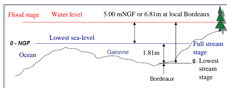
Figure D-12 Two ways of measuring water levels: NGF and local river level
