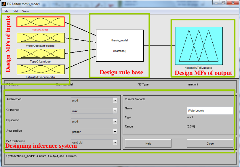
Figure III-33 Interface of the FIS Editor in the Matlab Fuzzy Logic Toolbox™
