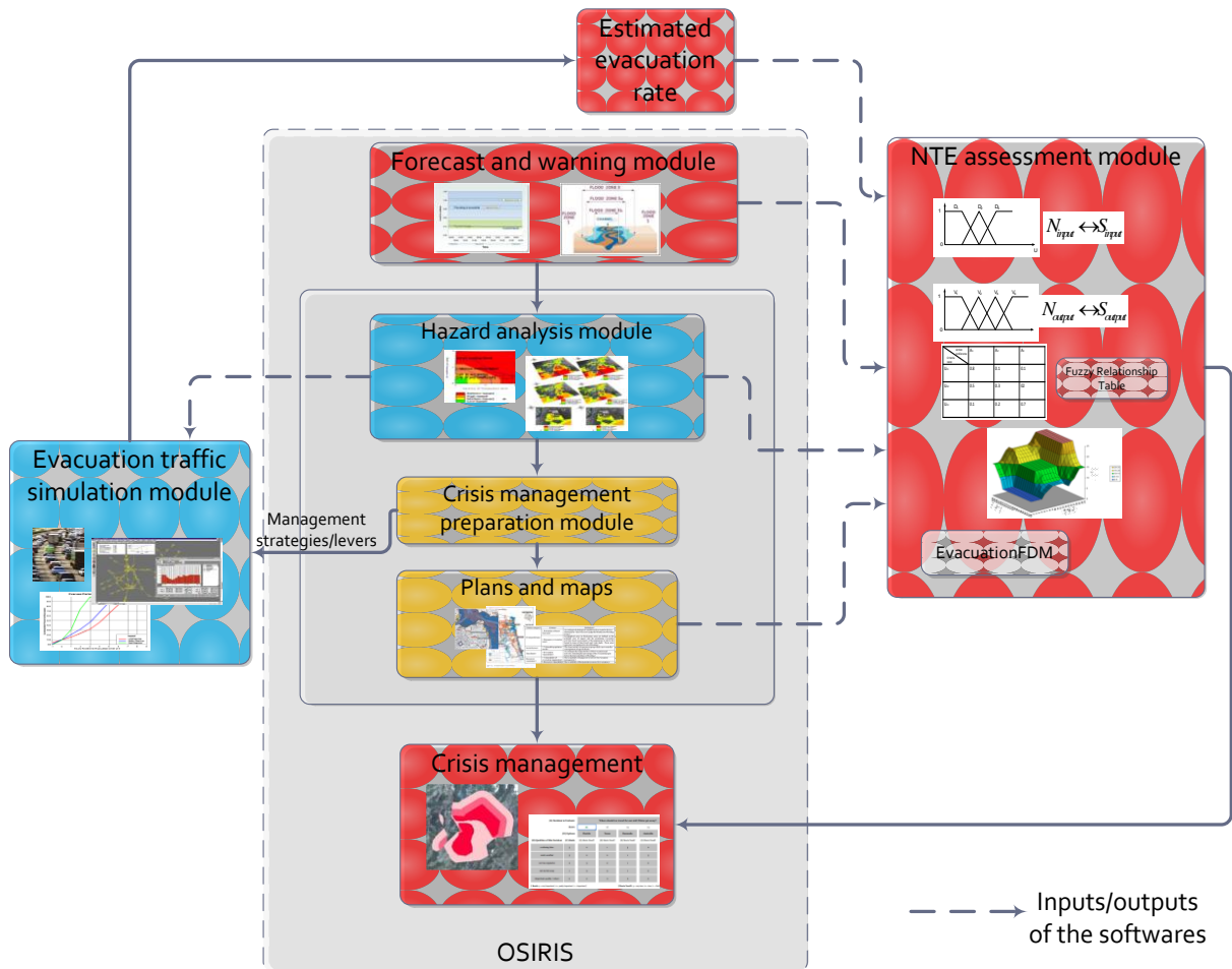
Figure V-1 A schematic view of an evacuation fuzzy decision module integrated into the OSIRIS platform
