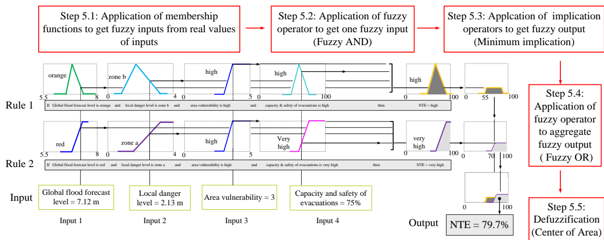
Figure III-26 Overview of the steps of the fuzzy inference system
