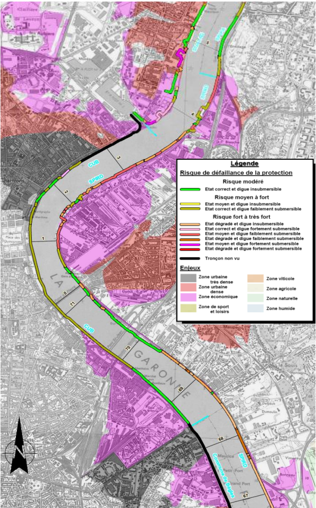
Figure D-11 River-embankment breach risk in Bordeaux Areas (source: SOGREAH 2009c)
