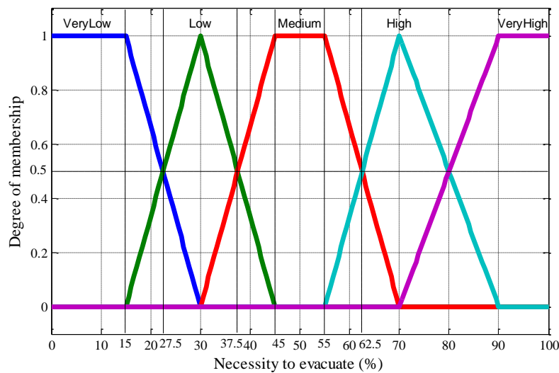
Figure III-24 Membership Functions for the necessity to evacuate (NTE)
