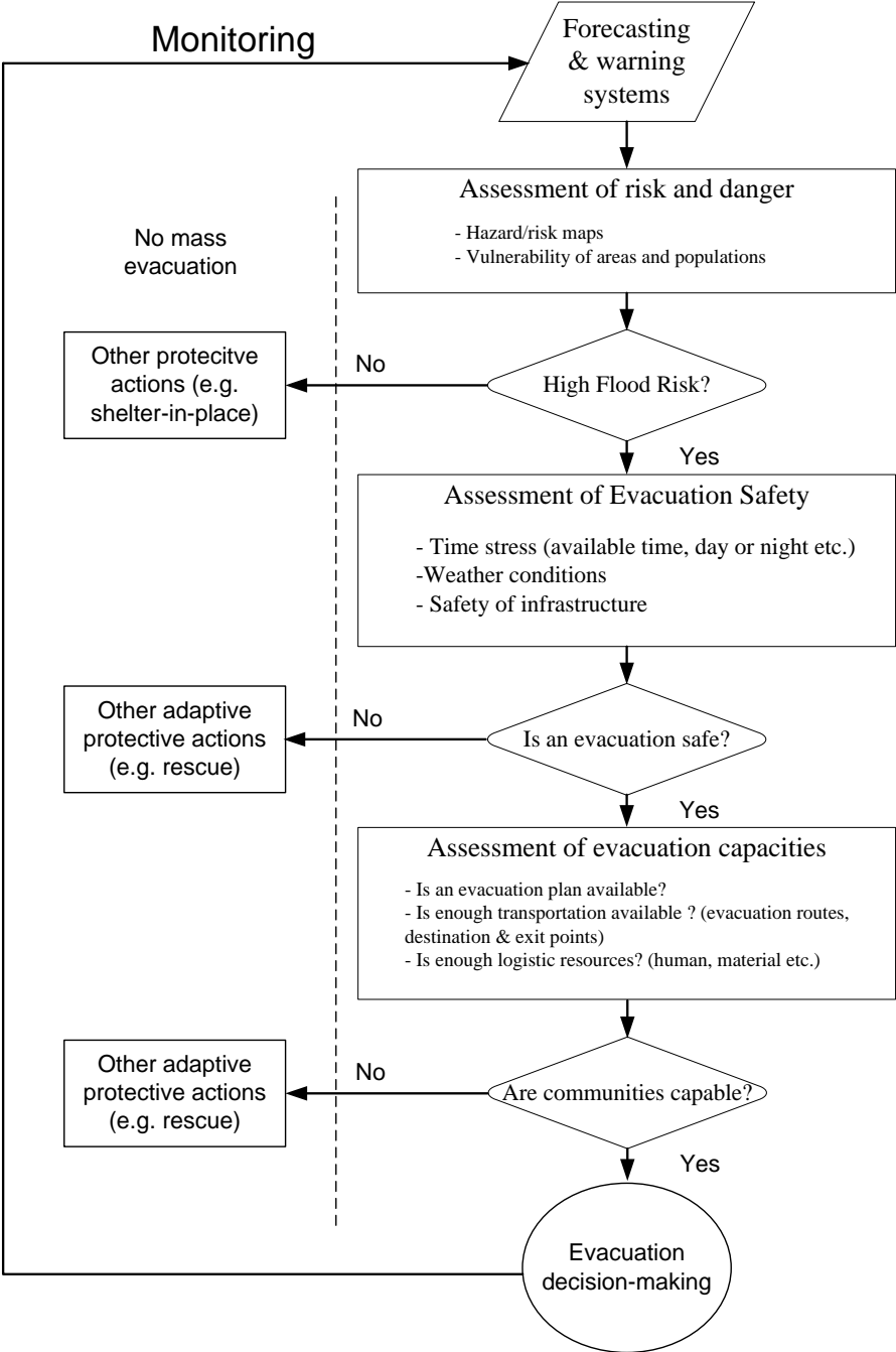
Figure III-1 Evacuation decision-making process and critical relevant factors
