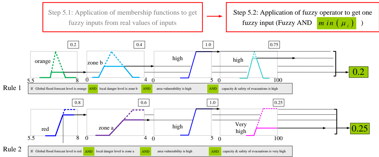
Figure III-29 Examples of combining fuzzy inputs to get a single input, using the fuzzy AND operator
