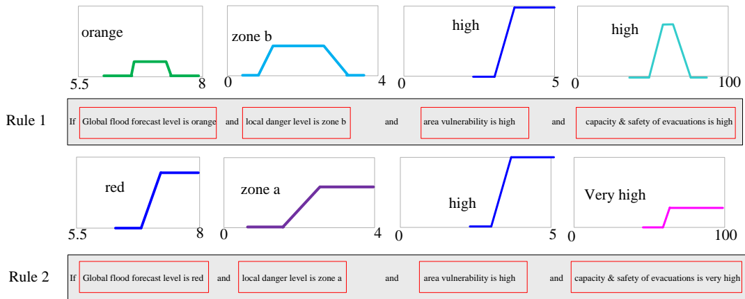
Figure III-28 Results of the fuzzification first step applied to 2 rules
