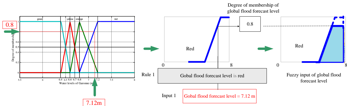
Figure III-27 Example of fuzzifying the initial value of the global forecast criteria
