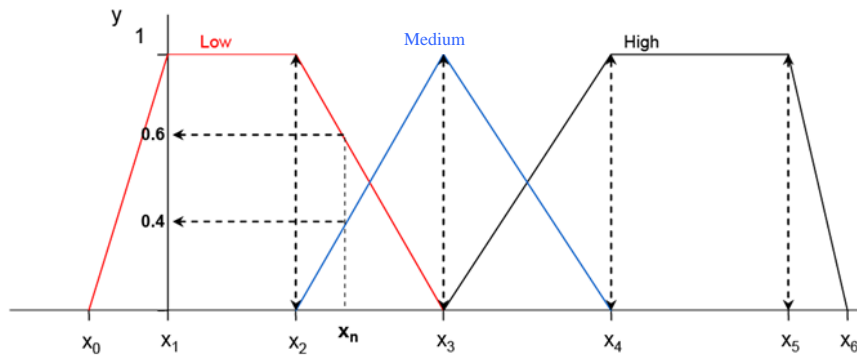
Figure III-12 Example of the three MFs for a given input
