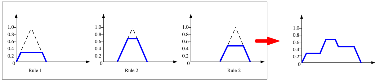
Figure III-13 Example of aggregated fuzzy outputs with fuzzy maximum operator
