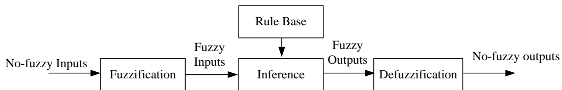
Figure III-11 General structure of a ruled-based fuzzy logic system
