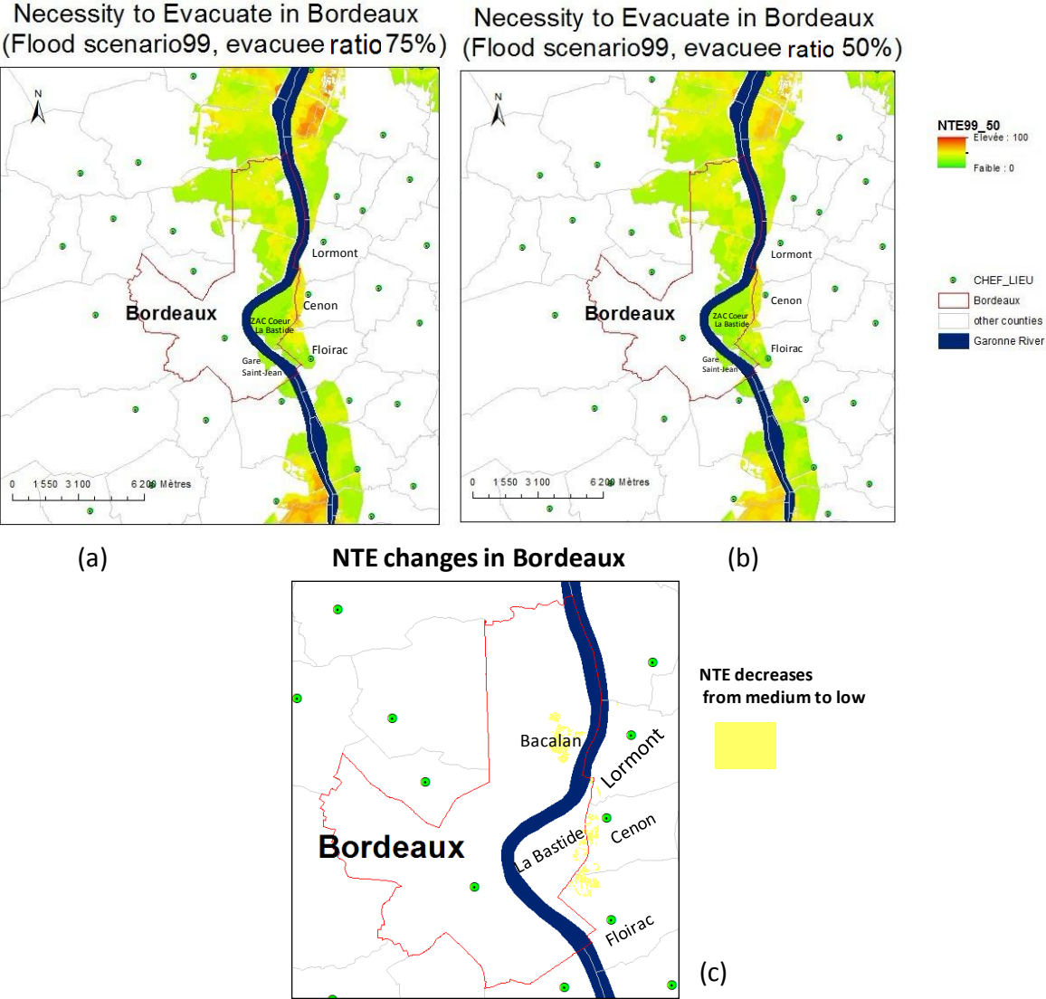
Figure IV-9 Comparison of the NTE for the 1999 scenario with 50% and 75% of evacuee ratio
