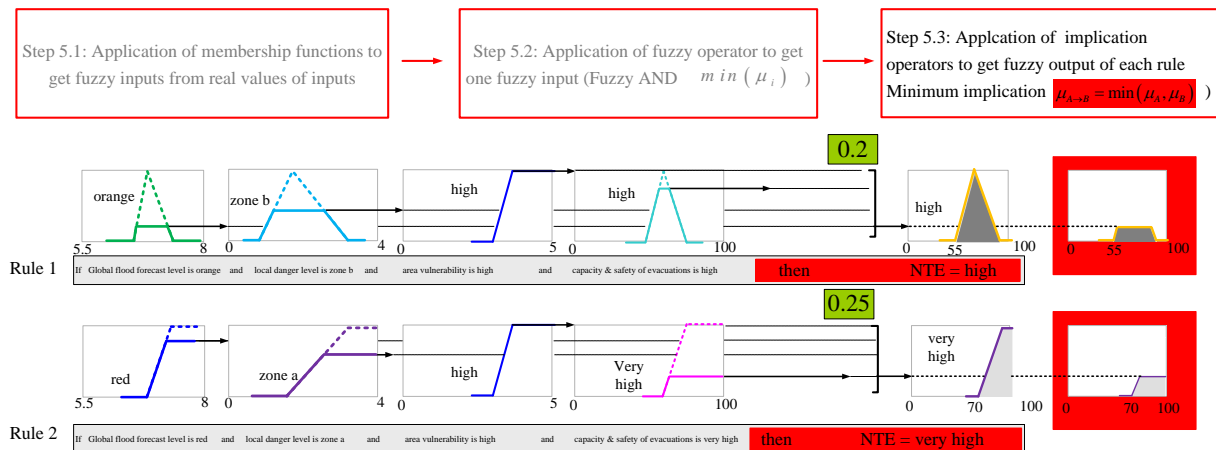
Figure III-30 Example of applying minimum implication operator to get fuzzy outputs
