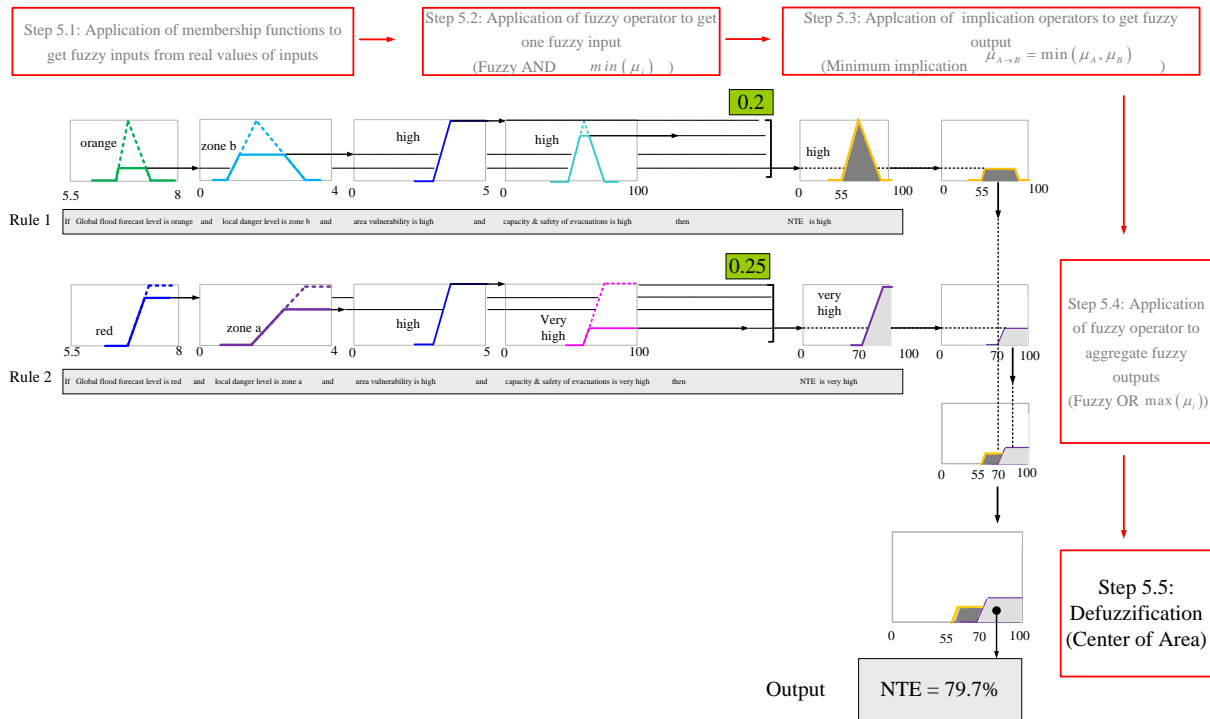
Figure III-32 Example of applying defuzzification methods to get the final value of the NTE
