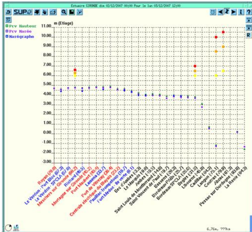
Figure III-16 Example of forecasted water levels in the Gironde estuary (Sarralde, 2010)
