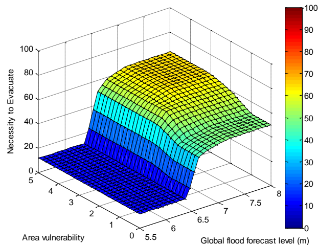
Figure III-38 Fuzzy surfaces of NTE varying with the global forecasted level and the area vulnerability
