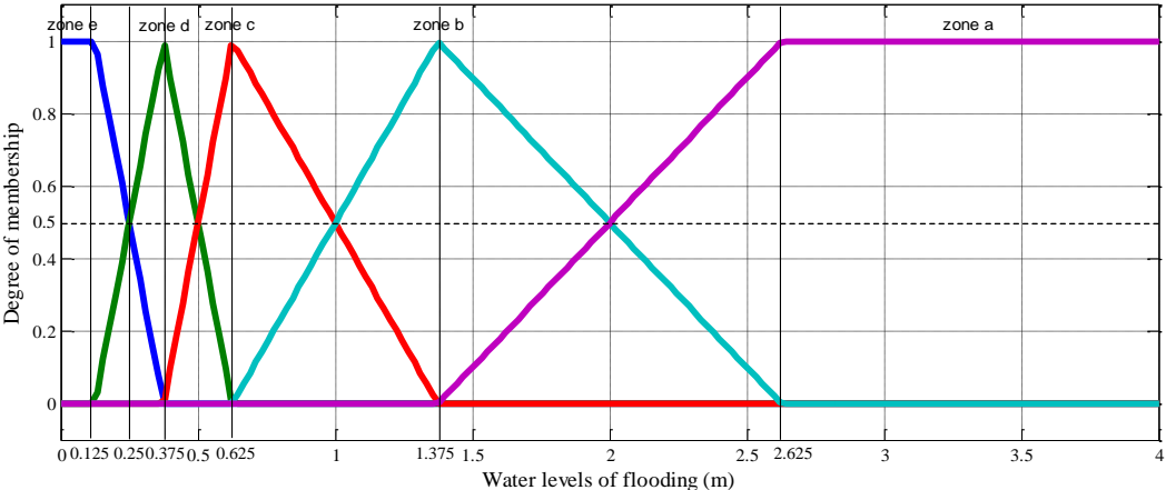
Figure III-21 Membership functions for the local danger level
