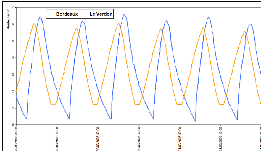
Figure D-19 Example of local water levels data at Bordeaux, with the tide cycle
