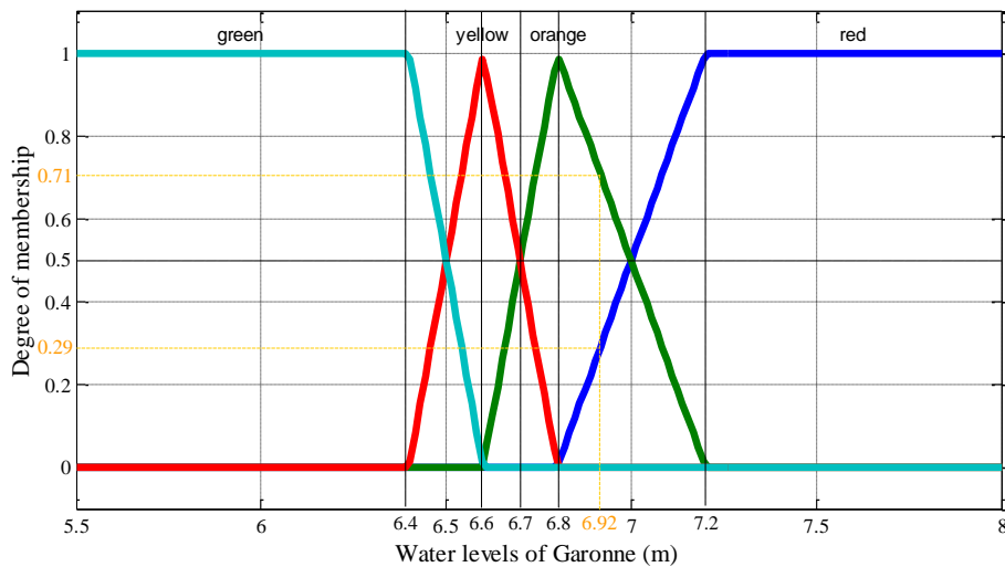
Figure III-20 Membership functions for the global flood forecast level
