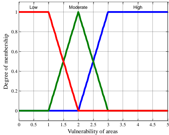
Figure III-22 Membership functions for vulnerability of areas
