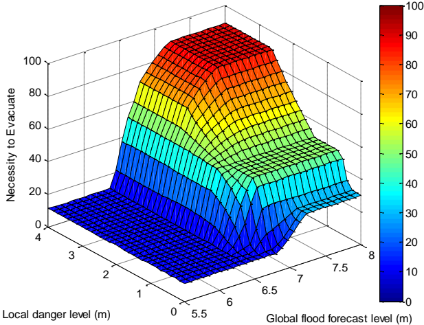
Figure III-35 Fuzzy surface of NTE varying with the global forecasted level and the local danger level
