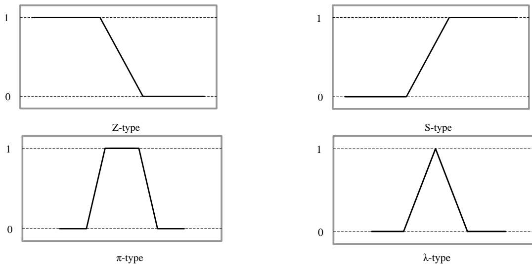
Figure III-8 Four basic membership functions shapes
