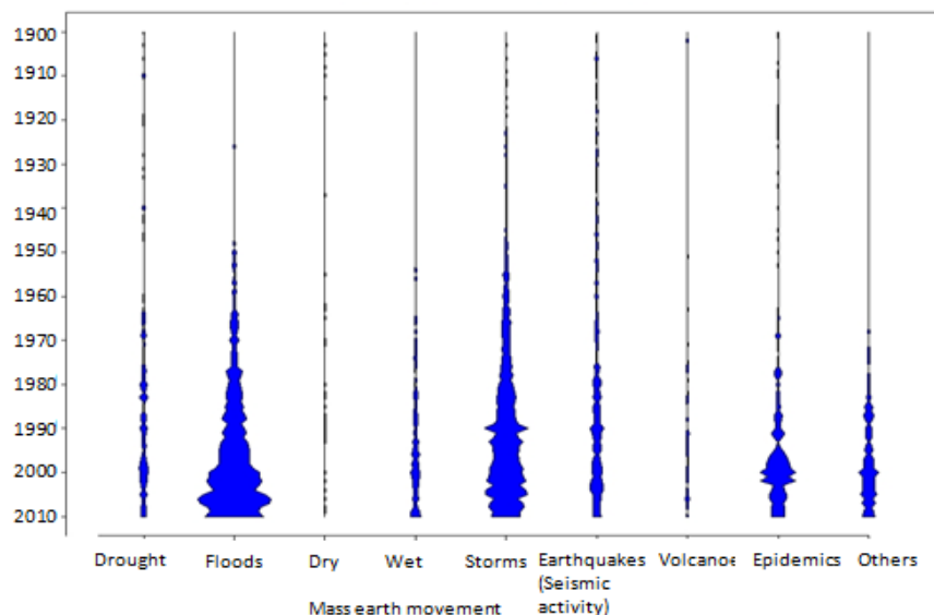
Figure I-3 Number of natural disaster reported 1900-2010 (EM-DAT: the OFDA/CRED - International Disaster Database- http://www.emdat.be/ - Université Catholique de LOUVAIN, Brussels-Belgium)
