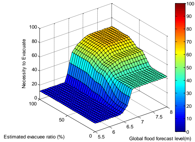
Figure III-37 Fuzzy surfaces of NTE varying with the global forecasted level and the Evacuee ratio
