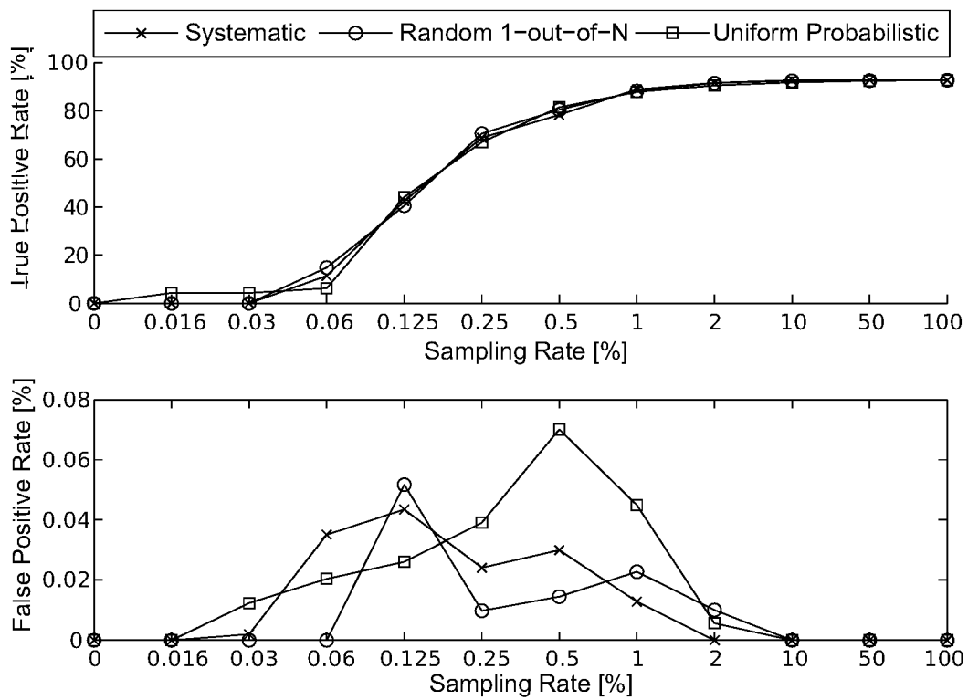
Figure 6.7: TPR and FPR—the influence of three sampling methods on the proposed scheme based on analyzing SYN-ACK segments in the case of host scan activity.
