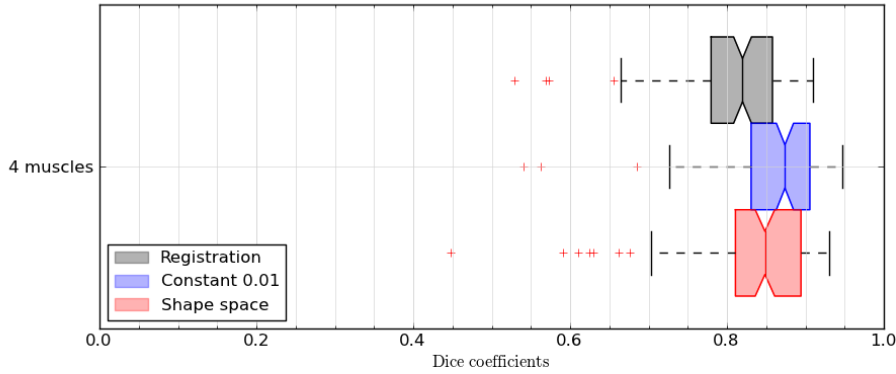
Figure 4.4.1 – Comparison of our RW with shape space method (bottom box) with the simpler RW with prior method with constant weighting (middle box, see section 4.3) and the registration-based baseline method (top box, see section 4.3.4).
