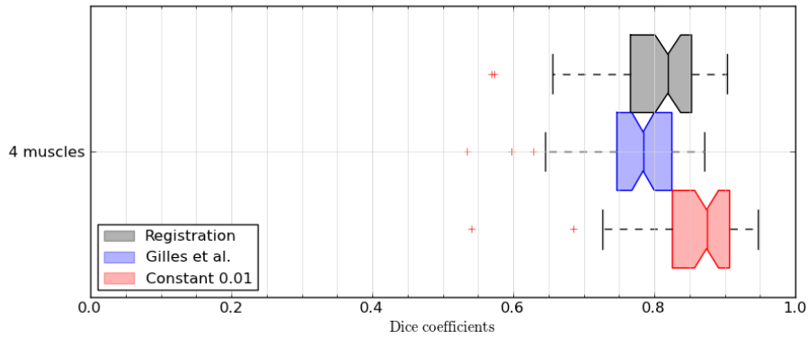
Figure 4.3.9 – Comparison of our method (bottom box) with the “registration” method (top box) and the method from (Gilles and Pai, 2008) (middle box). Dataset : subset of the 4-muscle dataset with only 15 test volumes.
