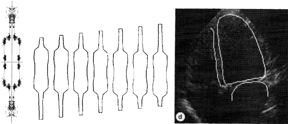
Figure 2.1.7 – Active Shape Model: (left): scatter plot of the landmarks of the training examples ( Cootes et al., 1995 ); (middle) synthesized models using: \mathbf{x} = \bar{\mathbf{x}} + \mathbf{U}\mathbf{p} for different values of \mathbf{p} [0] ( ibid ); (right) segmentation of a heart ventricle in an echo-cardiogram using ASM ( ibid ).
