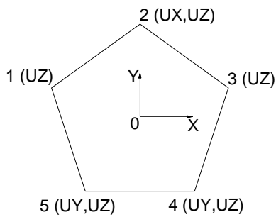
Figure 3.34. Conditions aux limites
