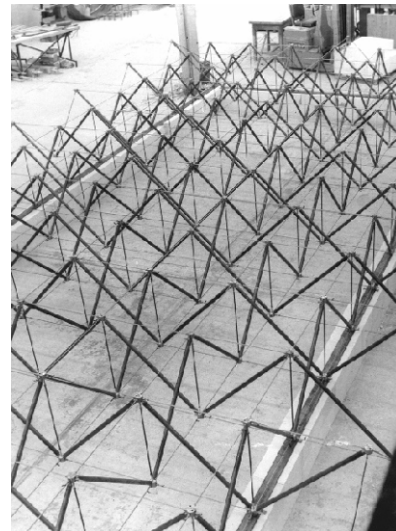
Figure 2.26. Tensarch
