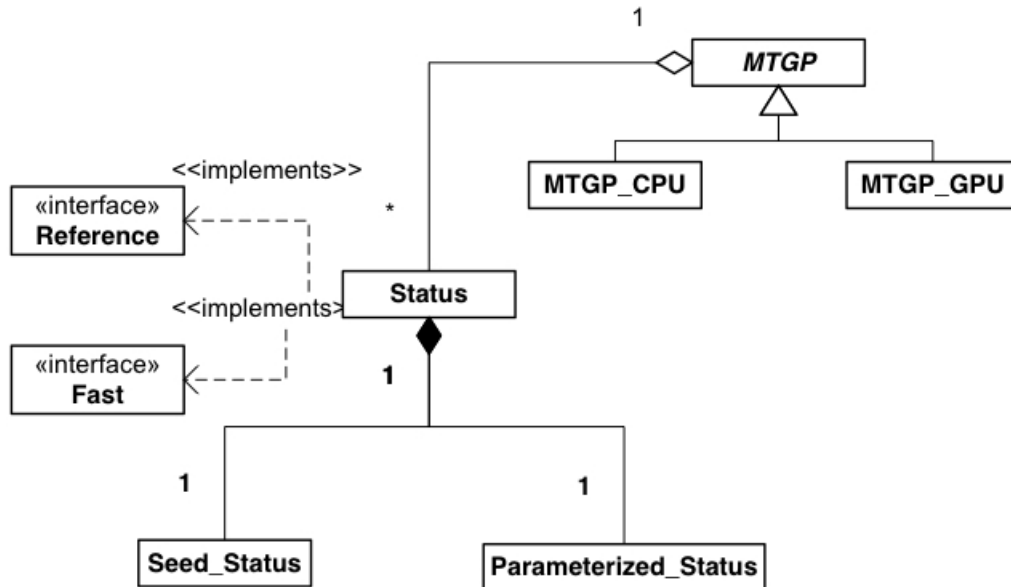
Figure 2.6: Class Diagram for MTGP and its components
