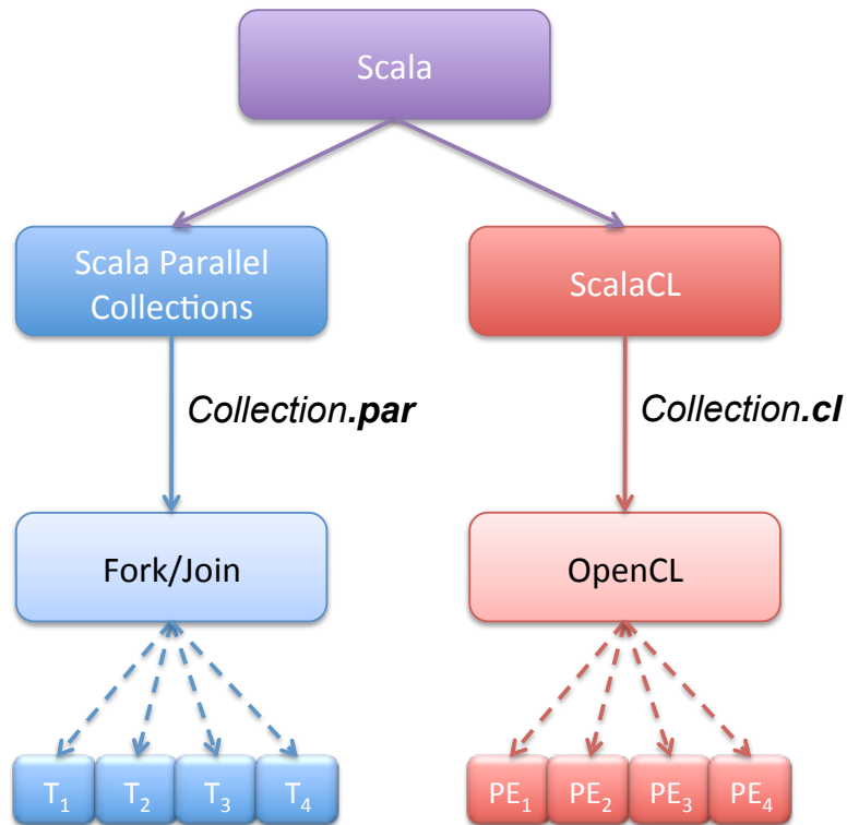
Figure 6.3: Schema showing the similarities between the two approaches: Scala Parallel Collections spread the workload among CPU threads (T), while ScalaCL spreads it among OpenCL Processing Elements (PEs)
