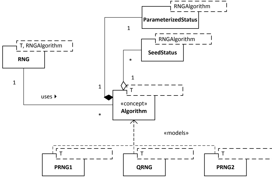
Figure 4.2: Meta-Model Describing the ShoveRand Framework
