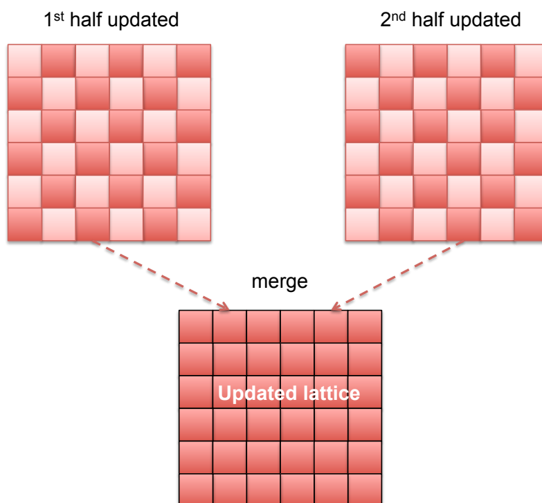
Figure 6.4: Lattice updated in two times following a checkerboard approach
