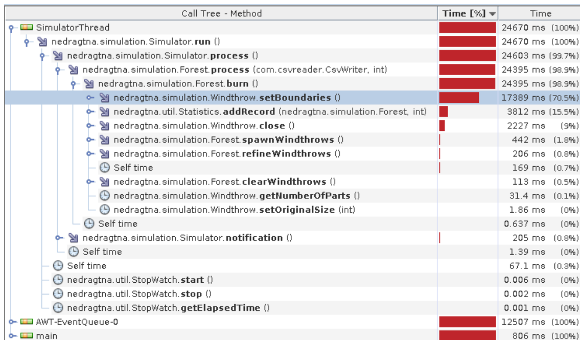
Figure 6.1: Output of the Netbeans Profiler after 200 iterations of the sequential Gap Model
