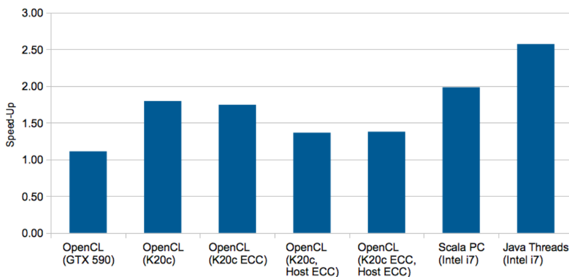
Figure 6.5: Speed-up obtained for the Gap Model depending on the underlying technique of parallelization
