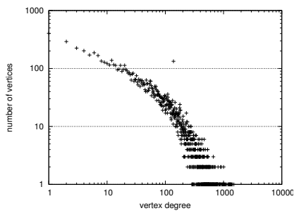
(a) Vertex degree distribution for \text{BioData}_{150}
