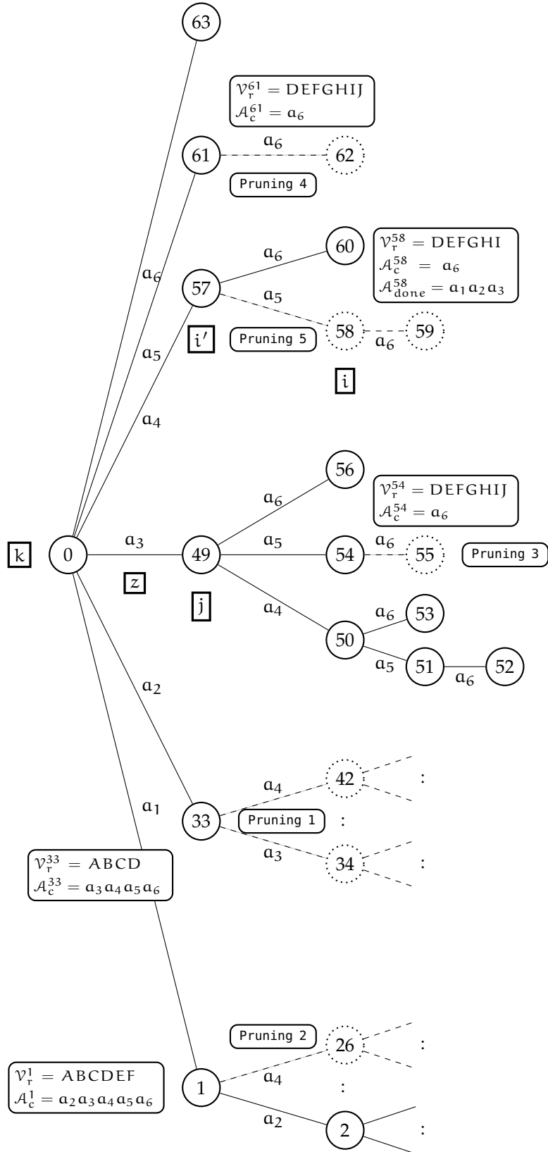
Figure 13.: Enumeration tree with pruning techniques 1, 2, 3, 4, and 5 corresponding to the attributed graph presented Figure 11 for constraints C_2^{homo} and C_{2,3}^{clique} .
