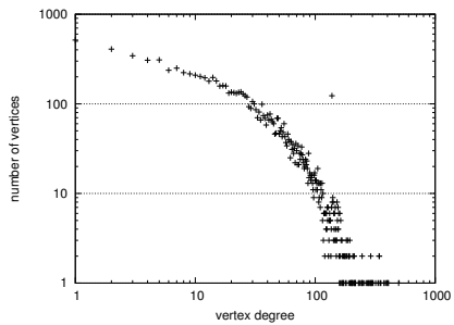
(c) Vertex degree distribution for \text{BioData}_{400}
