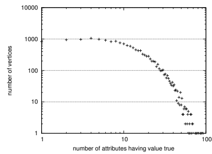
(b) Attributes distribution for \text{BioData}_{150}
