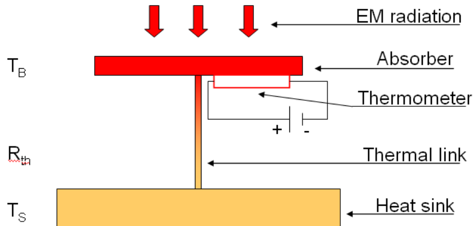
Fig. 2.1: Bolometer principle
