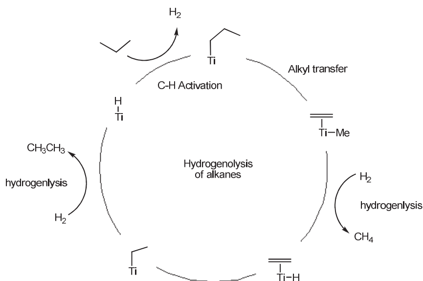
Scheme I.6: Proposed mechanism of alkane (propane) hydrogenolysis, Ti-H = [(\equiv\text{SiO})_{(4-x)}\text{TiH}_x]/ x= 1 or 2 .
