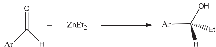
Scheme I.10: Ti(IV)-catalyzed \text{ZnEt}_2 addition to aromatic aldehydes.
