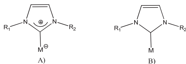
Scheme II.5: Different representations of metal-NHC bond.
