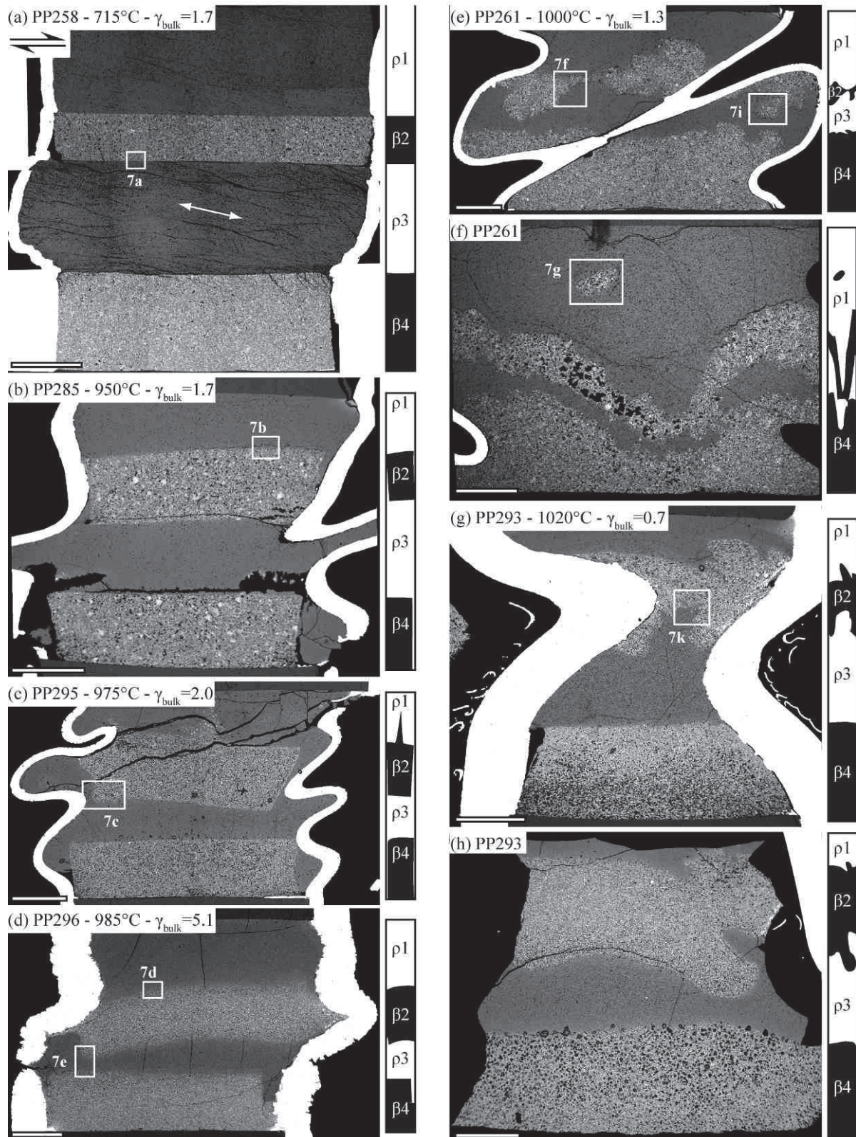
Figure VI* 5 : SEM pictures of large sections showing the relative position of layers after torsion experiments. The experiment conducted at 600°C and poorly deformed is similar to the 715°C one and not presented. The scale bar on the bottom left corner represents 1 mm. A sketch of the layer position is drawn on the right side. Black parts in (b) and (f) are holes unfortunately created during cutting and polishing preparation. The sense of shear presented in (a) is common for all sections. Note the bubble alignments created in PP258 (white couple of arrows).
