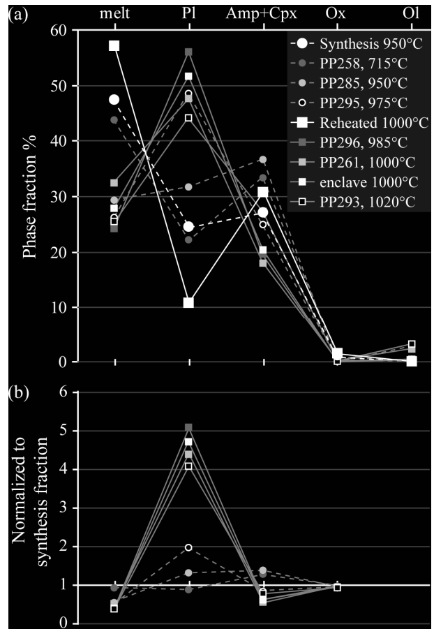
Figure VI* 6 : Phase fractions (a) and phase fractions normalized to the 950 and 1000°C starting suspensions ones (b) of the mafic layers in an area comprised between 0 and 150 \mu\text{m} from the contact with the felsic magma. The olivine fraction in (b) could not be calculated due to its absence in the starting suspension.
