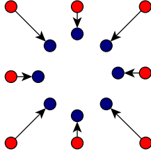
Figure 3.5: Illustration of the Earth-Mover-Distance. Here we see a set R of red points and a set B of blue points. The Earth-Mover-Distance EMD(R, B) is the weight of a minimum weight perfect matching between R and B . This matching is illustrated by the arrows and the value of EMD(R, B) corresponds to the sum of the lengths of these arrows.
