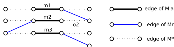
Figure 4.13: m_1, m_2, m_3 have each an edge of M_R incident and can be augmented with this edge and an incident edge from M^* . If m_2 is augmented with its incident edge from M_R and o_2 , then this may prevent m_1 and m_3 from being augmented.
