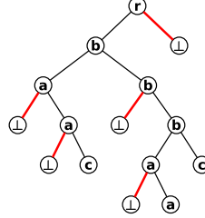
Figure 6.3: \text{FCNS}^\perp encoding of the example tree already shown in Figure 6.1. \text{XML}^{\text{F}\perp}(t) = rba\perp\perp a\perp\perp c\bar{c}a\bar{a}b\perp\perp ba\perp\perp a\bar{a}c\bar{c}bb\perp\perp \bar{r} .
