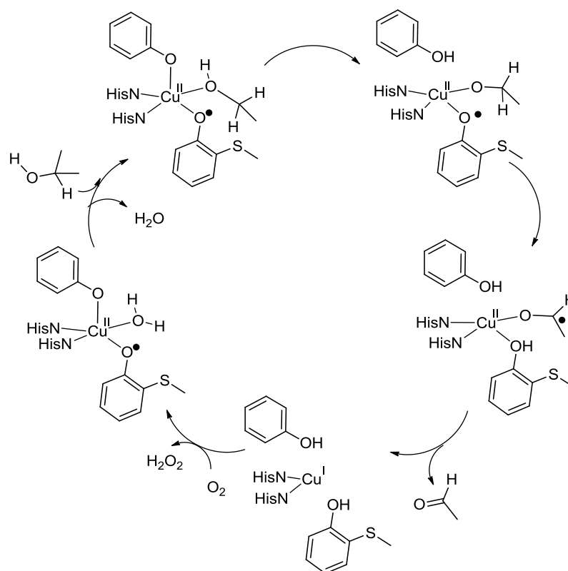
Figure 5: Cycle catalytique de la GO.
