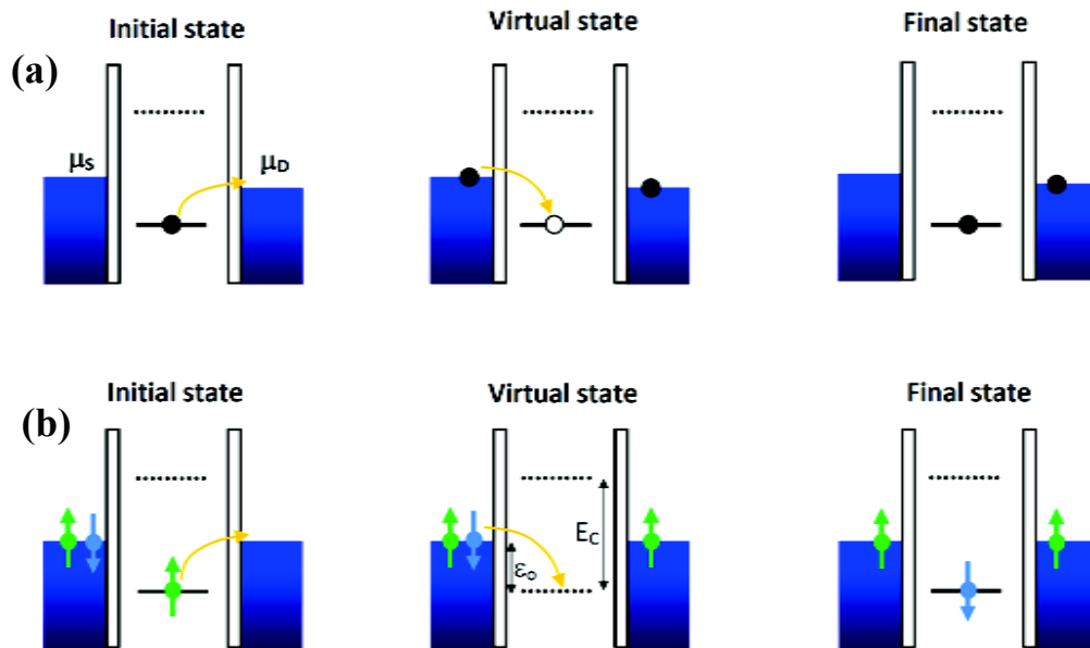
Figure 5.11. Higher-order tunneling events that overcome Coulomb blockade. (a) Elastic cotunneling in general. There are N electrons on the dot. The N^{\text{th}} electron jumping from the dot to the drain will be immediately replaced by an electron from the source. At a small bias voltage, such processes lead to the flow of a current through the dot. (b) Elastic cotunneling with spin flip. The spin-up electron jumping out of the dot is immediately replaced by a spin-down electron. Many such higher-order spin flip events together build up a spin singlet state consisting of electron spins in the reservoirs and the spin on the dot. The spin on the dot is thus screened [8].
