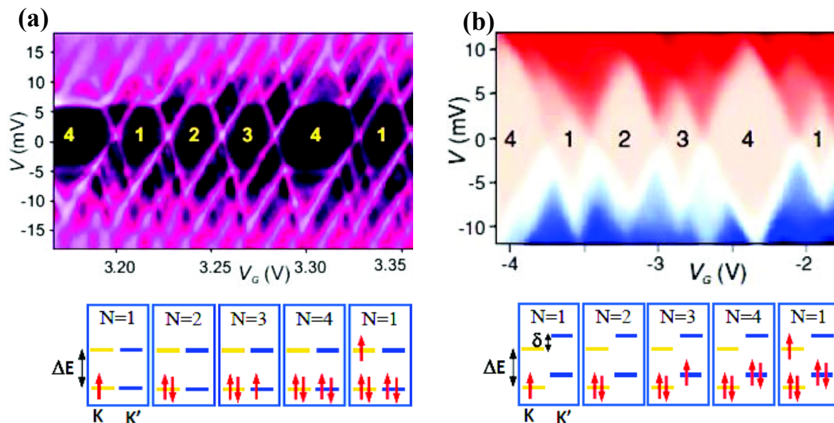
Figure 5.7. Measurements of addition energy of (metallic) CNT QDs. (a) Perfect four-fold level degeneracy, from ref. [10]. The addition energies follow the sequence [ E_c , E_c , E_c , E_c + \Delta E ] (see inset). (b) An orbital energy mismatch leads to an increase of the addition energy for N=2 , from ref. [11] and the sequence is now [ E_c , E_c + \delta , E_c , E_c + \Delta E ].
