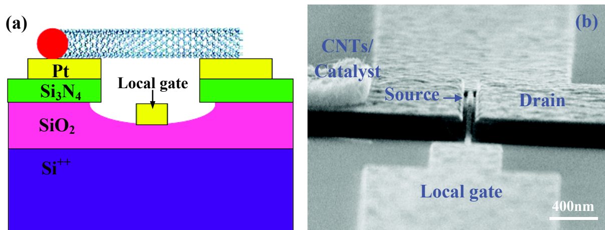
Figure 4.5. Fabrication of a local gate device. (a) Schematic and (b) SEM image of a final device. The arrow is at the position of the suspended CNT.
