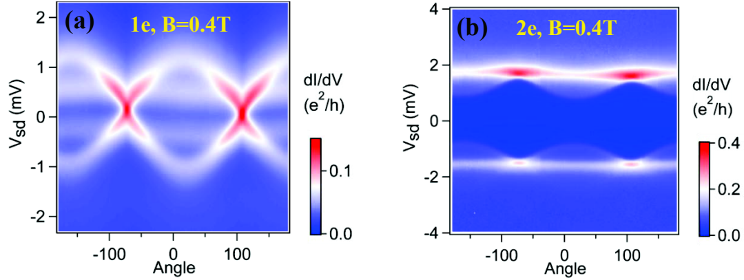
Figure A2.2. Evolution of the differential conductance as a function of B applied angle and V_{SD} . The B applied is fixed at 0.4T and V_{LG} is fixed in middle of (a) 1 st and (b) 2 nd diamond, respectively.
