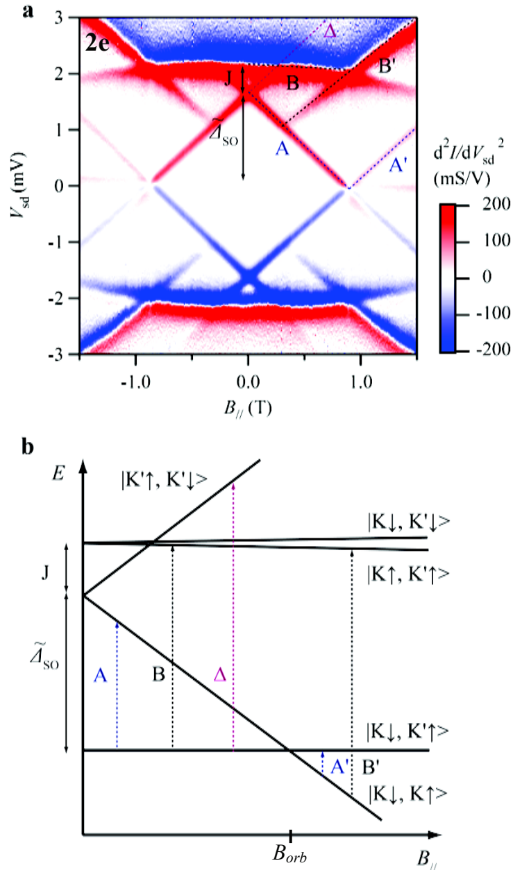
Figure 6.7. (a) Second derivative d^2I/dV_{SD} along the center of the N = 2e diamond (orange dotted line in Fig. 6.3) as a function of V_{sd} and B_{//} . (b) Expected energy level scheme of the N = 2e ground state. The excited states at energy 2\Delta are not shown here.
