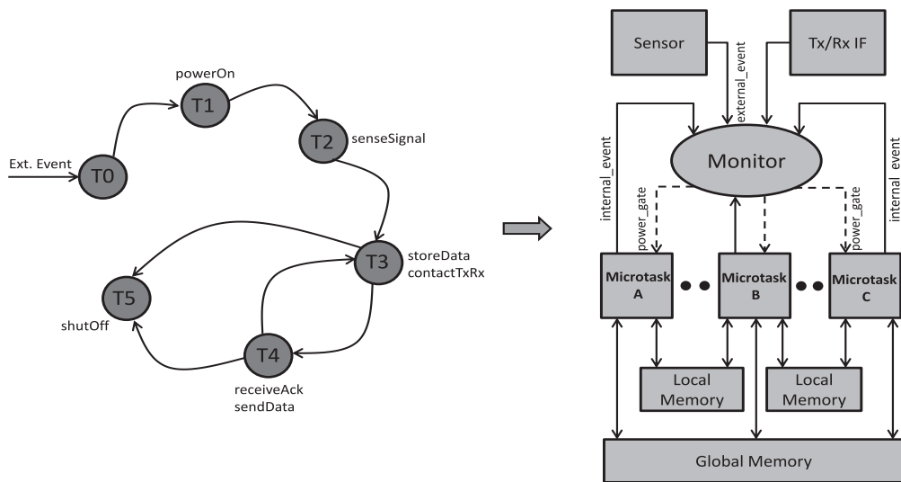
FIGURE 1.2: A generalized task flow graph and system level view of generated architecture as proposed in [1].
