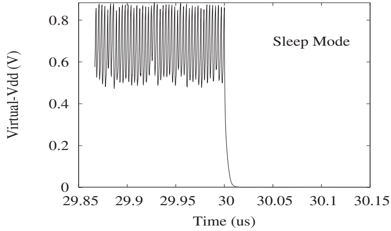
FIGURE 3.5: Active mode and sleep mode Virtual-Vdd in power-gated c6288 ( W=12\mu\text{m} ).
