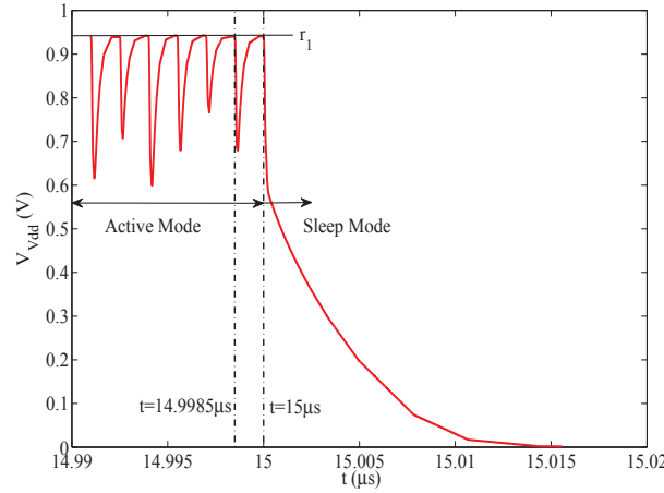
FIGURE 3.10: Virtual-Vdd in active and sleep modes.
